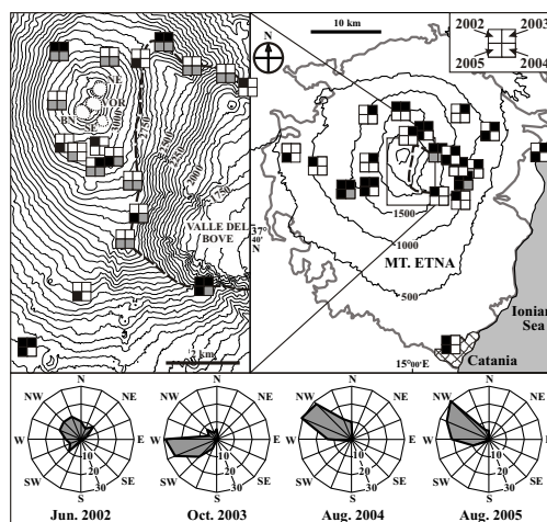
Fig. 1. Location of the sites where diffusive tubes were exposed on Etna during the different measurement campaigns. The bold grey line limits the outcrop area of Etean volcanic products, while the dashed line shows the rim of the Valle del Bove. The summit craters are indicated with different initials: NE – North-East Crater; SE – South-East Crater; BN – Bocca Nuova; VOR – Voragine. Diffusive tubes were exposed for about one month in four campaigns on May–June 2002, October–November 2003, July–August 2004 and July–August 2005. For each sampling site, the symbol is subdivided into four sectors, each referring to a different survey. A white sector indicates no sampling; a black sector indicates sampling of SO 2 and halogens; a grey sector sampling of SO 2 , halogens and H 2 S. The wind rose diagrams showing the frequency of wind provenance (directions from which the wind originated are marked) at 700 hPa during the four surveys are also shown – as based on Trapani Birgi atmospheric sounding data ( http://www.weather.uwyo.edu/upperair/sounding.html ).
