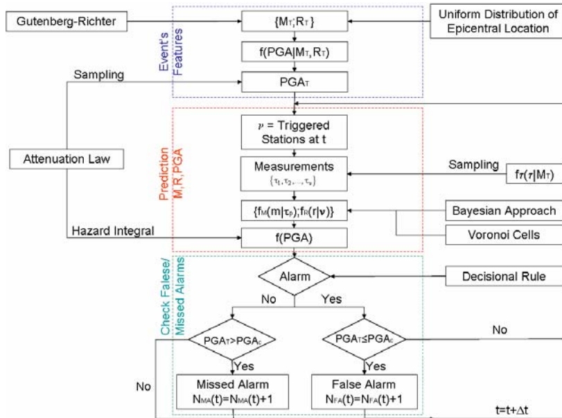
Figure 3: Simulation's flow chart
