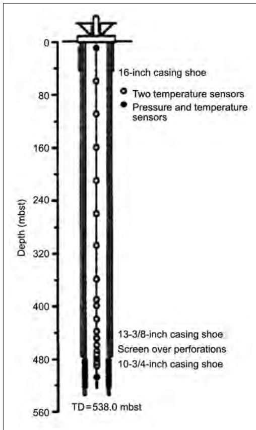
Fig. 5. Configuration of the sensor string under the CORK in the Hole 948D.
