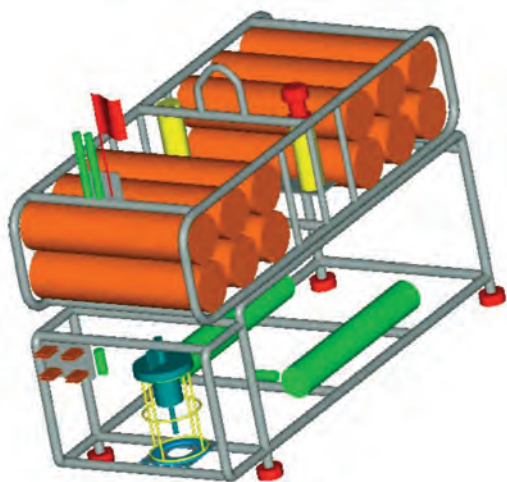
Fig. 2. The OT6000 thermal observatory is deployed and recovered as a lander (syntactic foam, acoustic release). The temperature needles are positioned by arms of the Nautile.
