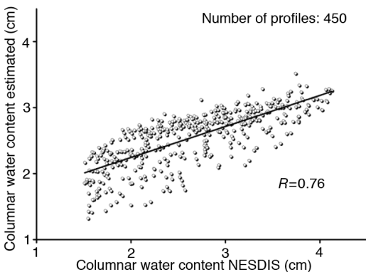
Fig. 2. Correlation index between the columnar content estimated and NESDIS.
