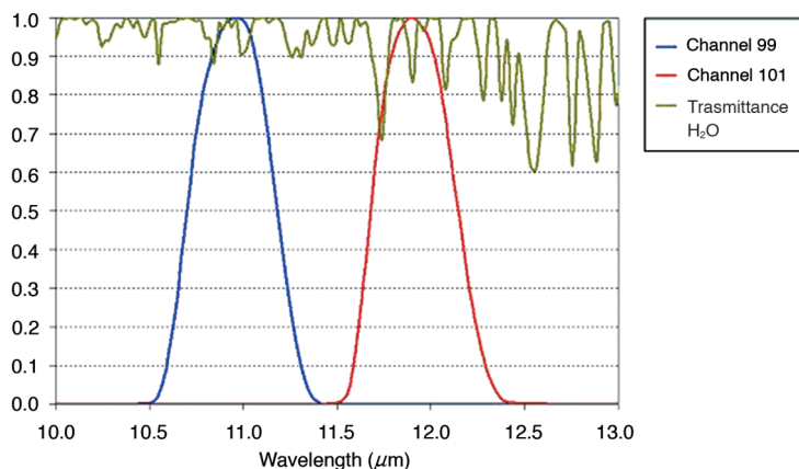
Fig. 1. MIVIS channel 99 (blue) and 101 (red) response functions versus transmittance (green).
