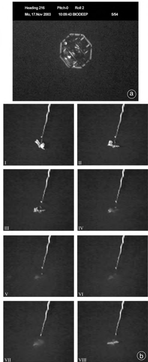
Fig. 6a,b. Images of the interface as seen by MODUS: a) view from MODUS to the suspended SCIPACK (10 m mechanical cable) right before entering the Urania Basin; b) sequence of the survey at the interface of L'Atalante (10 m cable): iron ball and flag approaching the interface (I-III), entering the brines (IV), laying below the interface (V-VII) and coming out (VIII).
