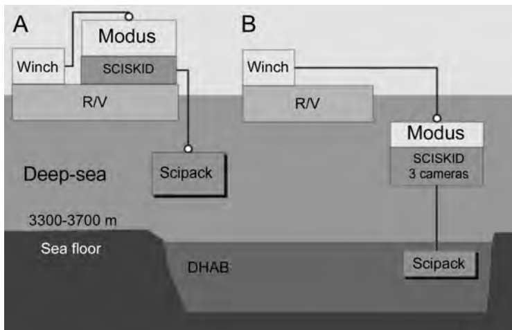
Fig. 4. Operational concept of BIODEEP mission for sampling and surveying: A – deployment of SCIPACK from the ship; B – operation of the MODUS-SCIPACK system at the interface of the DHAB.
