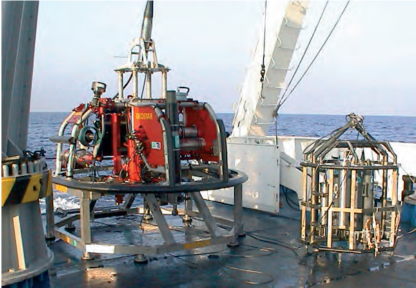
Fig. 3. MODUS with SCISKID (left) and SCIPACK (right) onboard R/V Urania.
