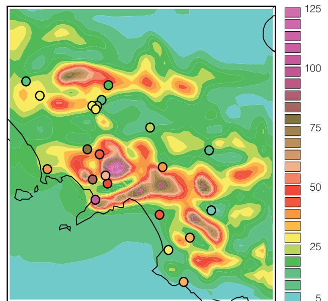
Fig. 6. 24 h accumulated precipitation (mm) ending at 0000UTC 5th May both predicted on domain 3 using three domains two way nested and observed at a few stations (colored circles). The circles are filled with the color corresponding to the scale shown on the right.
