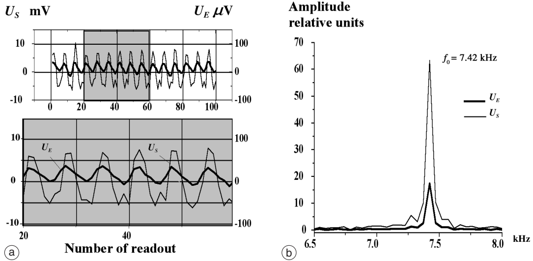
Fig. 6a,b. MSO of the first type ( E = 9 v/cm): a) electric ( U_E ) and acoustic ( U_S ) signals; b) spectra of the signals U_E and U_S .
