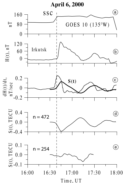
Fig. 3a-e. The variations in magnetic flux (a) at geostationary orbit of the GOES10 station ( 135^\circ\text{W} ), the variations of the H -component of the magnetic field H(t) (b), and of the time derivative dH(t)/dt (c) (thin line) for the time interval 16:00-18:00 UT, April 6, 2000, at station Irkutsk ( 52.2^\circ\text{N} , 104.3^\circ\text{E} ). The result of a global spatial averaging of S(t) (d) for 472 LOS on the dayside. A similar result for 245 LOS on the nightside (e). For comparison, panel (c) presents the inverted curve S(t) (heavy line) on the dayside. The time of SSC is shown on panels (a-e) by a vertical dashed line.
