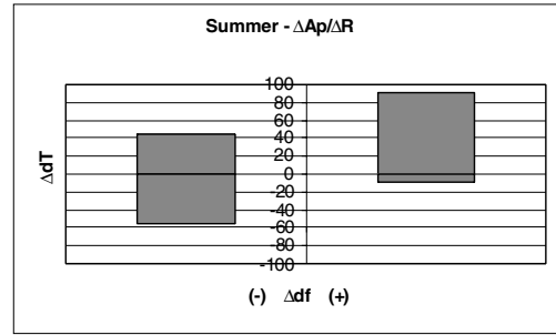
Fig. 4b. \Delta df versus \Delta dT behaviour in summertime and when \Delta A_p/\Delta R is positive.
