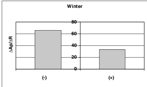
Fig. 3a. \Delta A_p/\Delta R behaviour in winter.
