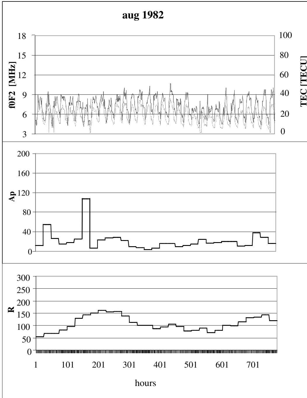
Fig. 1a. Characteristic month showing the f_oF_2 (solid line) and the TEC (dashed line), A_p and R values.
