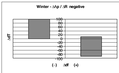
Fig. 4a. \Delta df versus \Delta dT behaviour in wintertime and when \Delta A_p/\Delta R is negative.
