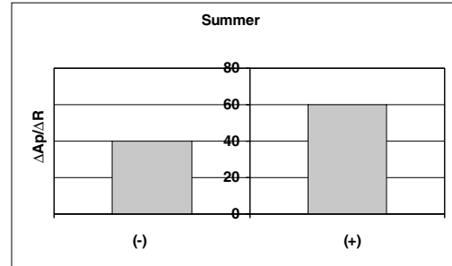
Fig. 3b. \Delta A_p/\Delta R behaviour in summer.
