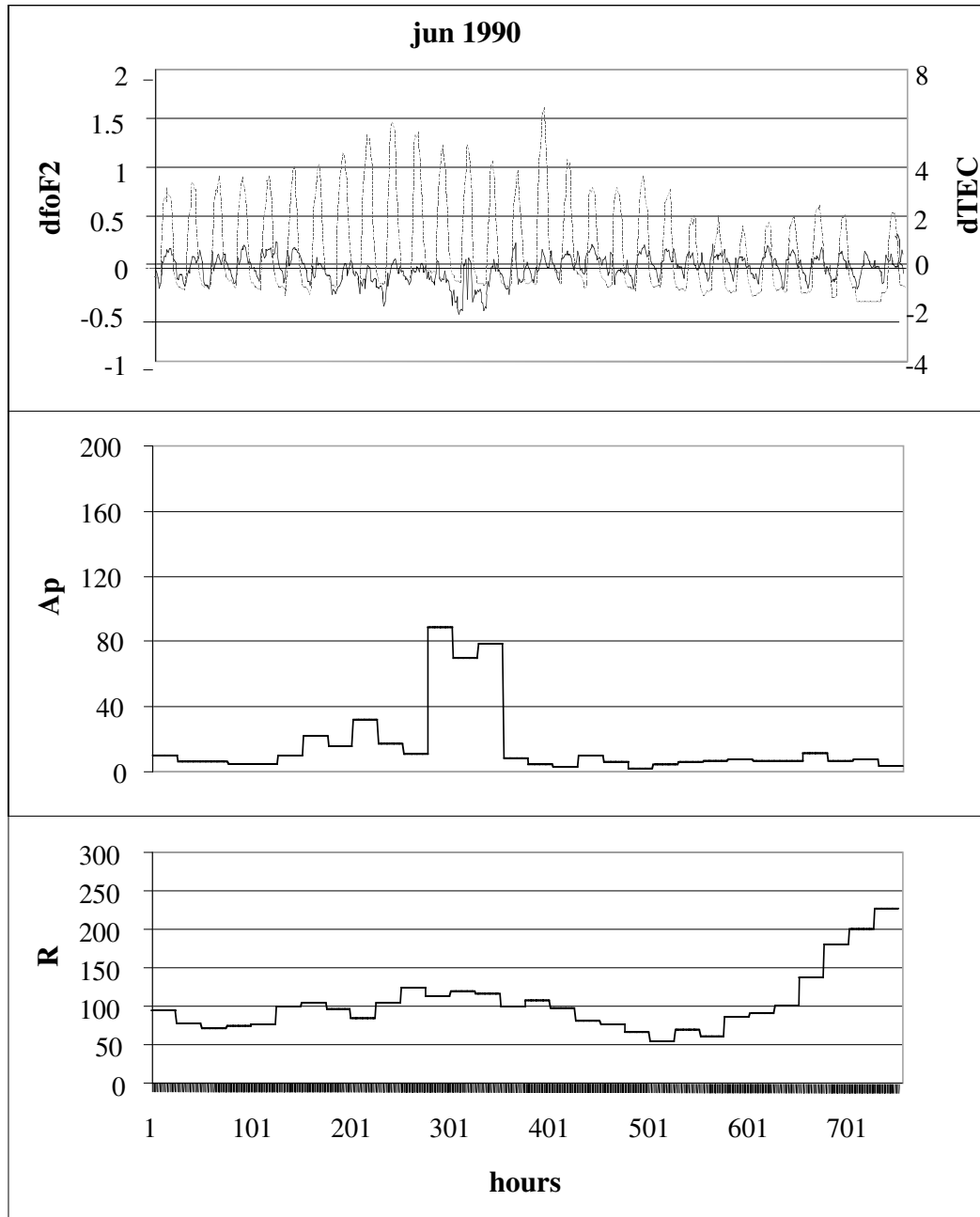
Fig. 2d. Presentation of df_oF_2 , dTEC , A_p and R .
