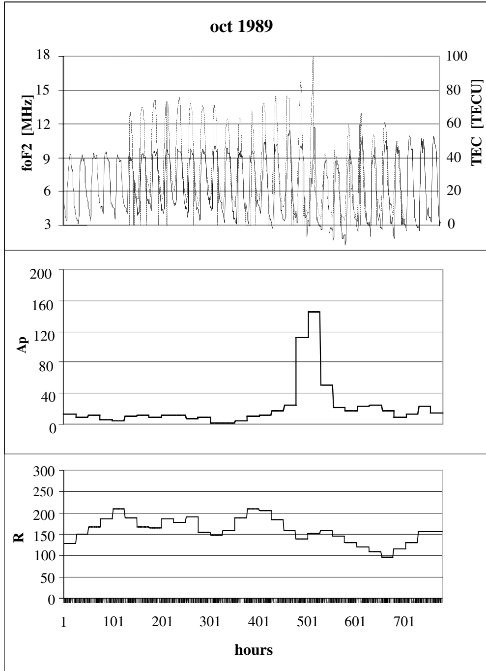
Fig. 1b. Characteristic month showing the f_oF_2 (solid line) and the TEC (dashed line), A_p and R values.
