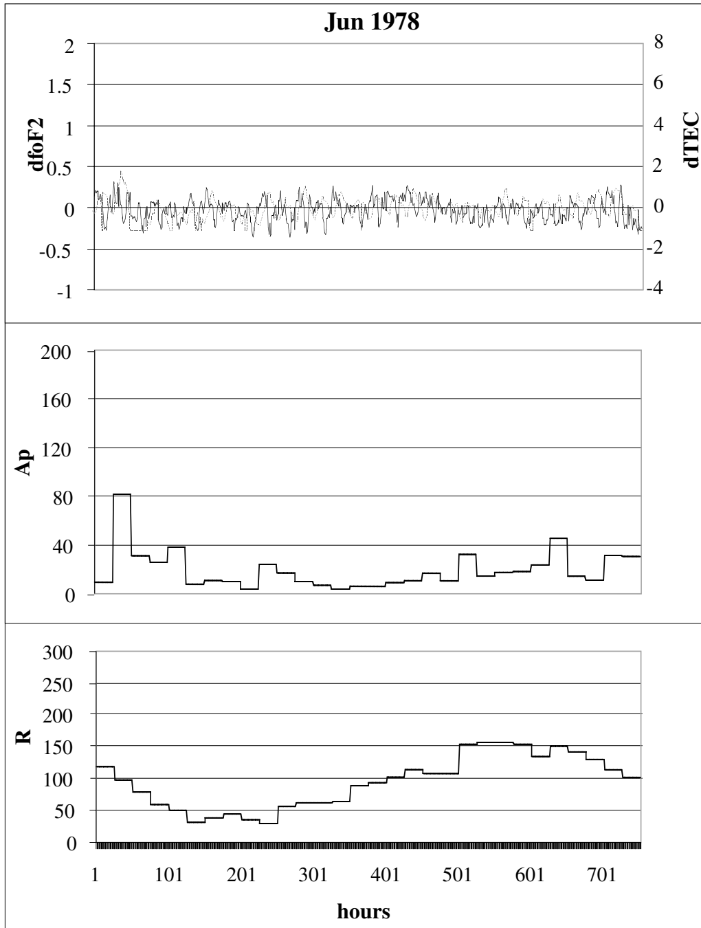
Fig. 2b. Presentation of dfoF_2 , dTEC , A_p and R .
