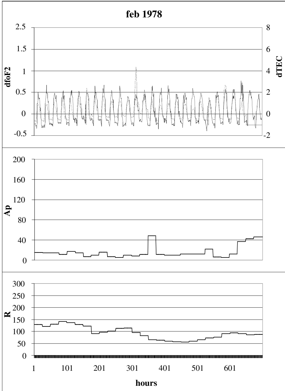
Fig. 2a. Presentation of df_0F_2 (solid line), dTEC (dashed line), A_p and R .
