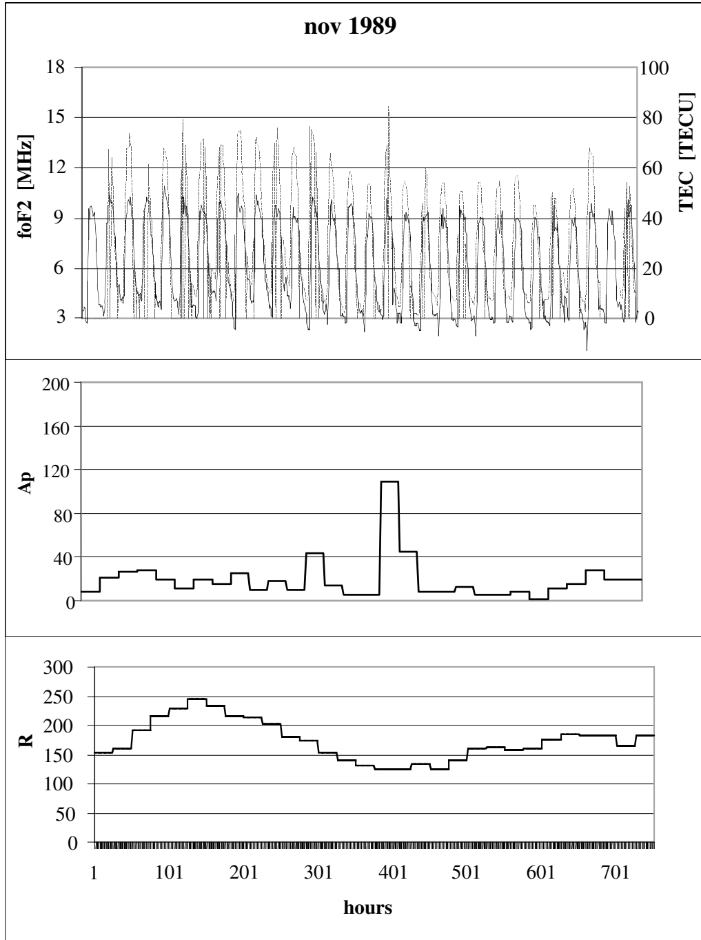
Fig. 1c. Characteristic month showing the f_oF_2 (solid line) and the TEC (dashed line), A_p and R values.
