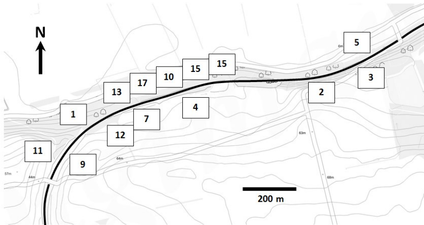
Figure 3: Earthworks Prioritization based on Network Rail weightings
