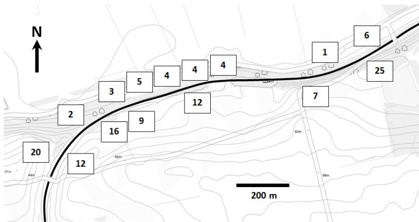
Figure 4: Earthworks prioritization based on Heritage Railway weightings
