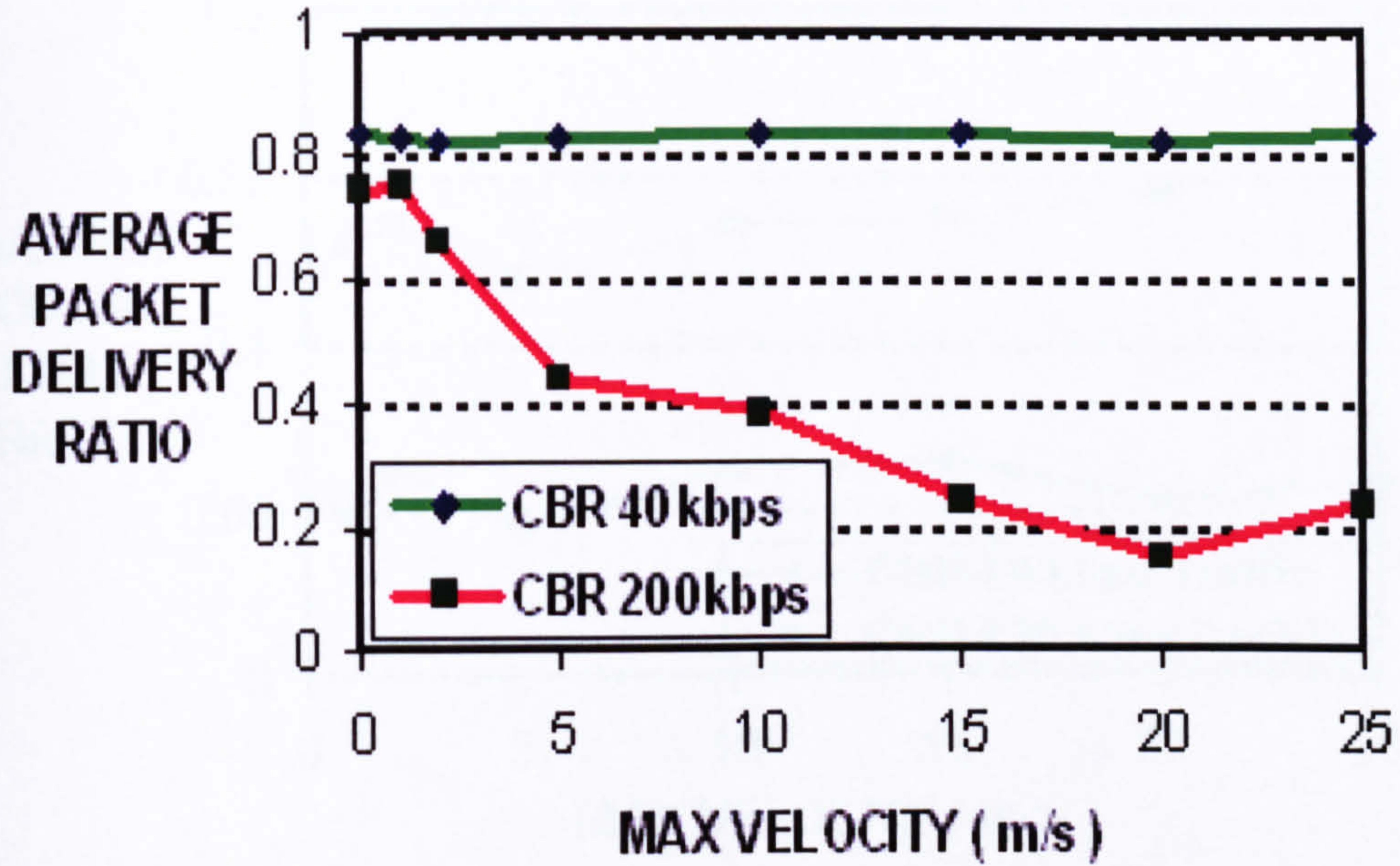
Figure 6-17 Average Packet Delivery Ratio as a Function of Max Velocity
