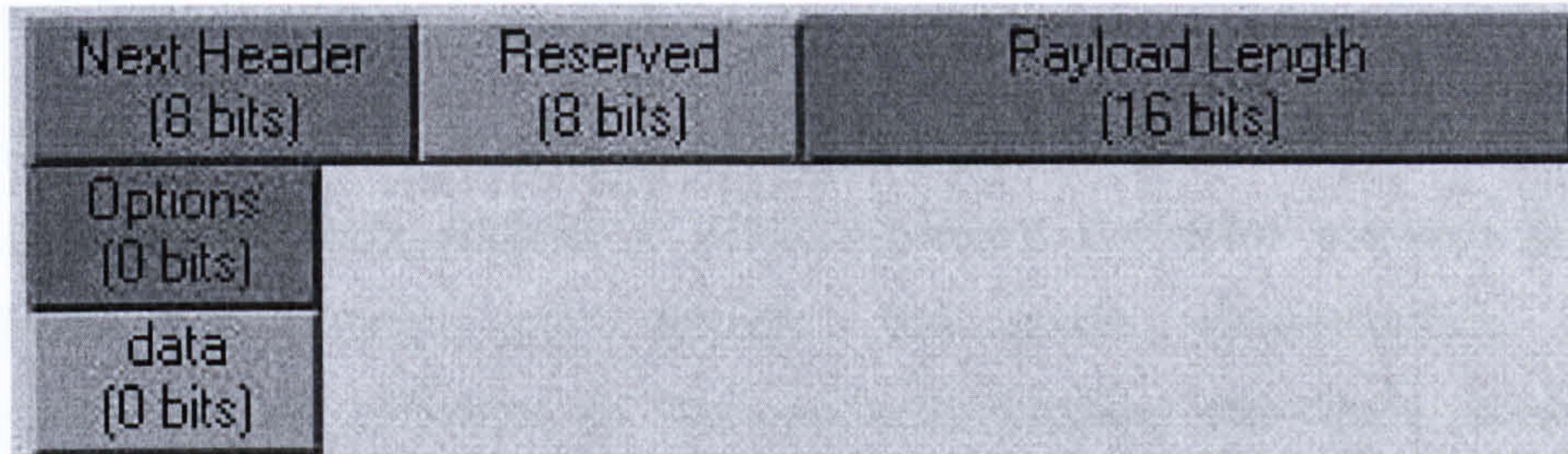
Figure 3-8 Fixed Portion of QOSRGA Packet
