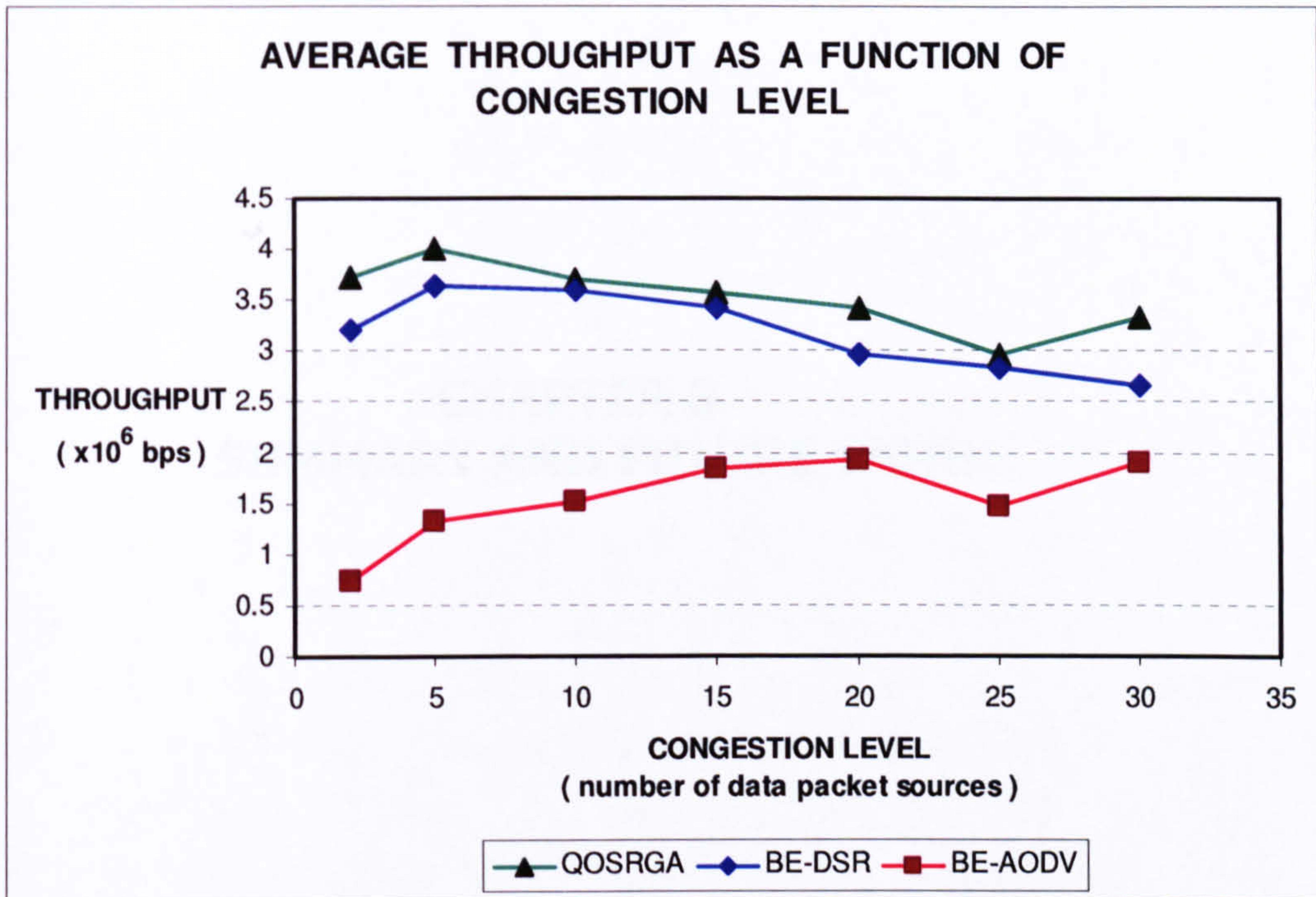
Figure 7.14 Average Total Throughput against the Congestion Level
