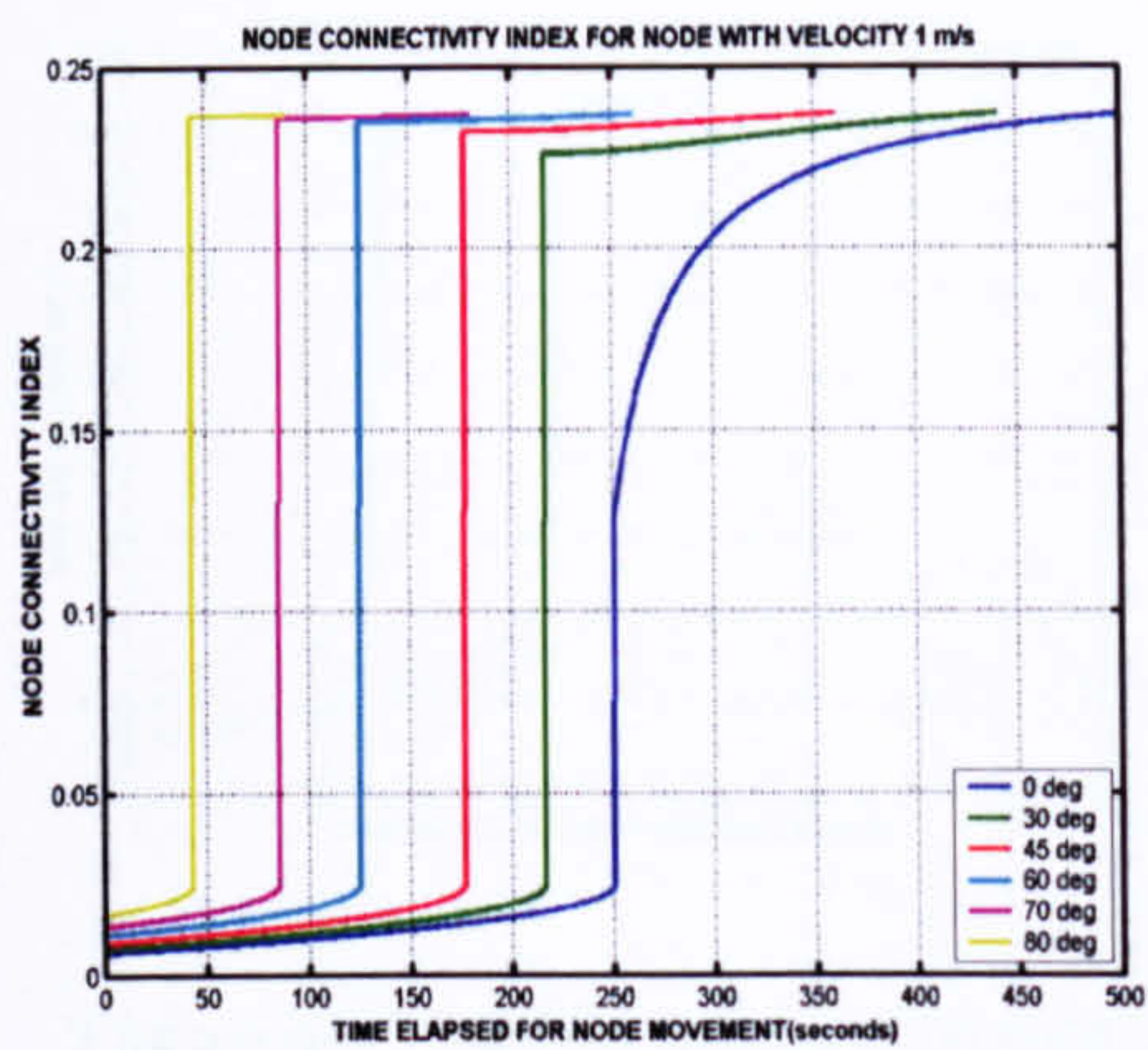
Figure 4-9 nci for velocity 1 m/s
