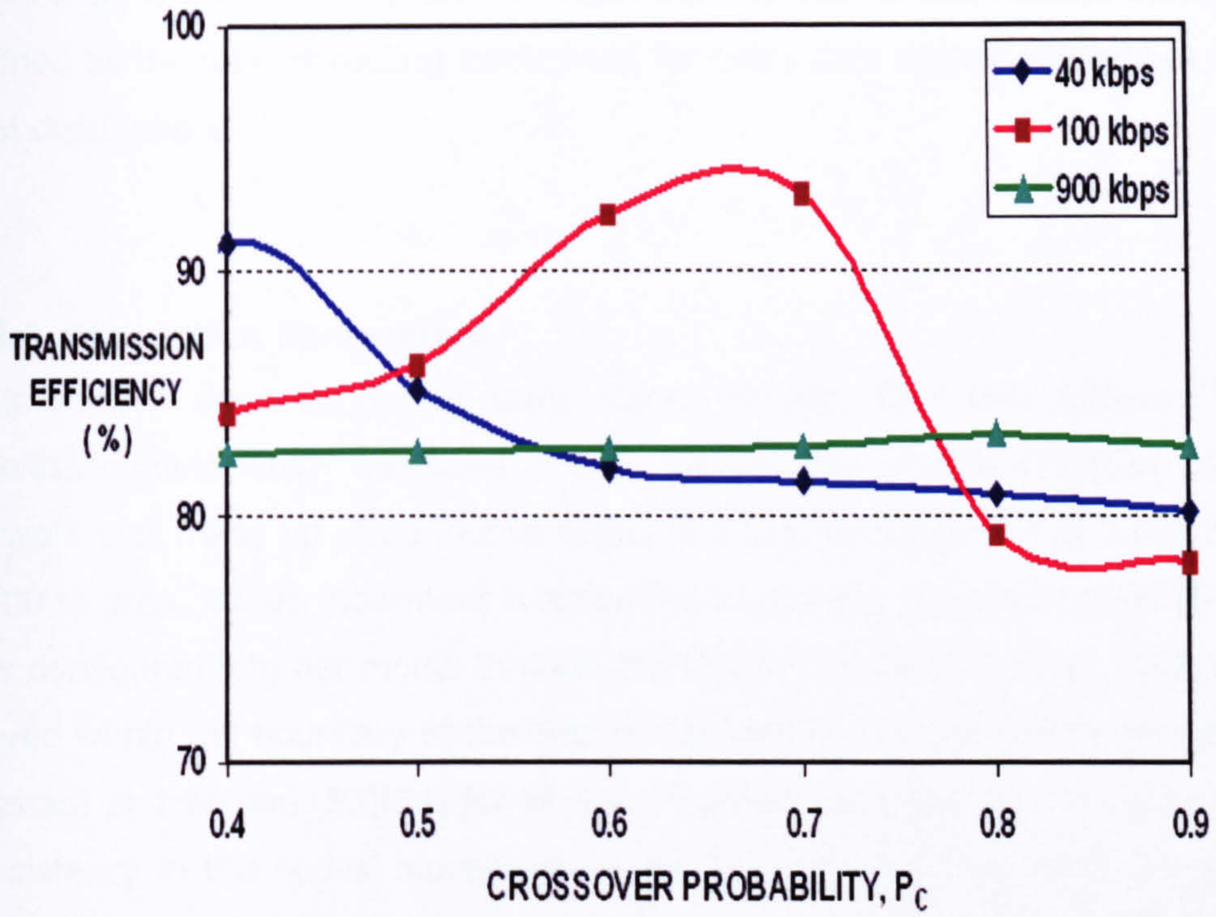
Figure 6-9 Transmission Efficiency as a Function of Crossover Probability
