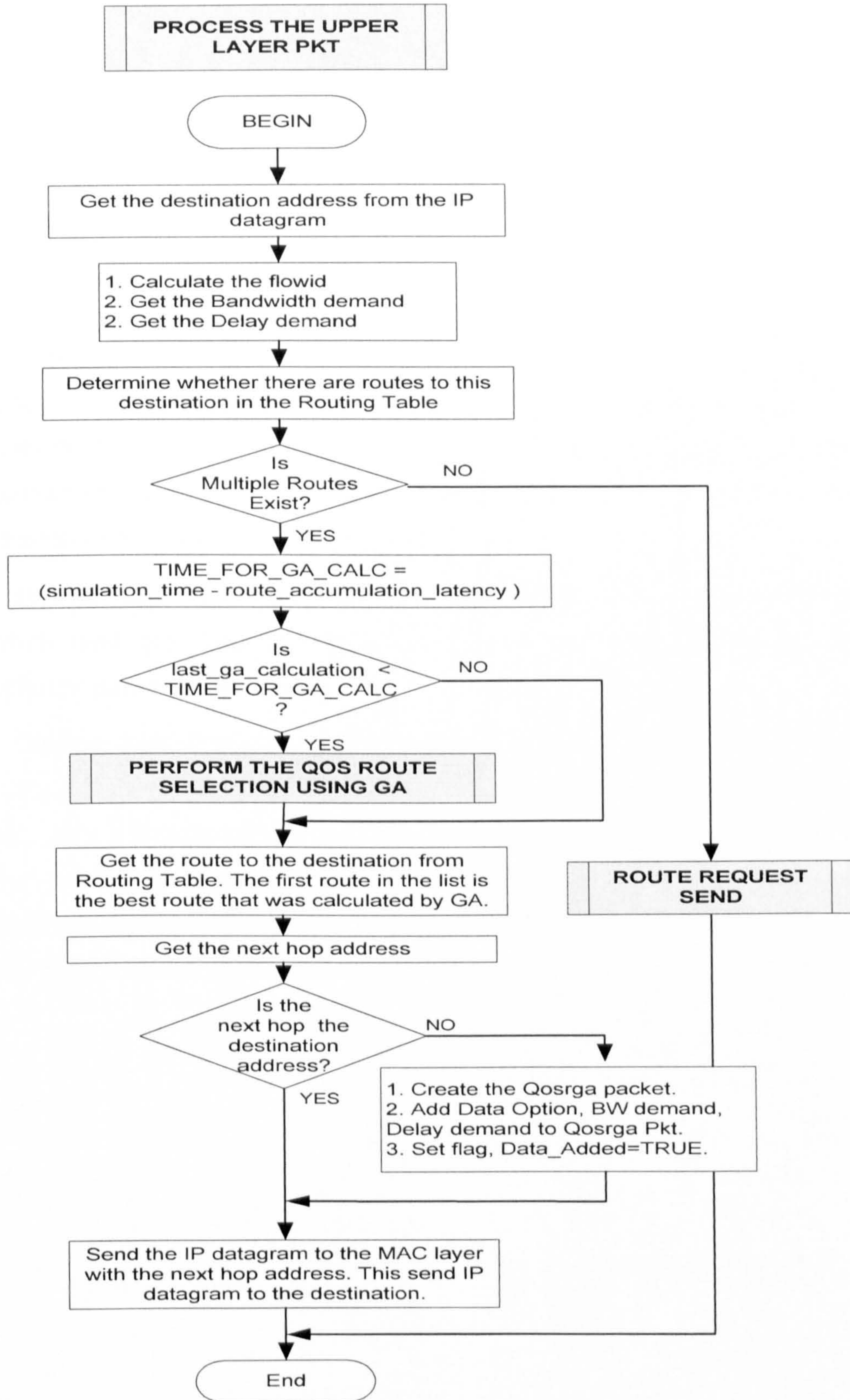
Figure 3-10 Process the upper layer packet
