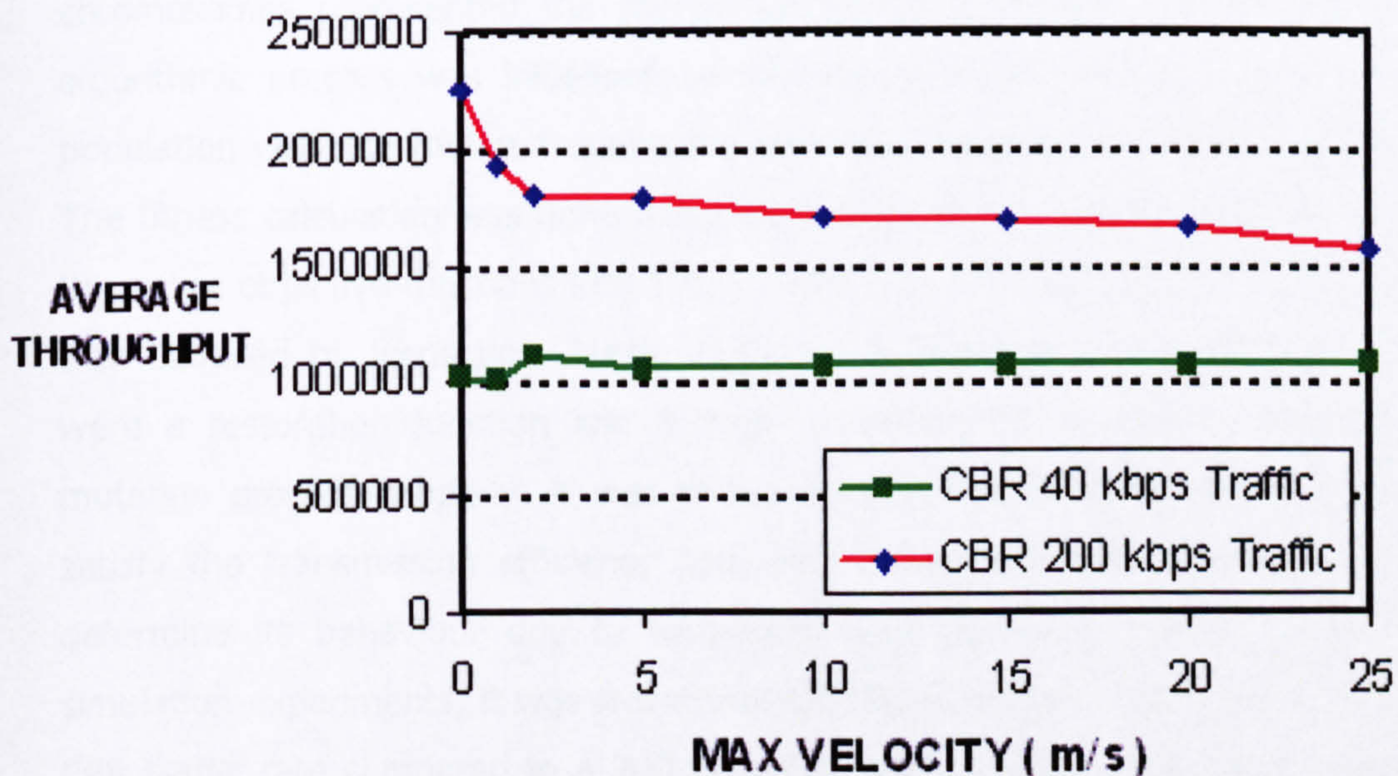
Figure 6-20 Average Throughput as a Function of Max Velocity
