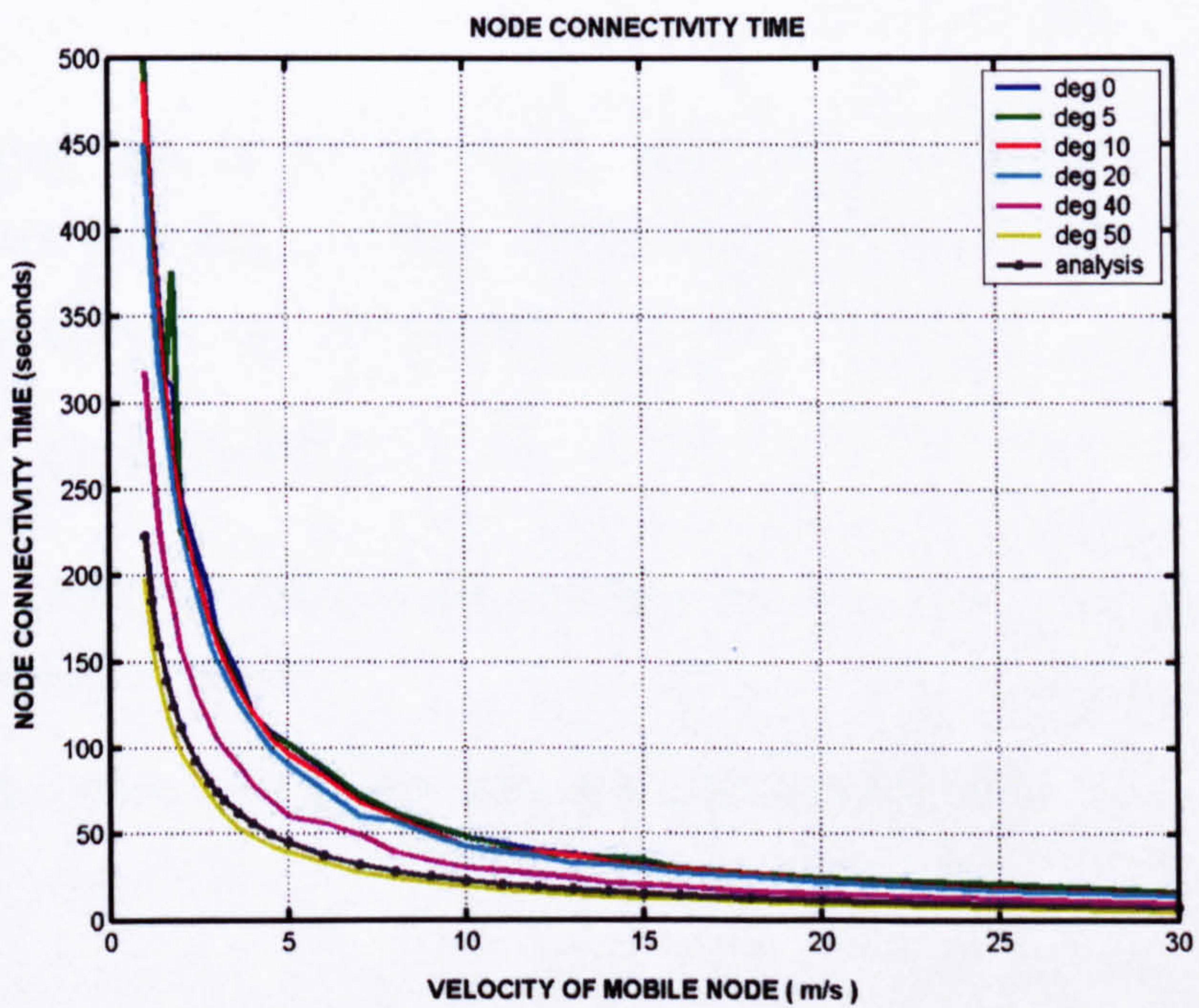
Figure 4-6 Node Connectivity Time against Velocity
