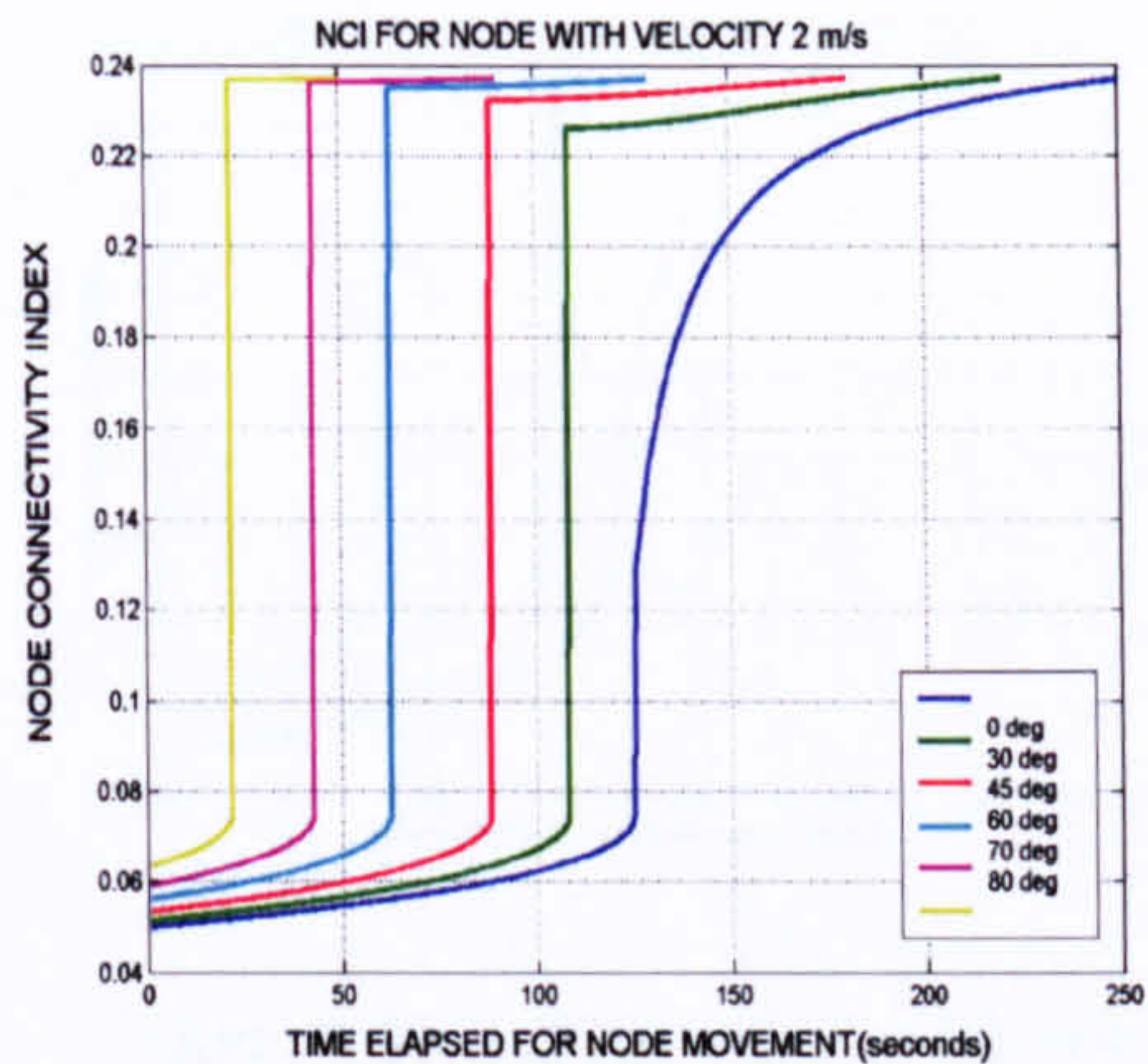
Figure 4-10 nci for velocity 2 m/s
