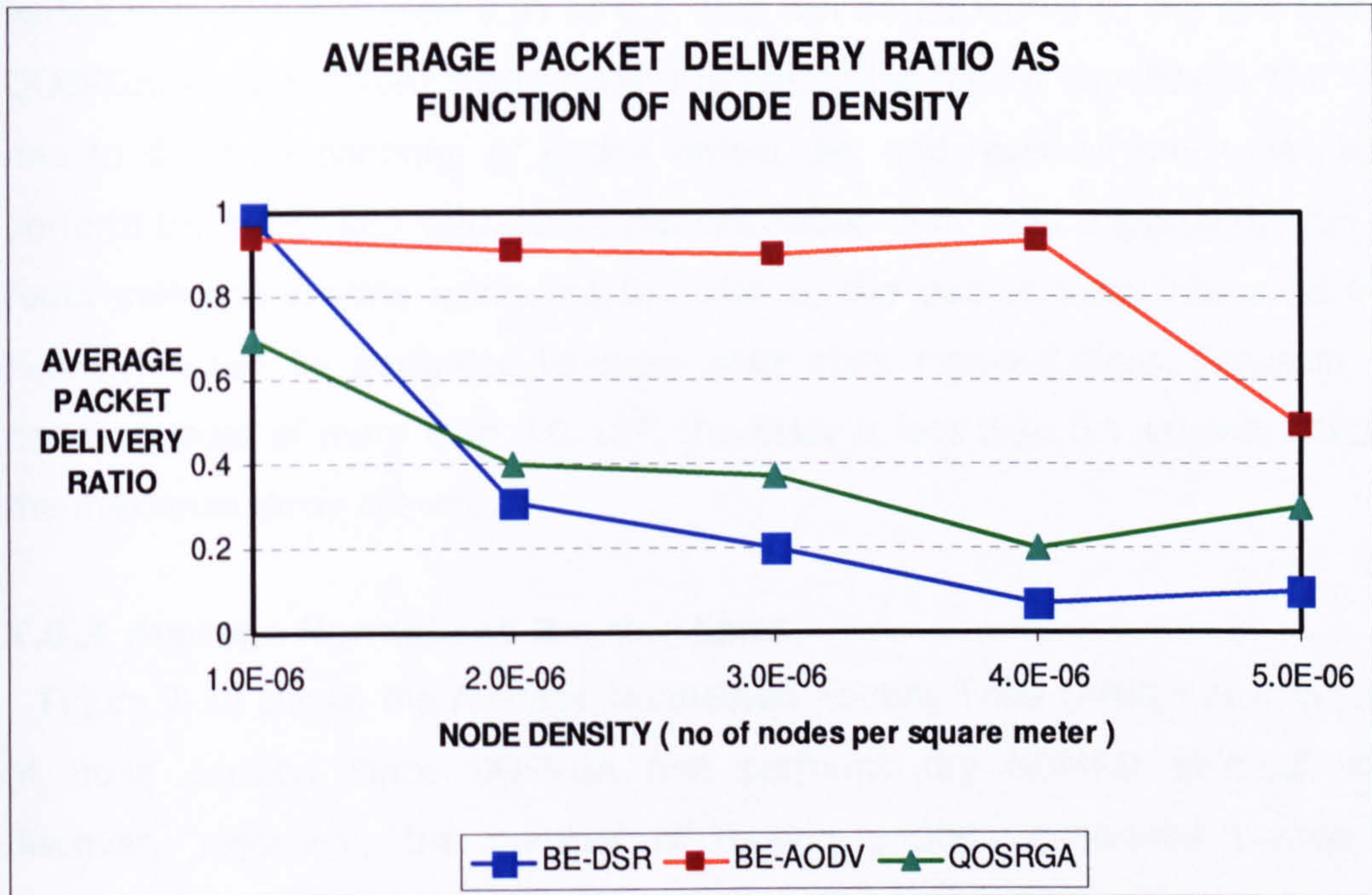
Figure 7-8 Average Packet Delivery Ratio against Node Density
