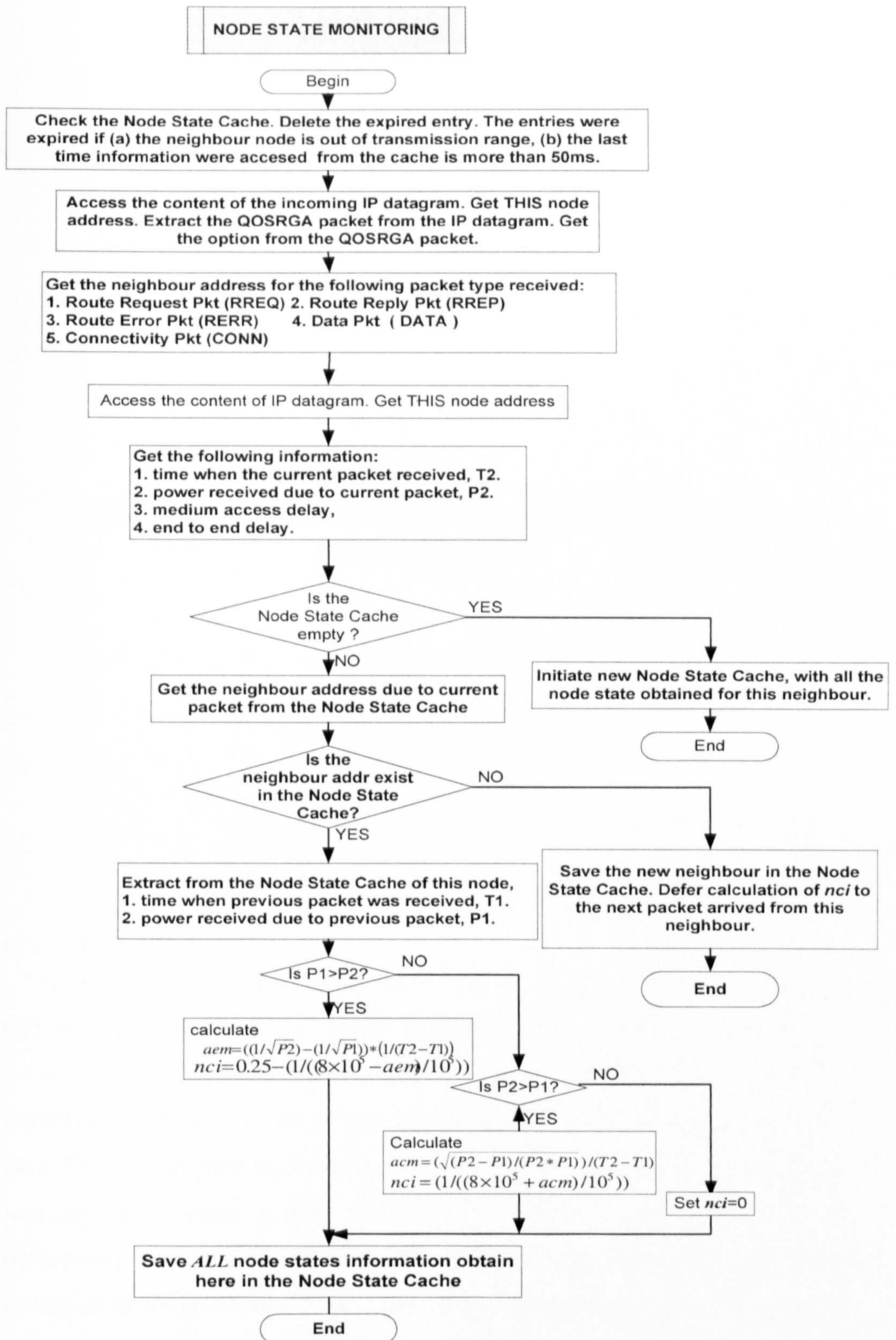
Figure 5-18 Flowchart of Node State Monitoring
