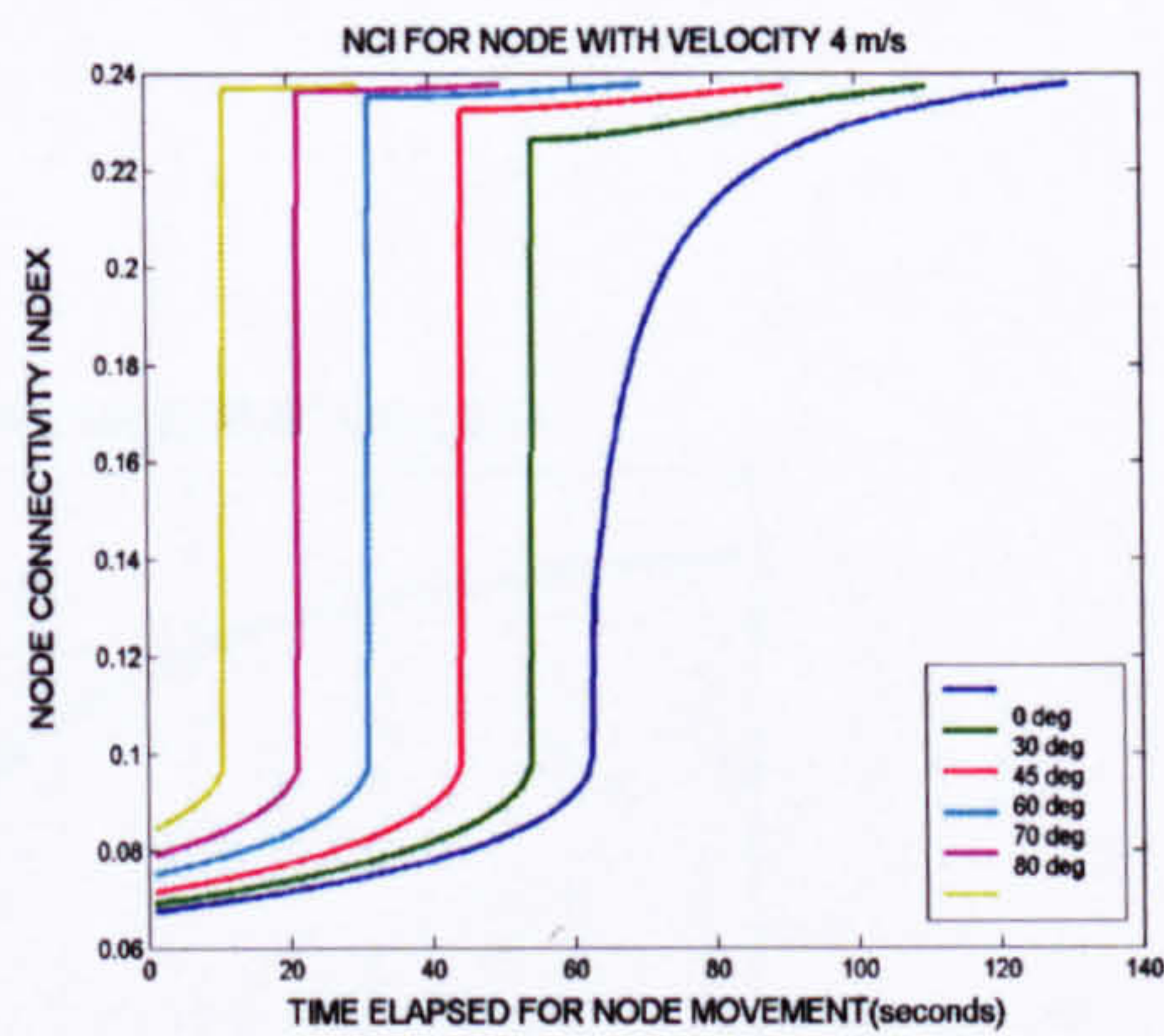
Figure 4-12 nci for velocity 4 m/s
