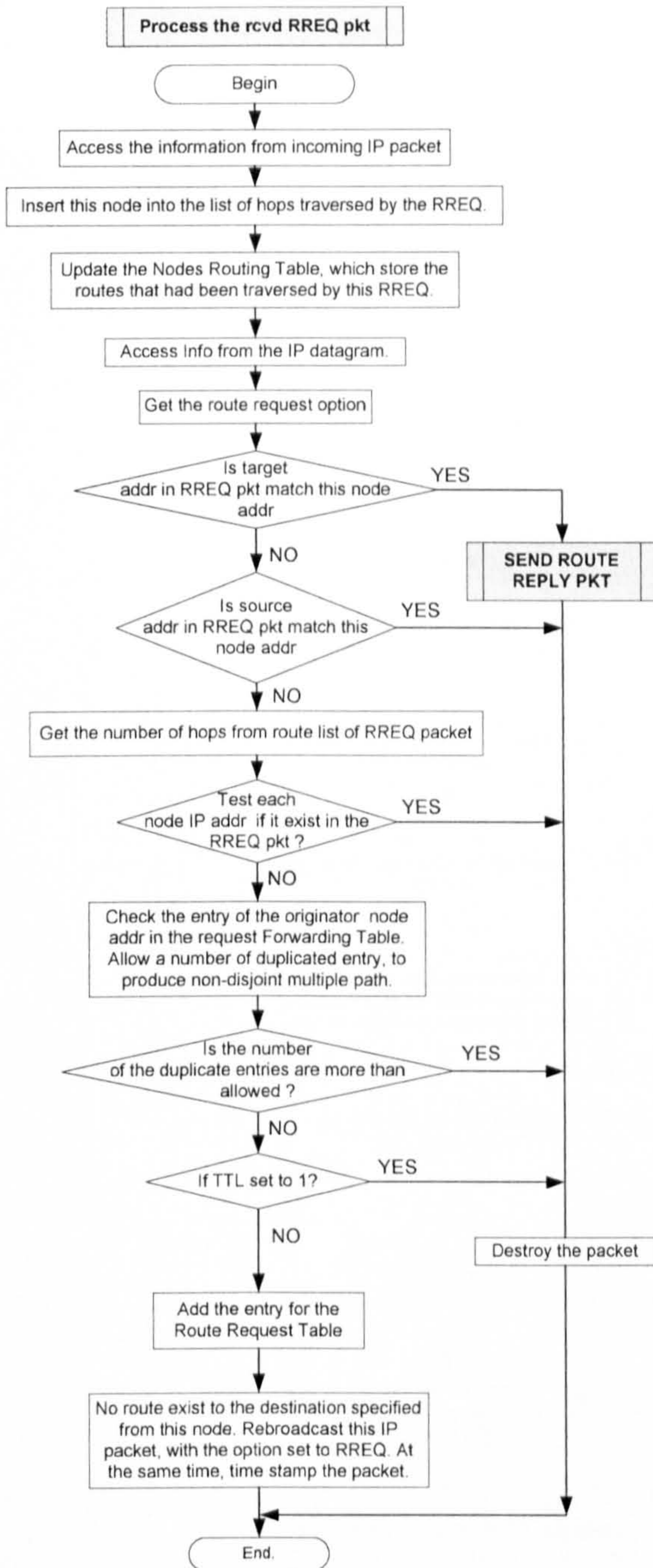
Figure 3-17 Received Route Request
