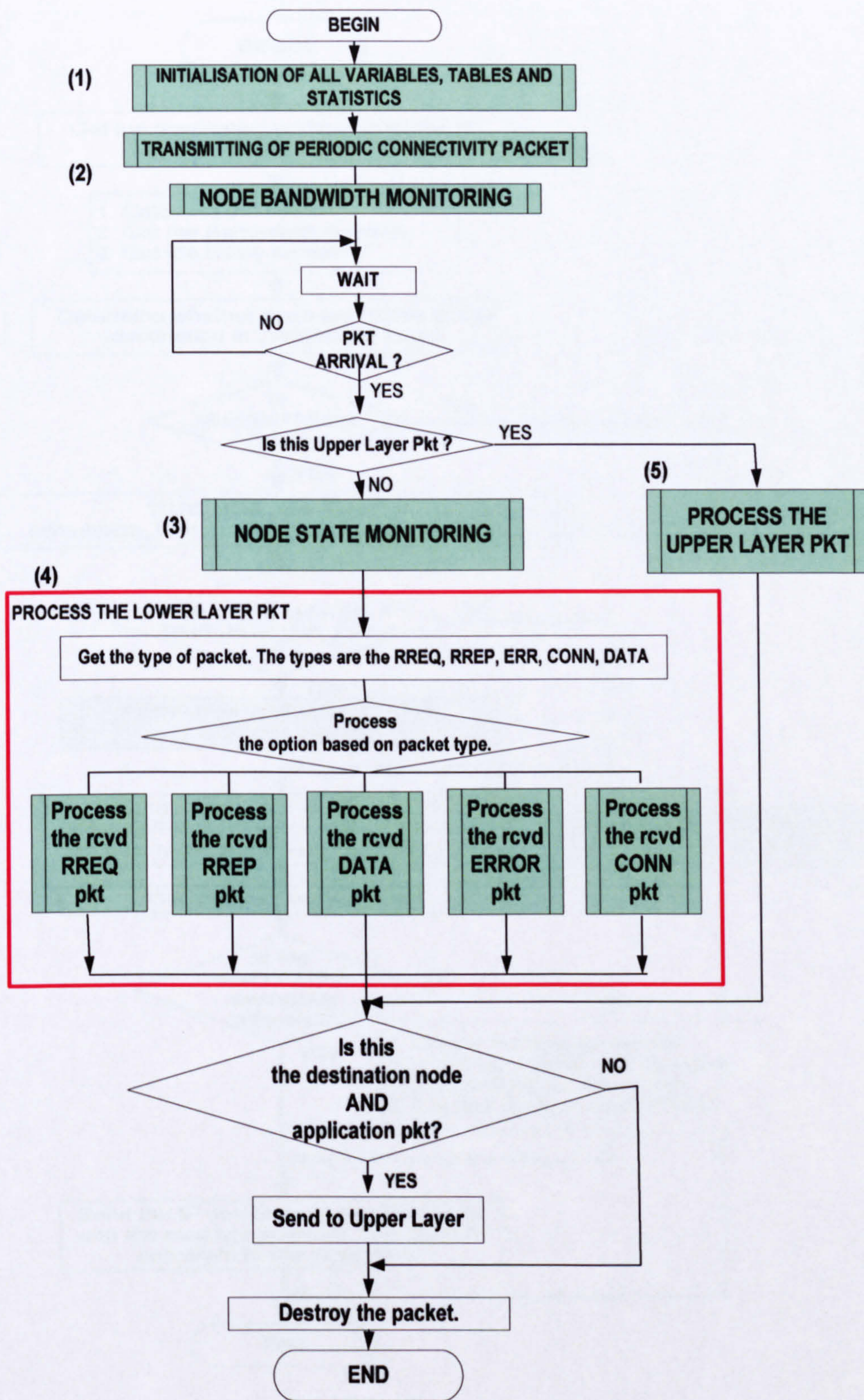
Figure 3-9 Overall Flowchart of QOSRGA
