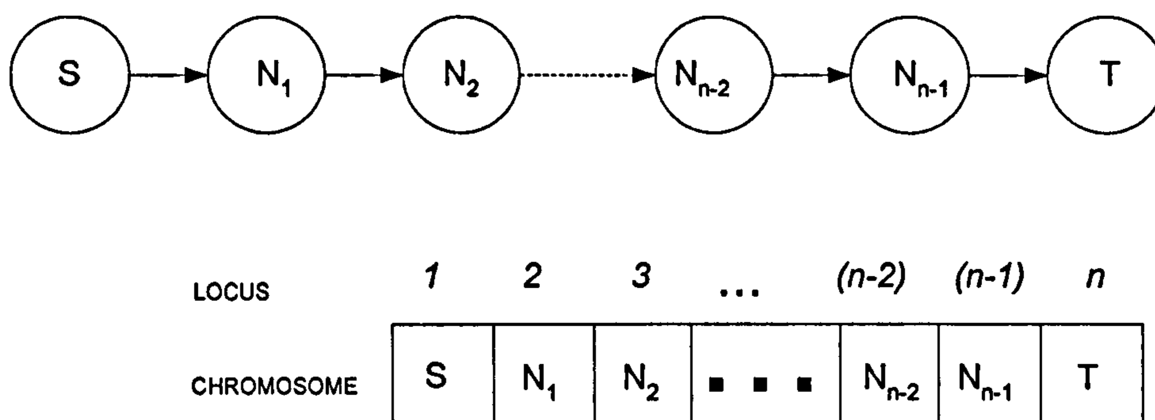
Figure 6-2 Chromosome Representation of S-T Route
