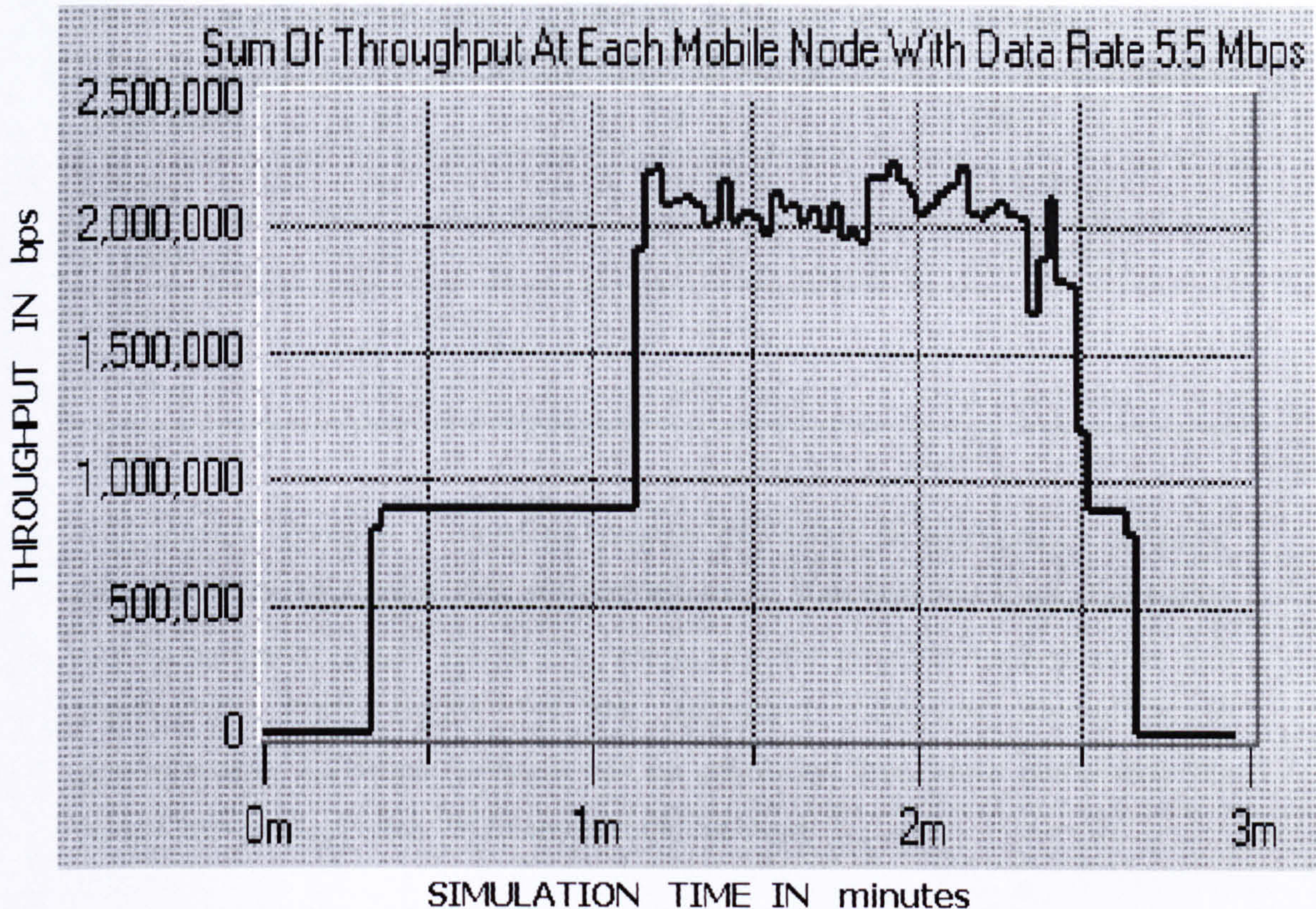
Figure 5-3 Sum Of Throughput from Each Mobile Node
