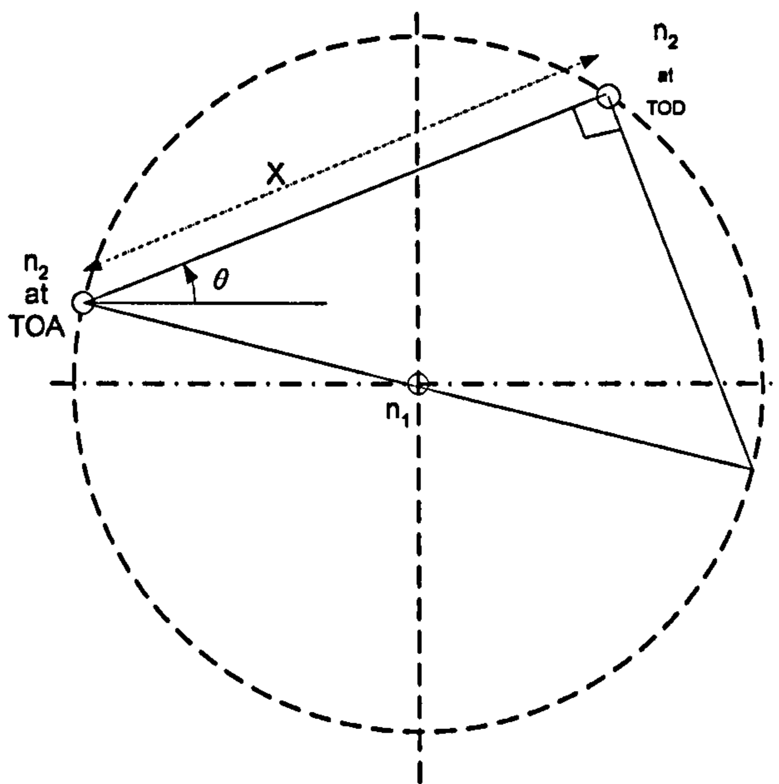
Figure 4-4 Estimating the Expected Node Connectivity Time
