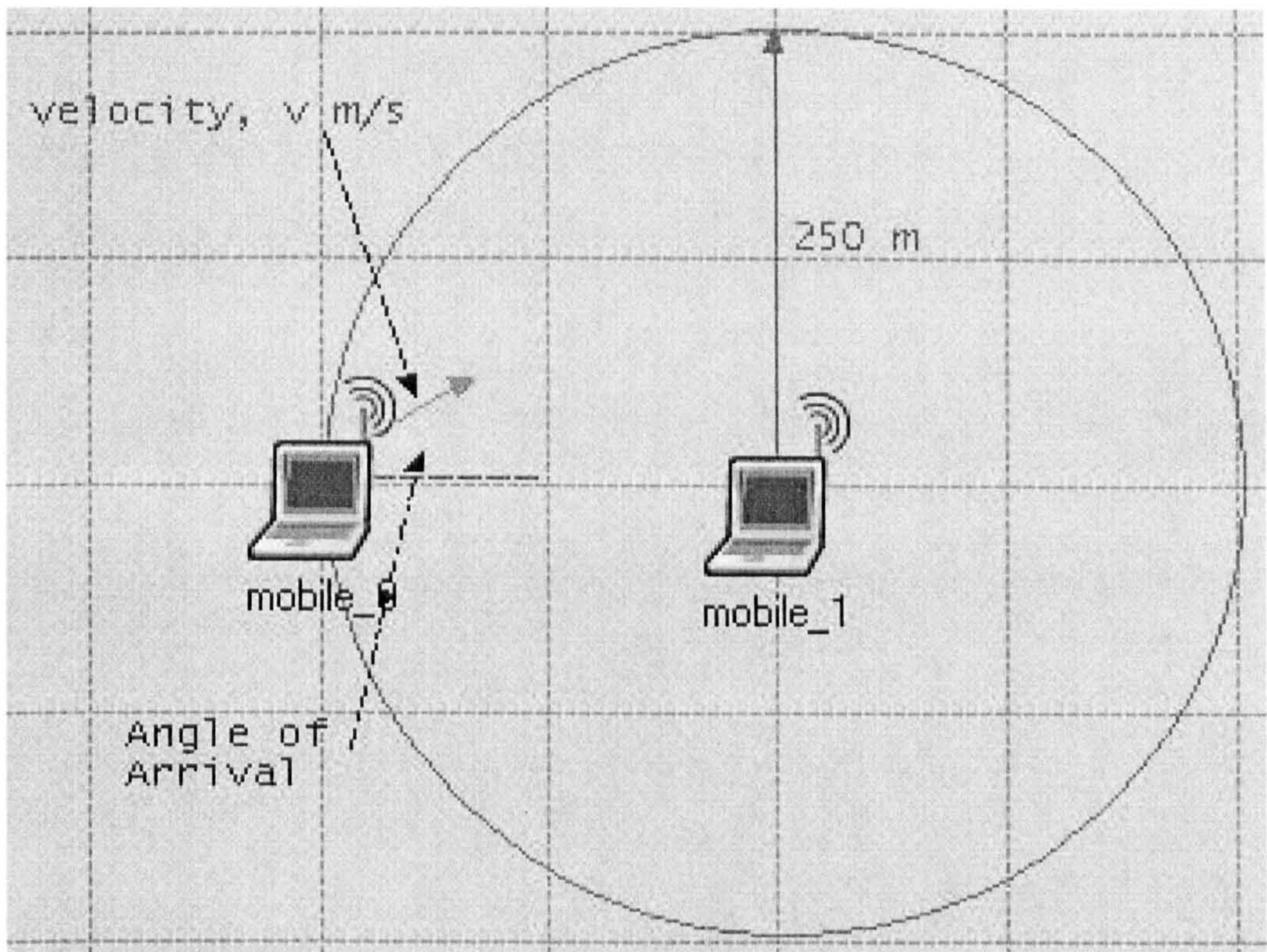
Figure 4-8 Scenario to Determine nci
