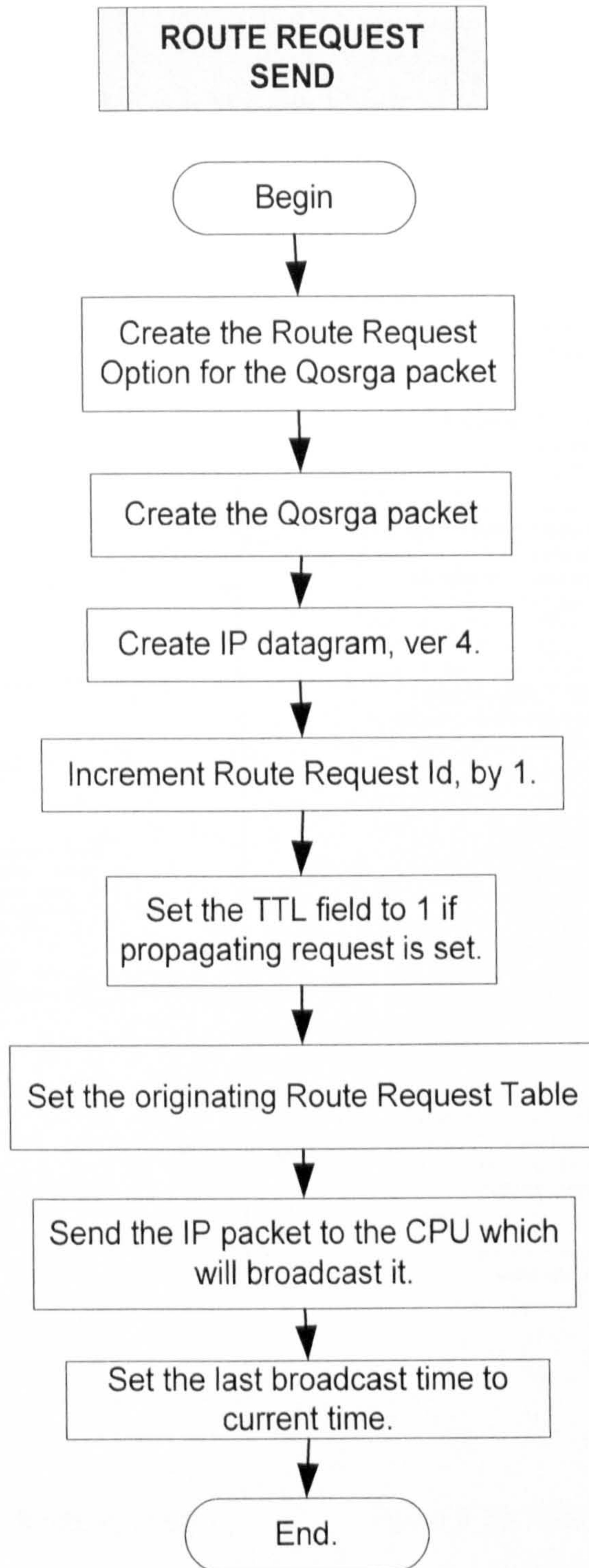
Figure 3-16 Route Request Send Operation
