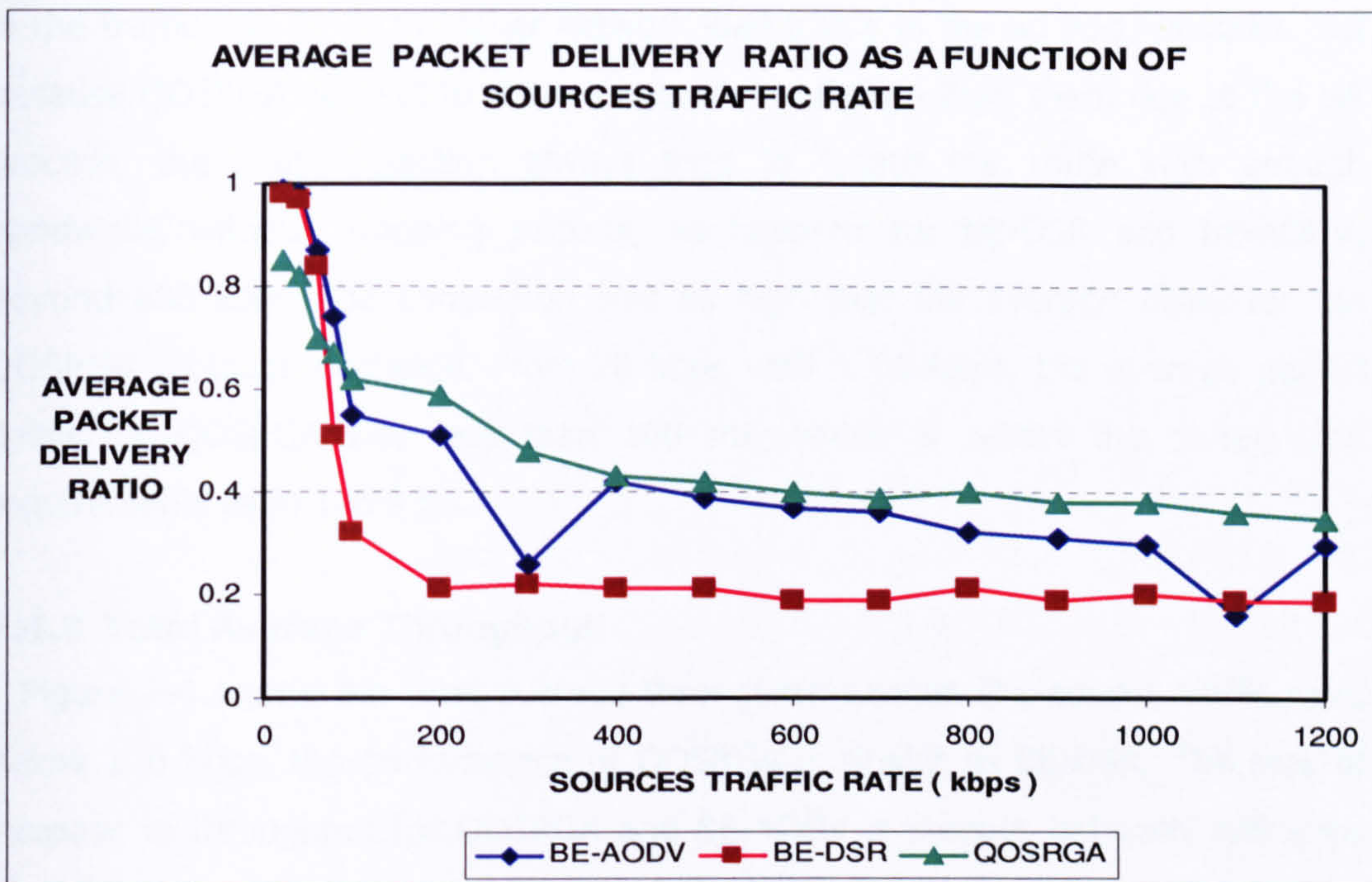
Figure 7.2 APDR against the Source Traffic Rates
