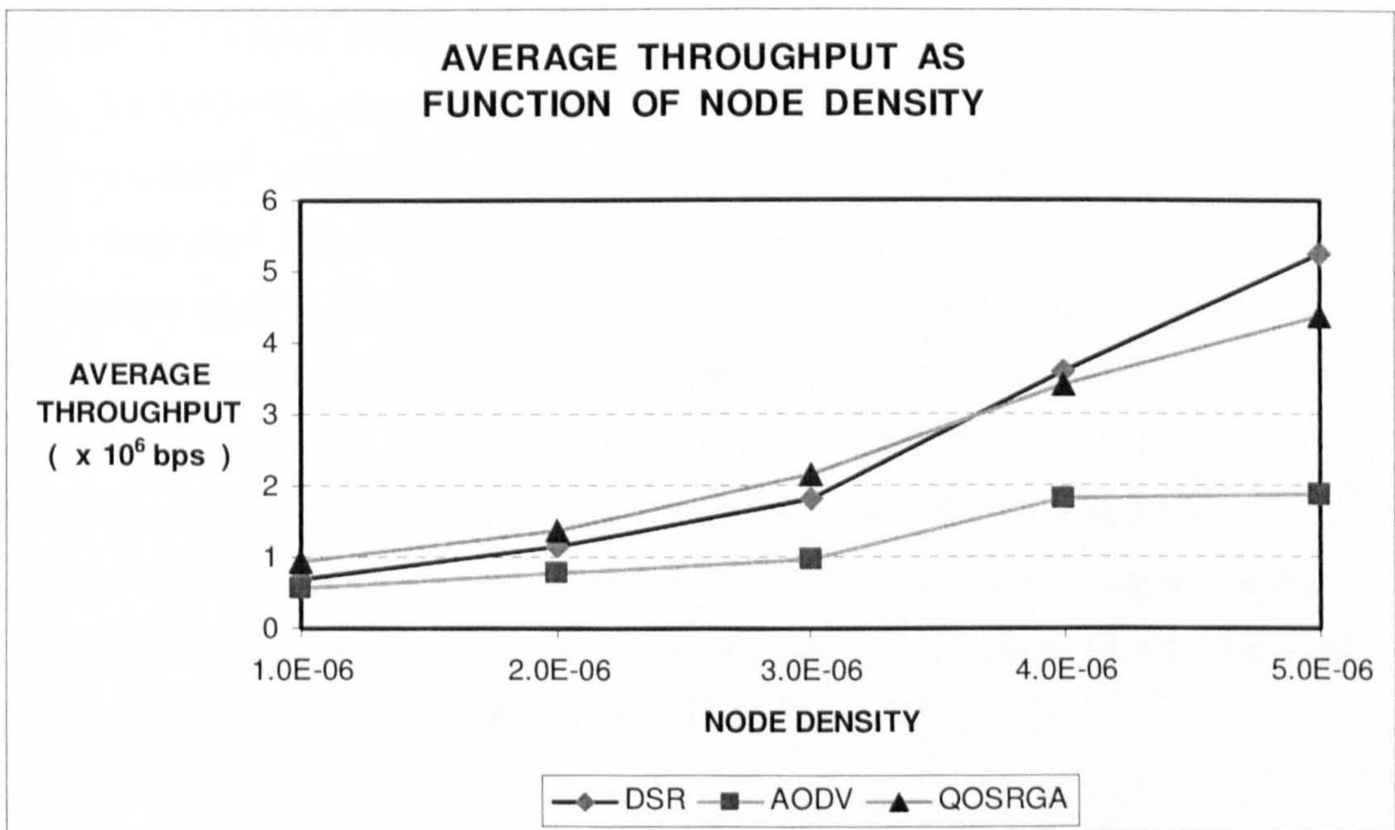
Figure 7.11 Average Total Throughput against Node Density
