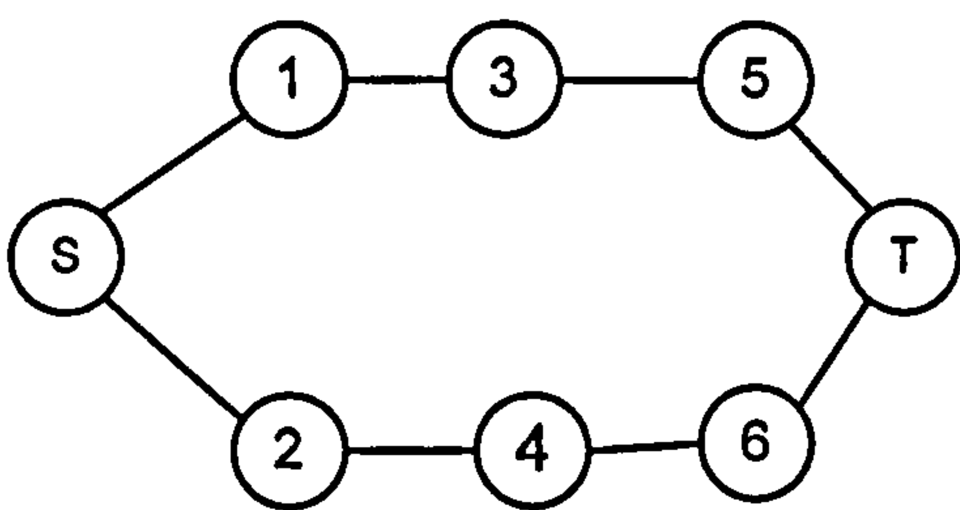
Figure 3-11 Disjoint Network
