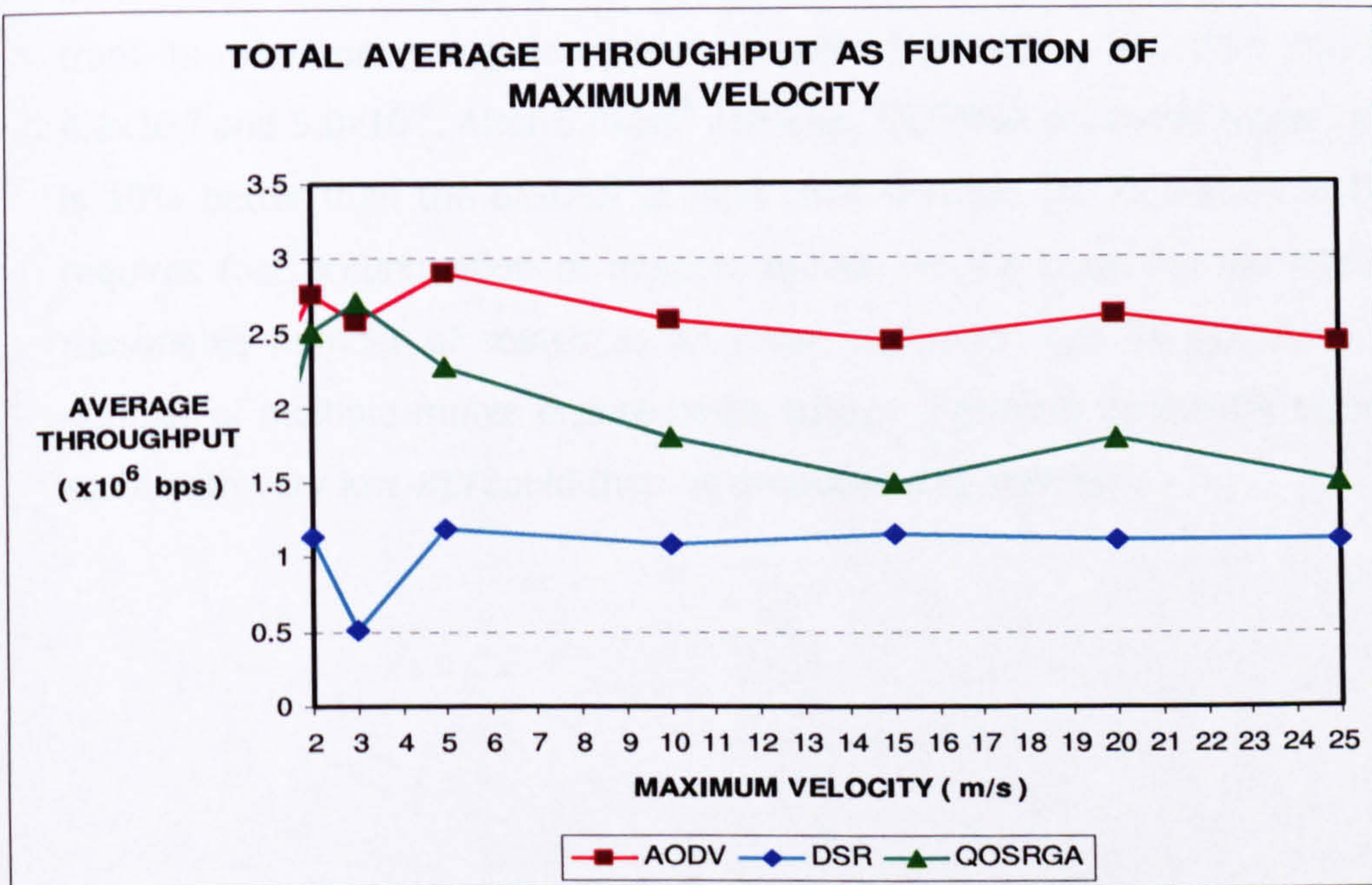
Figure 7.7 Average Total Throughput against Mobility Level
