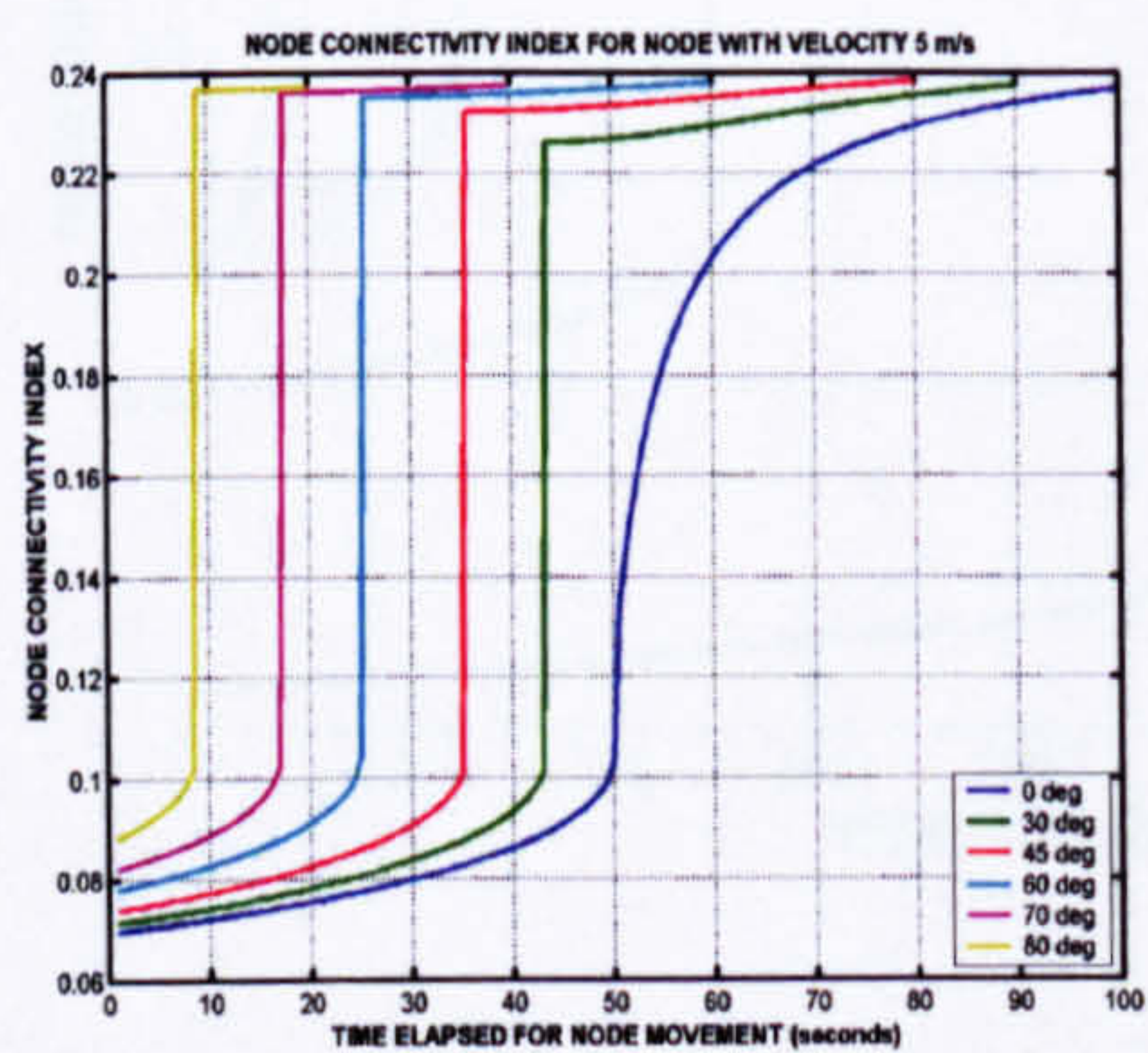
Figure 4-13 nci for velocity 5 m/s
