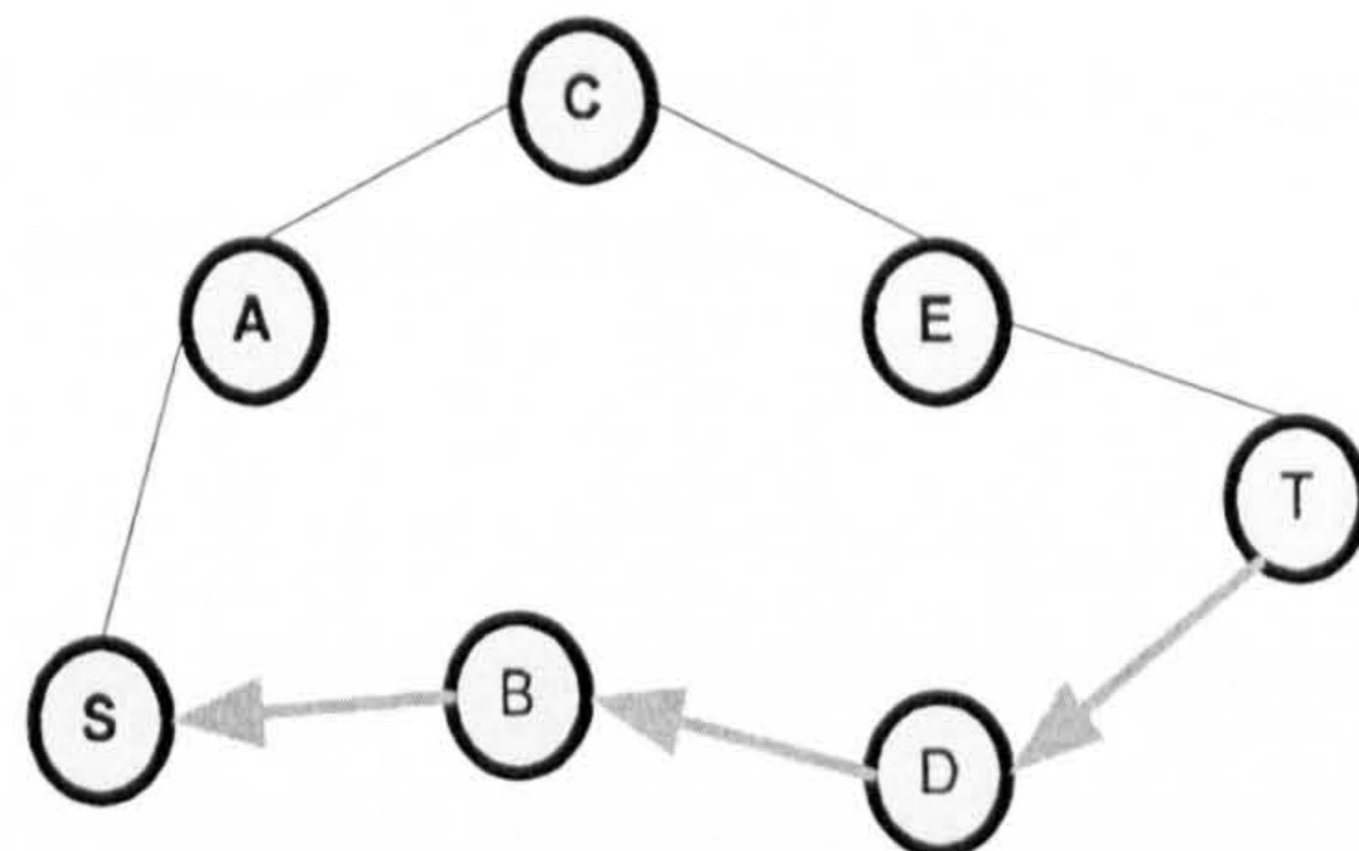
Figure 2-6 RREP Propagation to the Source
