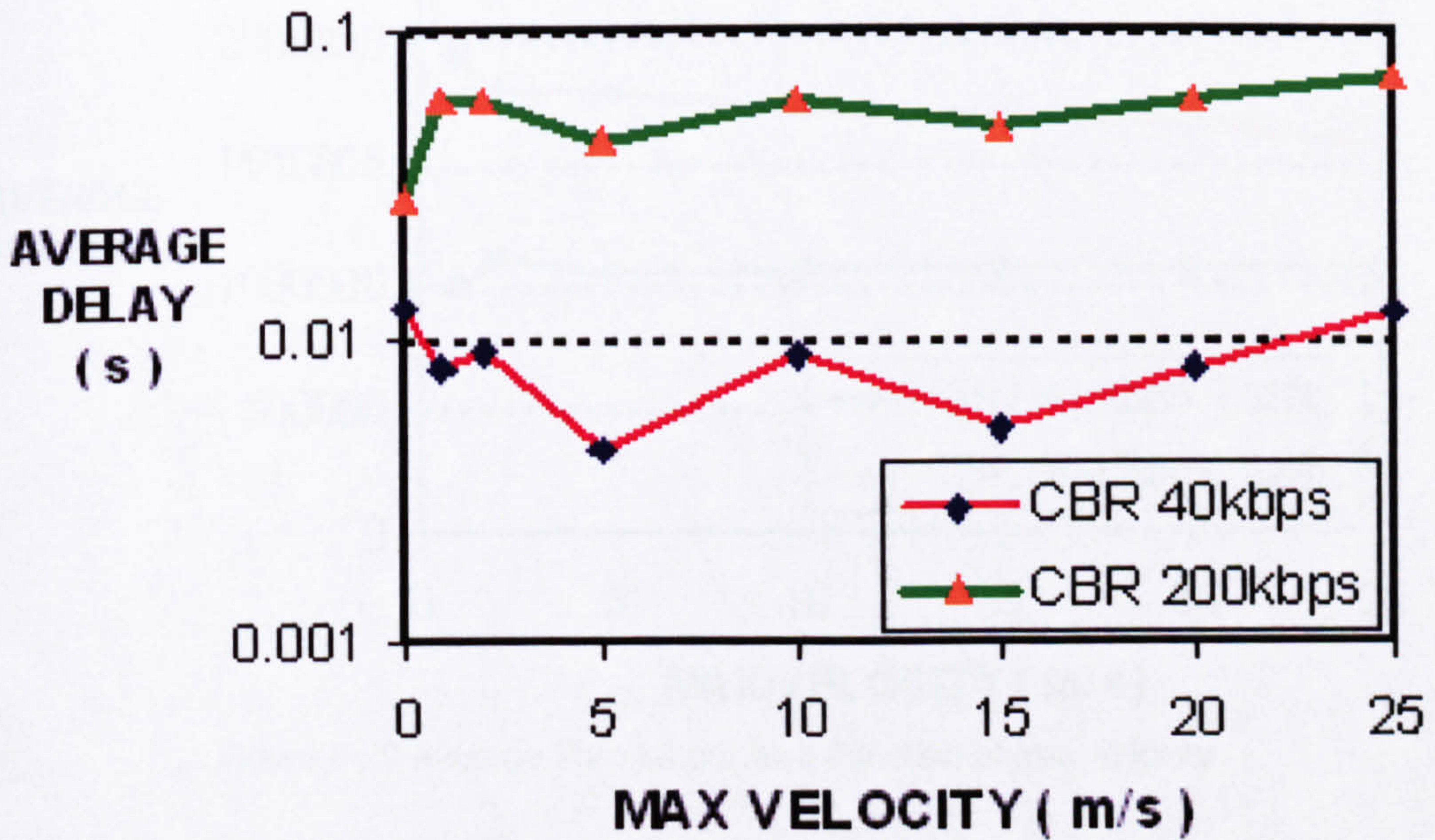
Figure 6-18 Average Packet Delay as a Function of Max Velocity
