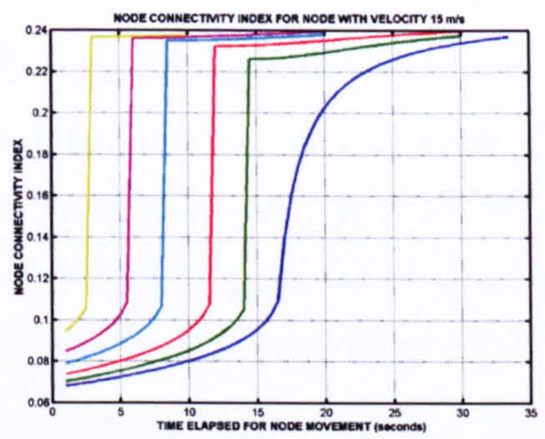
Figure 4-16 nci for velocity 15 m/s
