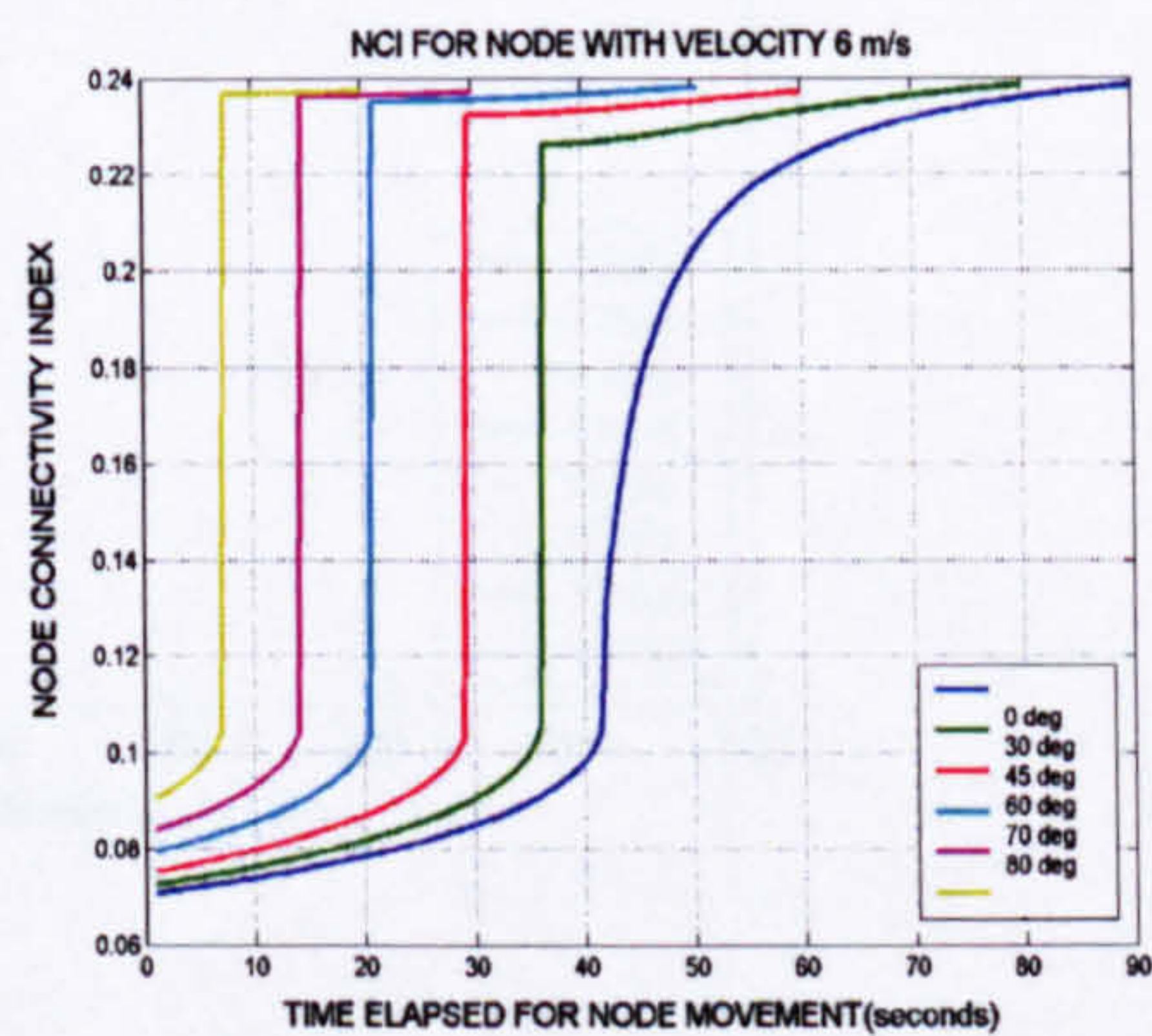
Figure 4-14 nci for velocity 6 m/s
