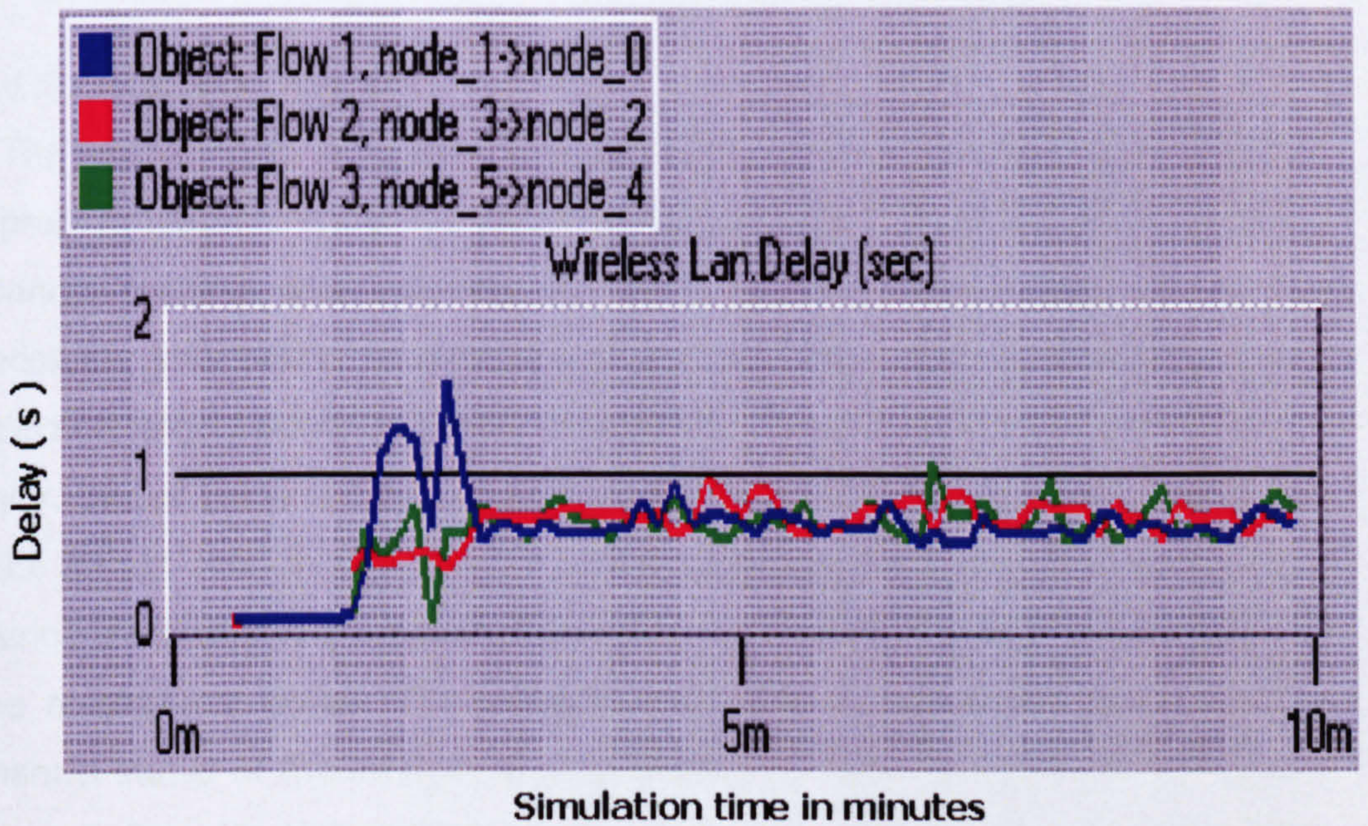
Figure 5-7 Delay for flows 1,2,3
