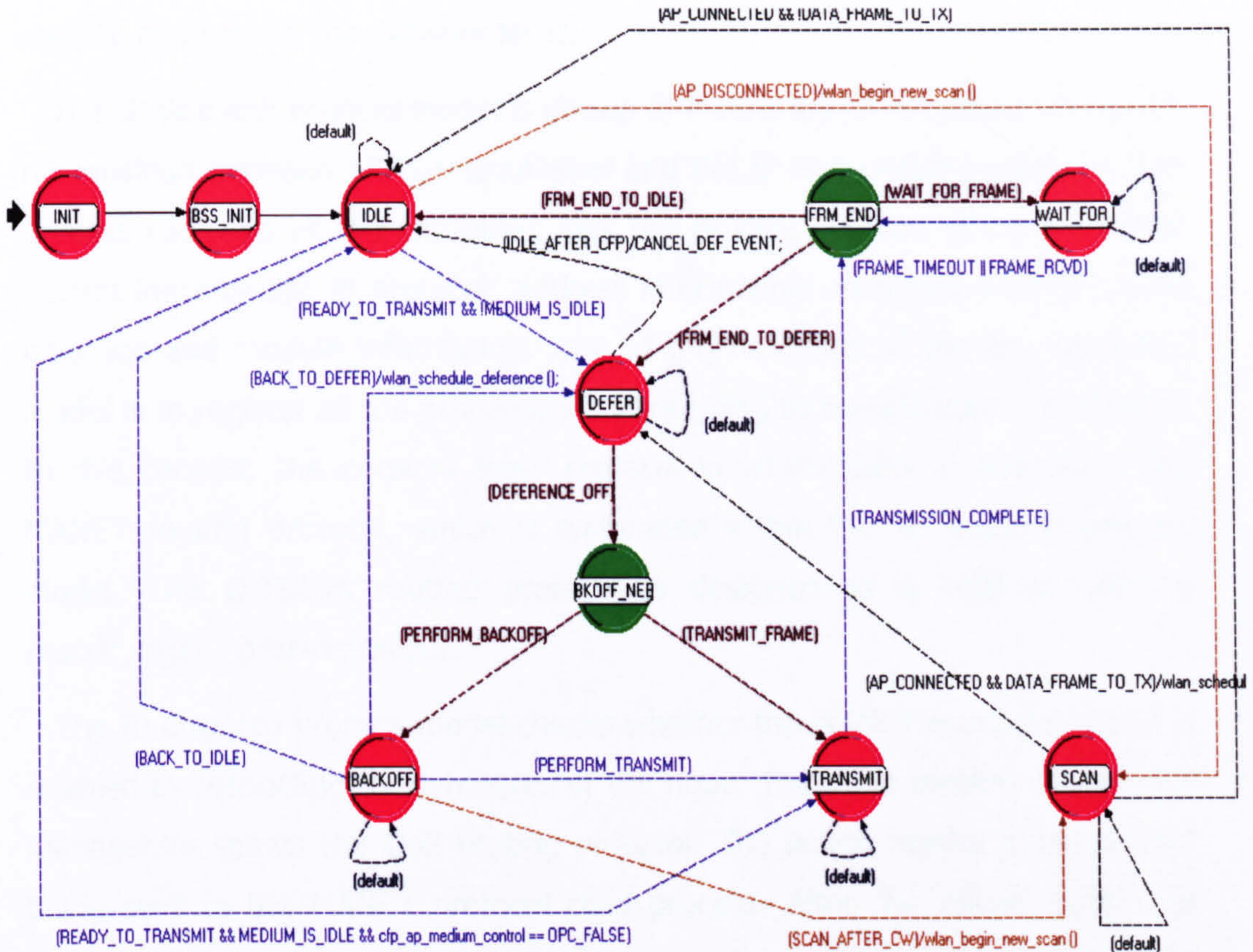
Figure 3-3 WLAN MAC Process Model [29]
