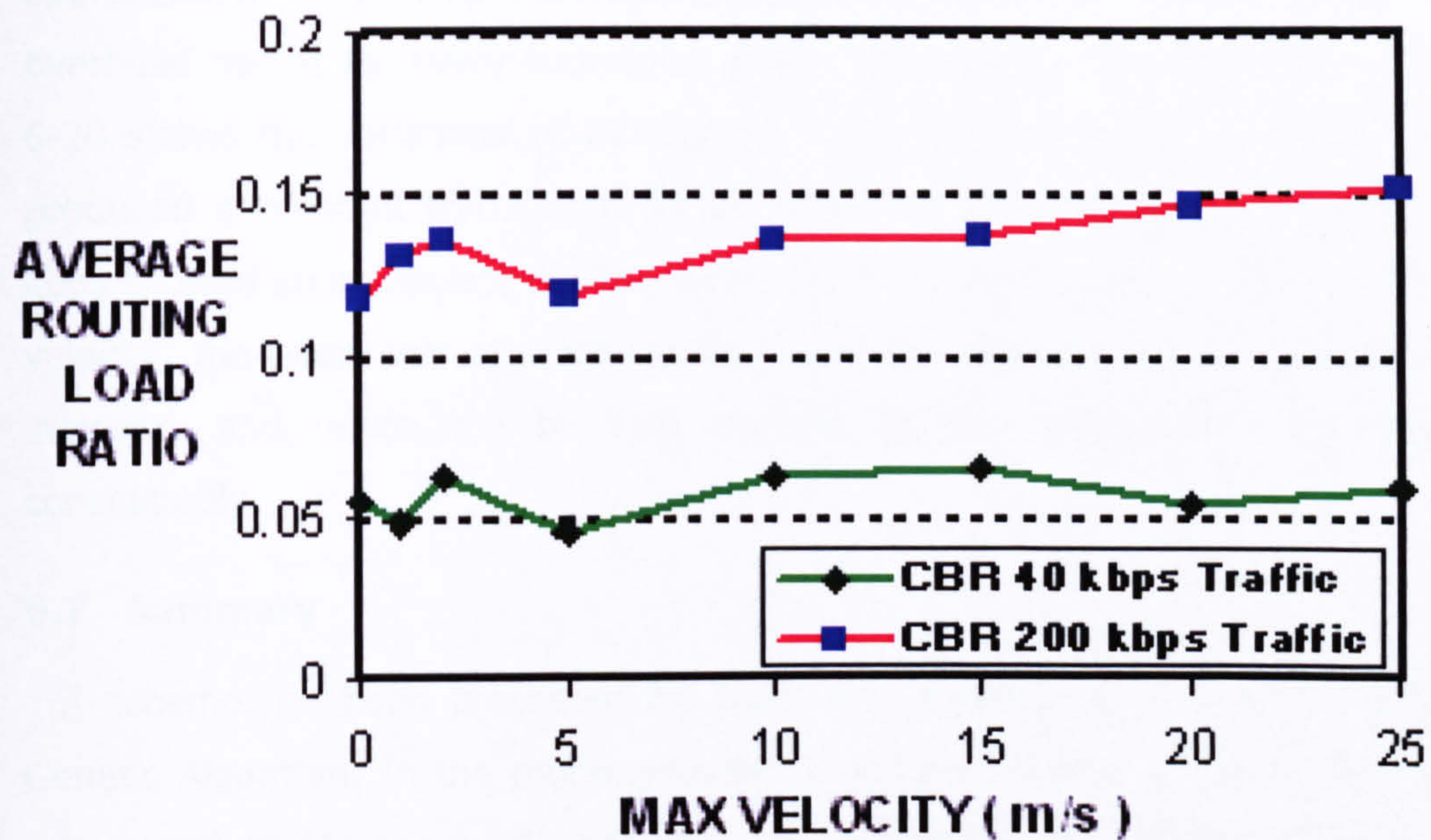
Figure 6-19 Average Routing Load as a Function of Max Velocity
