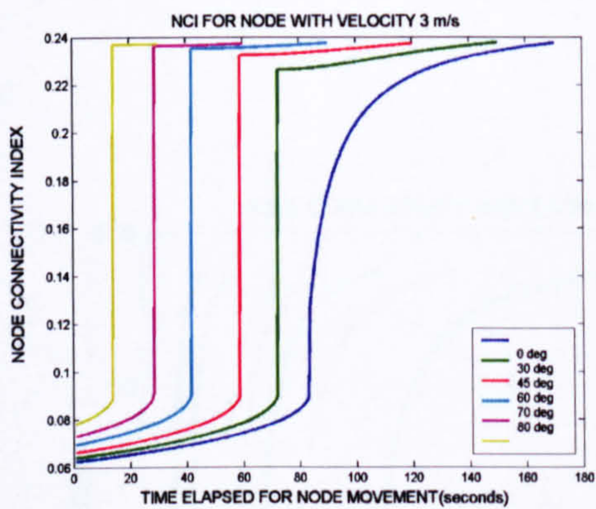
Figure 4-11 nci for velocity 3 m/s
