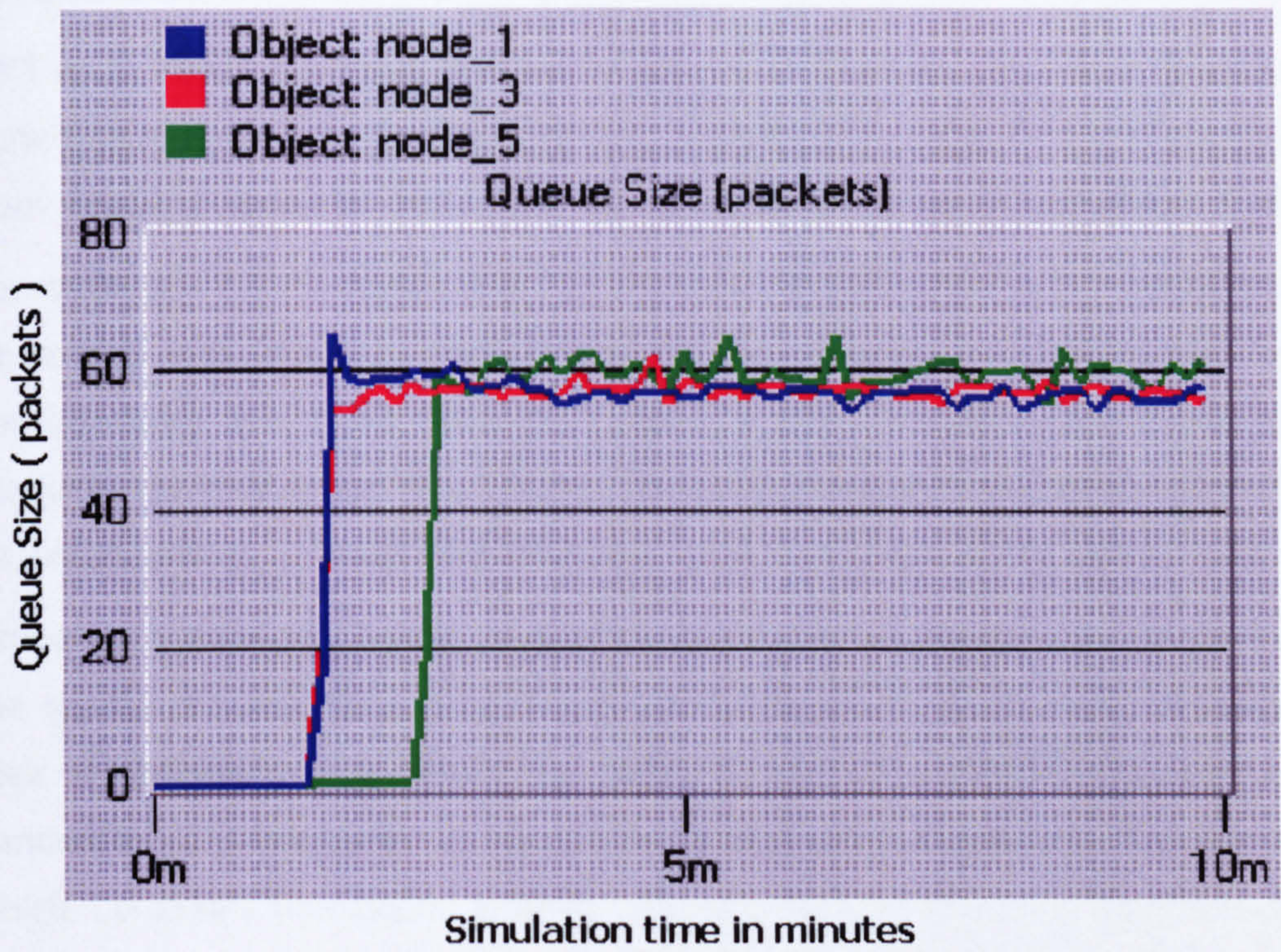
Figure 5-6 Queue at the Node's Transmitter
