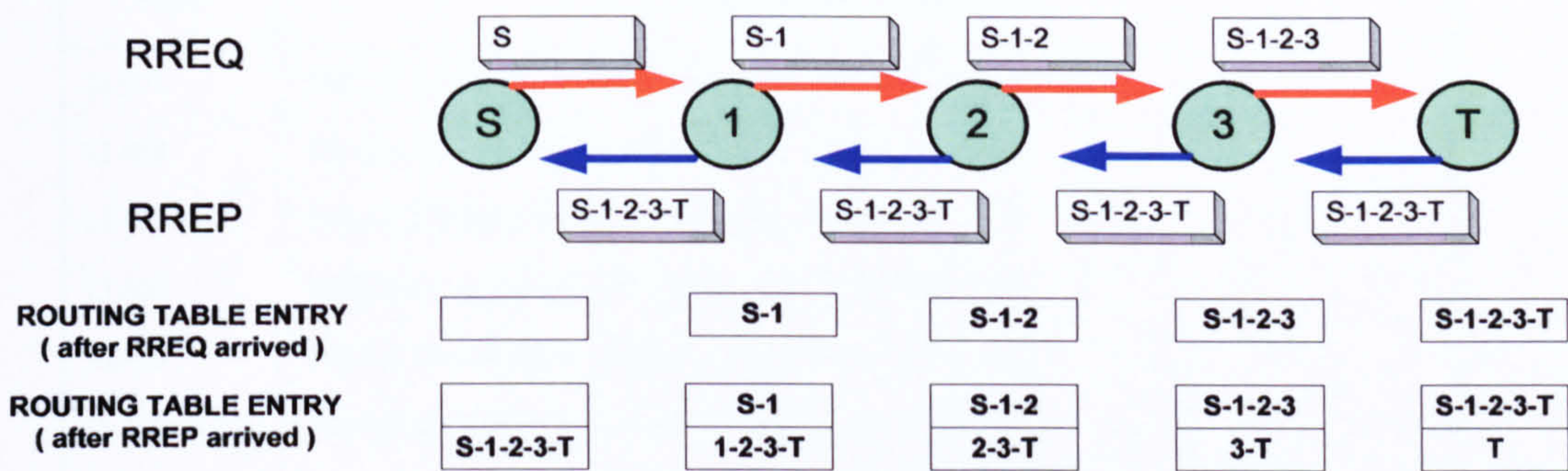
(a) Process Of Route Accumulation
