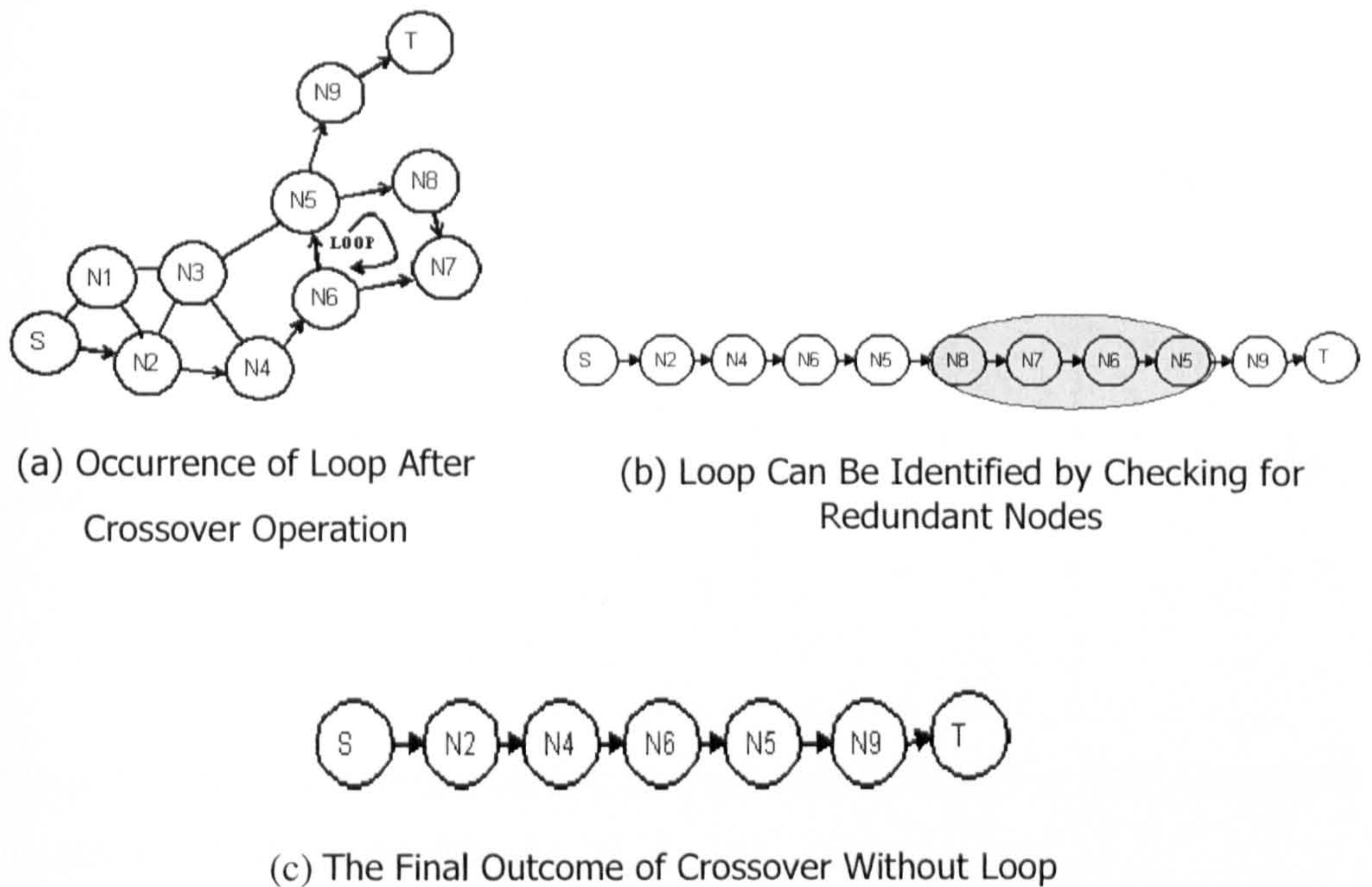
Figure 6-4 Restoration Operation
