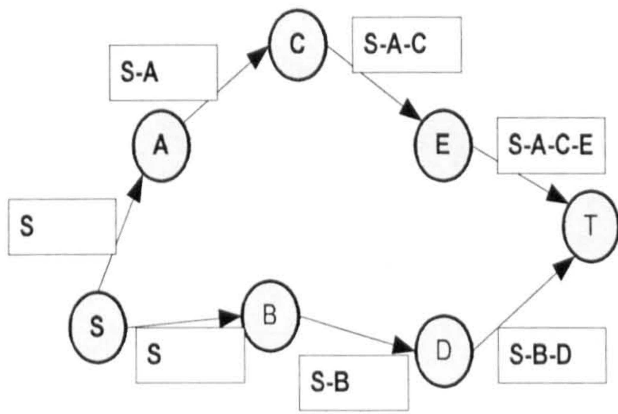
Figure 2-3 Propagating Route Request for BE-DSR
