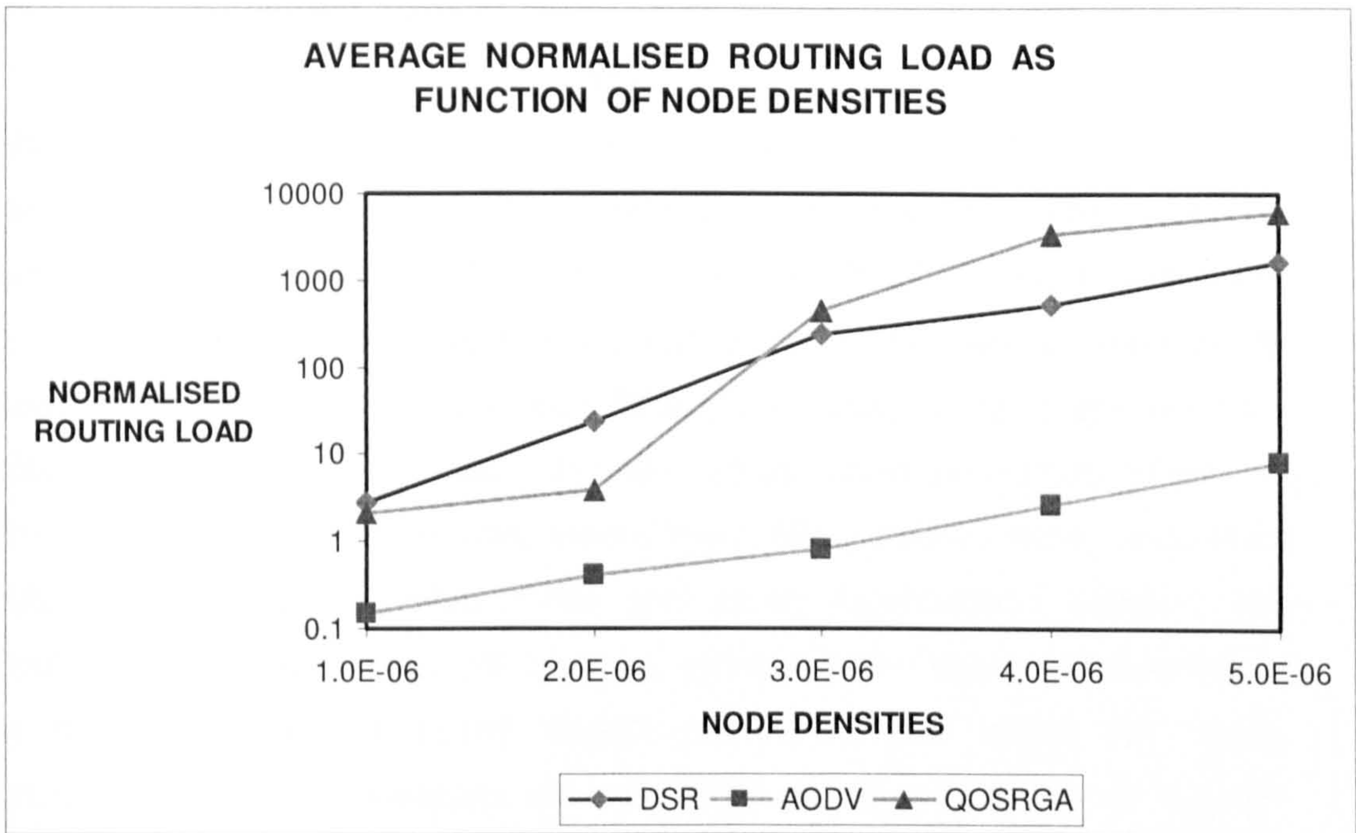
Figure 7.10 Average Normalised Routing Load against Node Density
