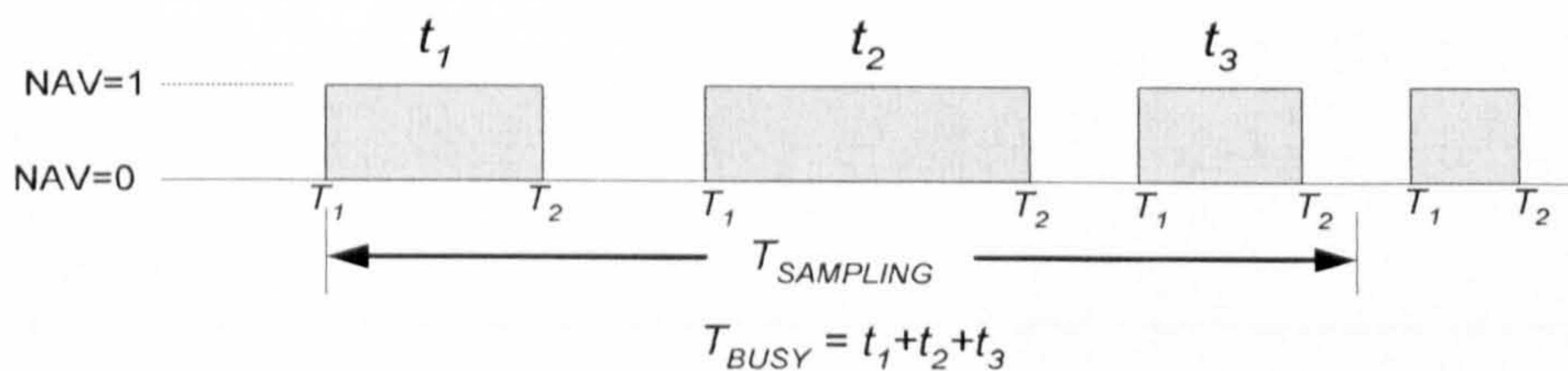
Figure 5.10 The Occupancy of Wireless Medium
