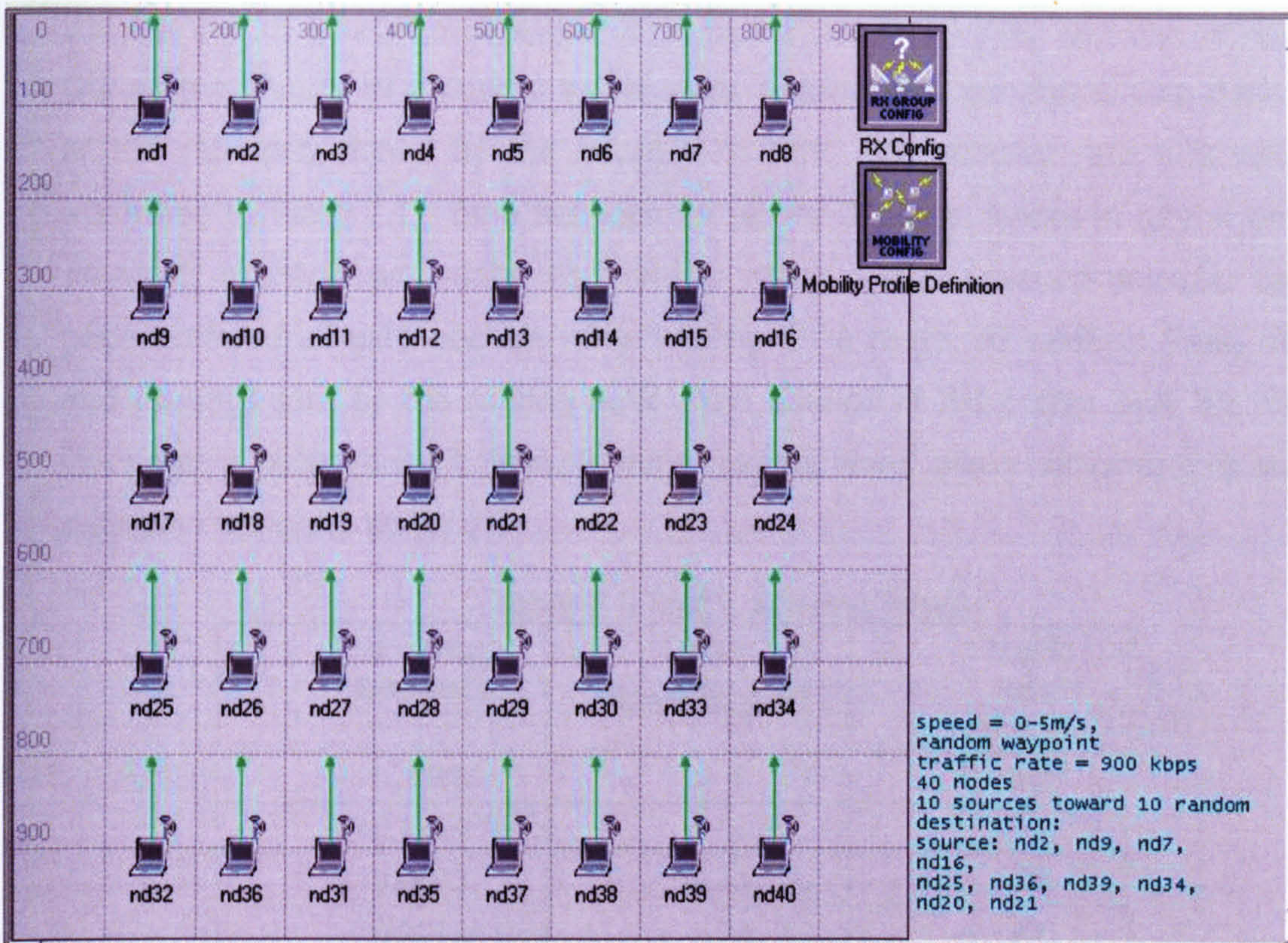
Figure 7-1 The Initial Setup of Simulation Environment with 40 Nodes
