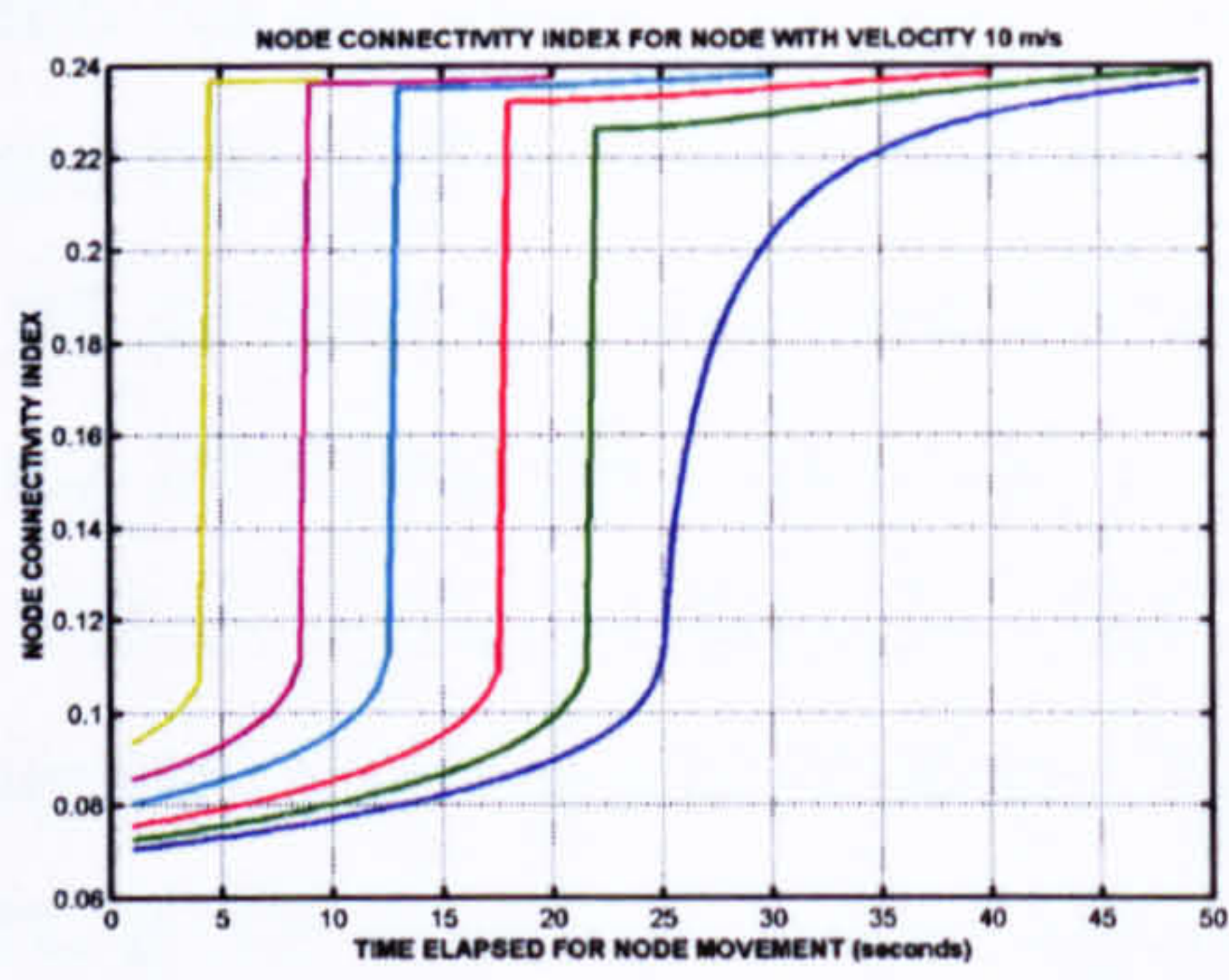
Figure 4-15 nci for velocity 10 m/s
