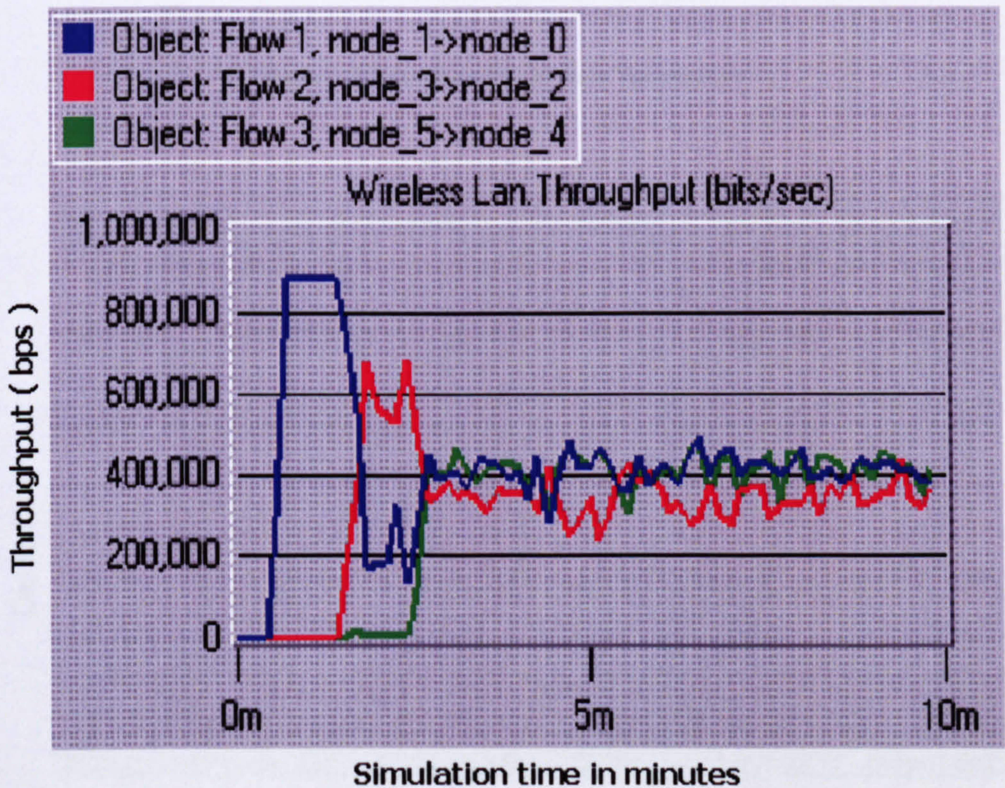
Figure 5-5 Throughput for Flows 1, 2, 3
