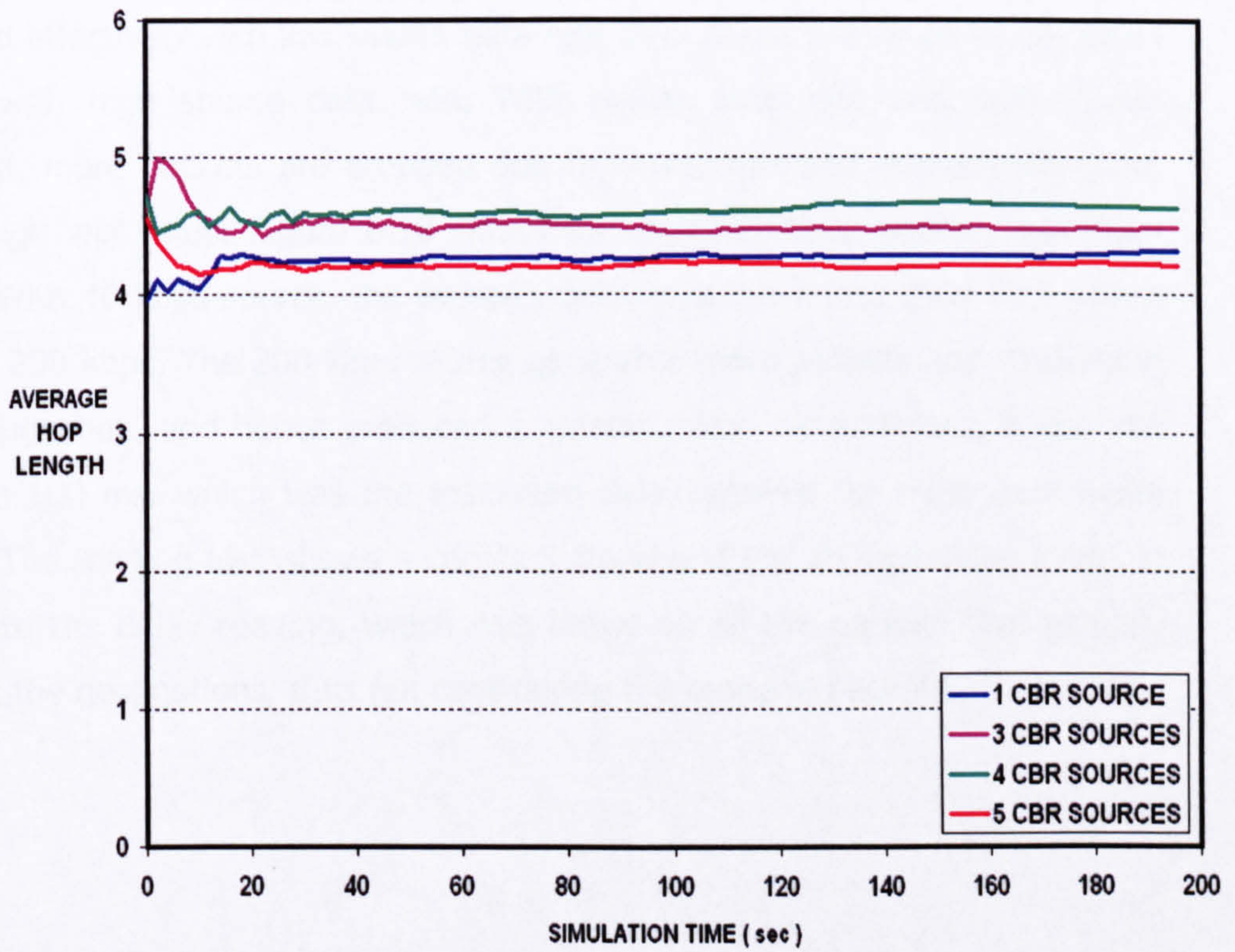
Figure 6-16 Average Number of Hops for Each Destination
