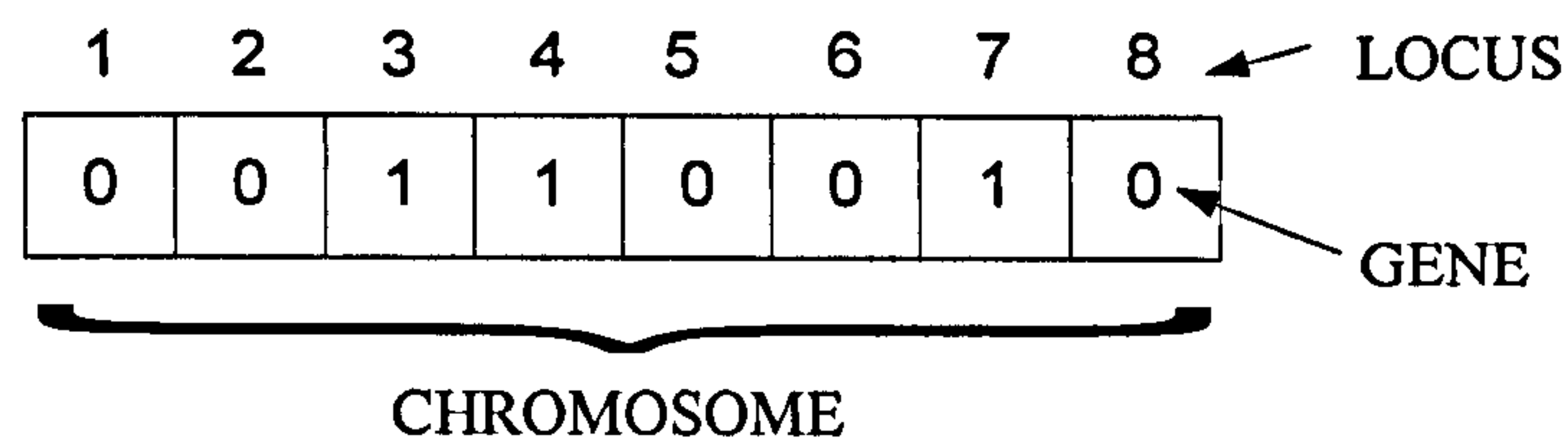
Figure 2-9 Chromosome Representation
