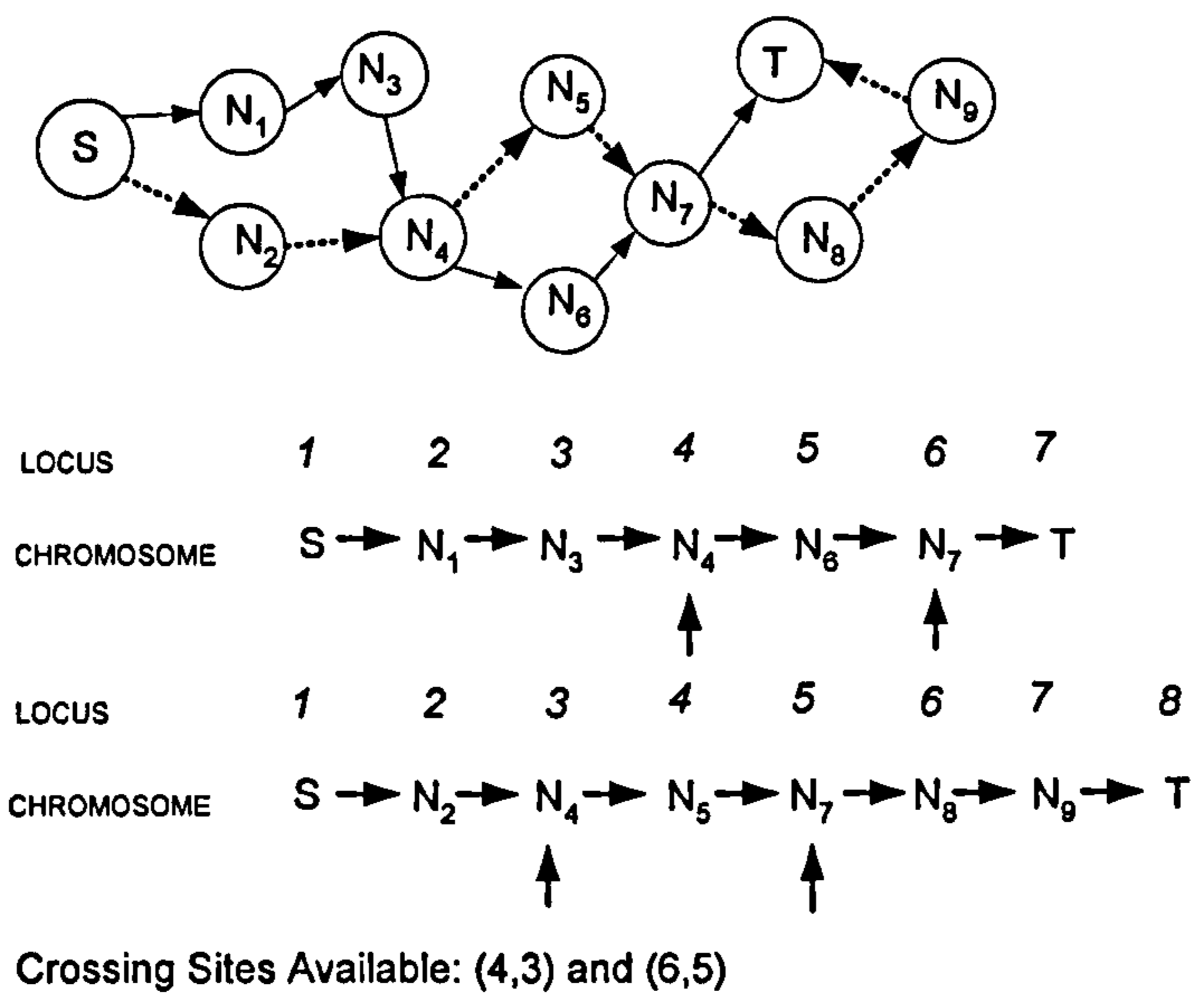
Figure 6-3 Route Crossover
