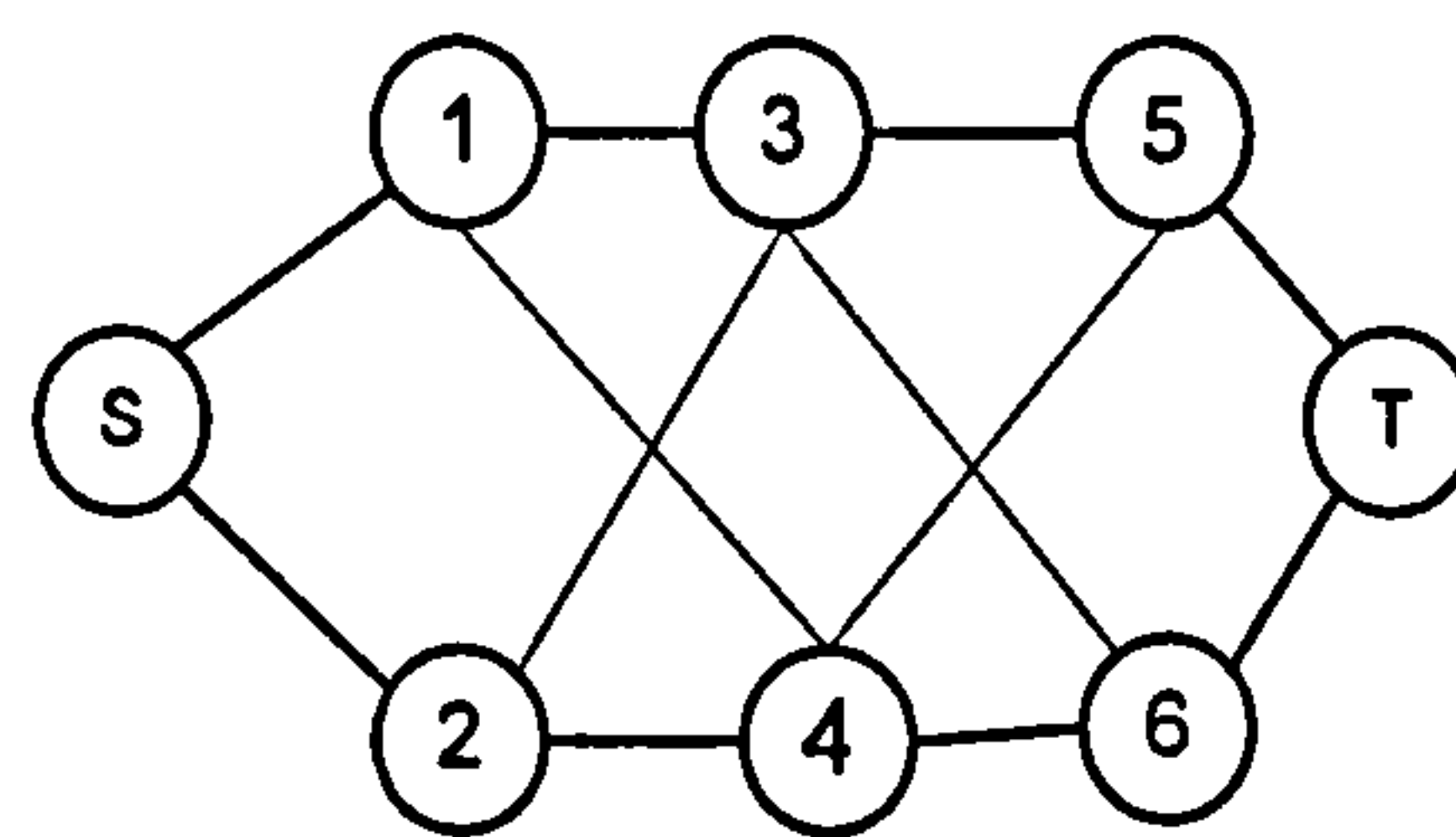
Figure 3-12 Non-Disjoint Network
