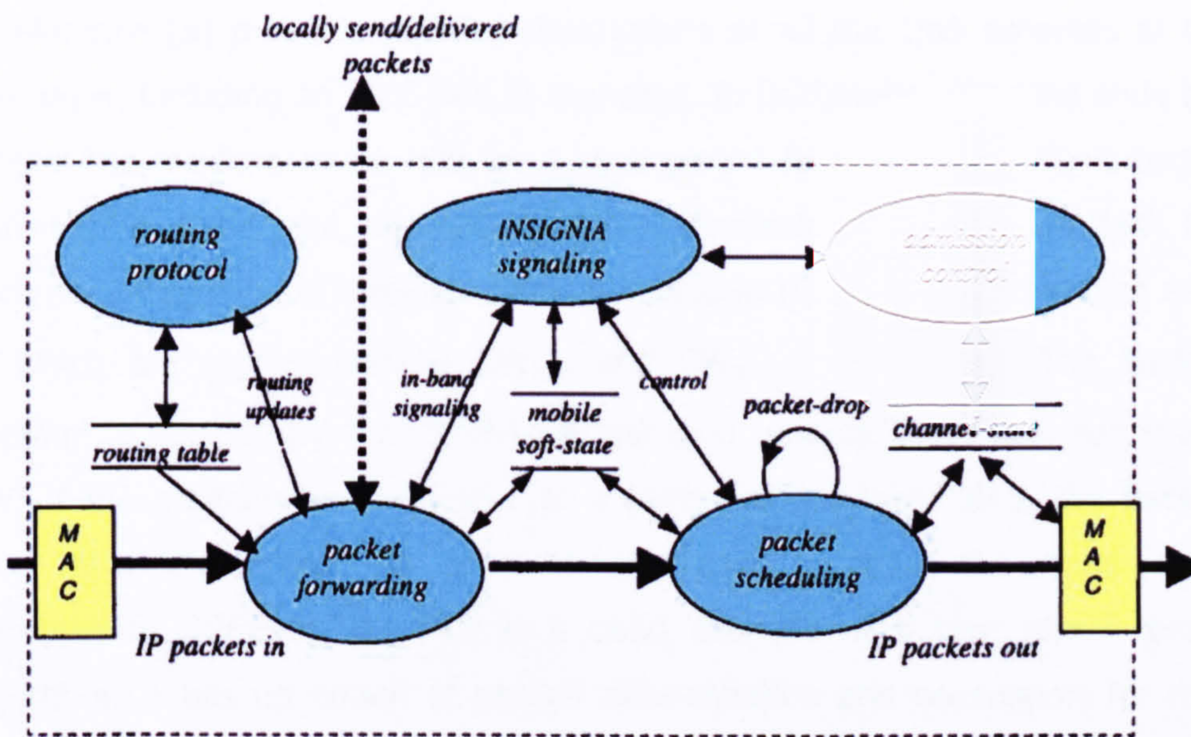
Figure 2-1 INSIGNIA Framework [3]
