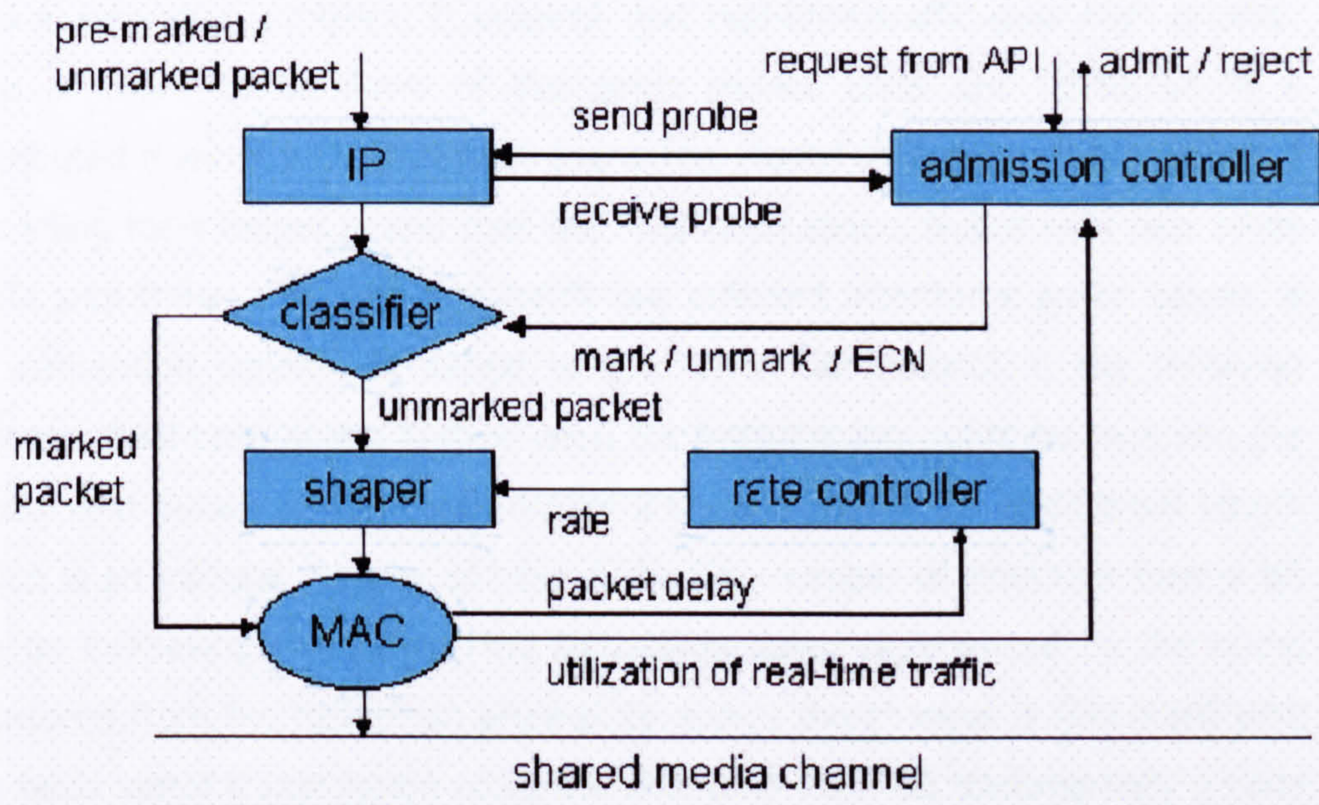
Figure 2-2 SWAN Framework [4]
