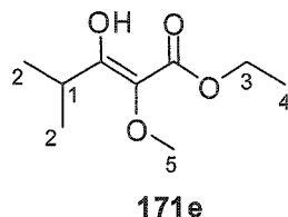
Figure 17. Suggested by-product 171e from conversion of picolinate 168e into bipyridine 116e .
