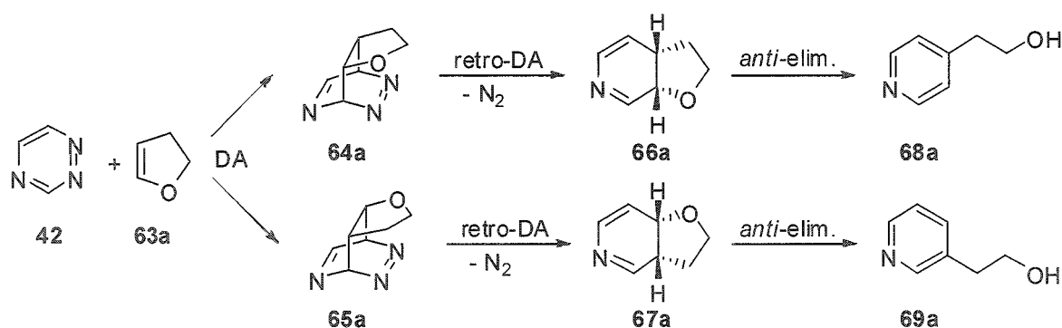
Scheme 11. Cyclic vinyl ethers in aza Diels-Alder reactions.
