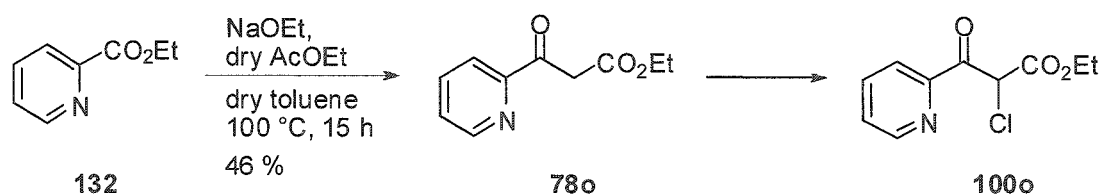
Scheme 32. Preparation and attempted \alpha -chlorination of \beta -keto- \beta -(2-pyridyl) ester 78o .
