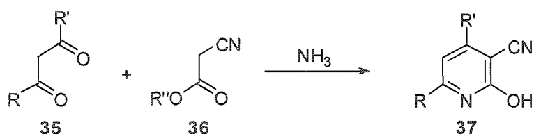
Scheme 4. Example of a GUARESCHI-Synthesis.
