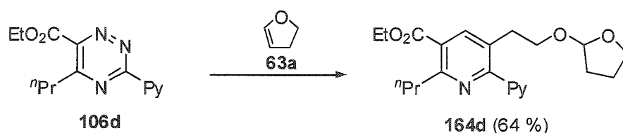
Scheme 49. DA reaction using cyclic vinyl ether 63a .
