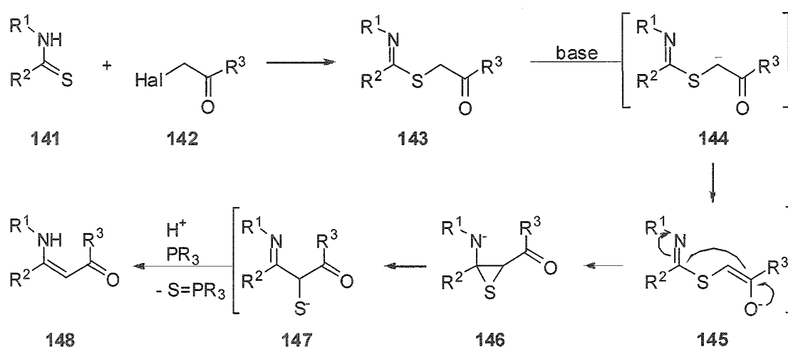
Scheme 39. Mechanism of the Eschenmoser sulfide contraction.
