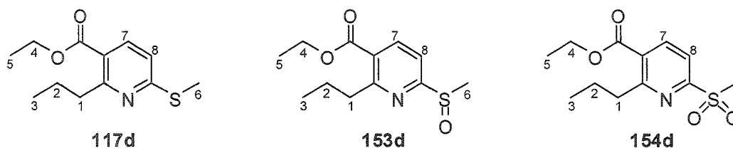
Figure 12. Sulfur-containing pyridines.
