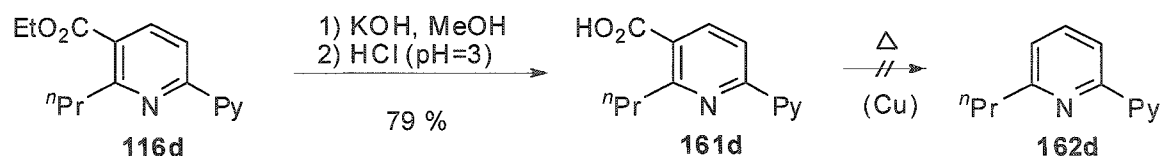
Scheme 47. (Attempted) FGI of the ester group in pyridine 116d .
