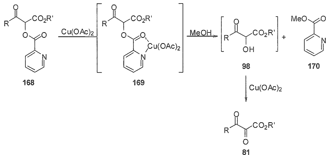
Scheme 52. A novel route to \alpha,\beta -diketo esters 81 .
