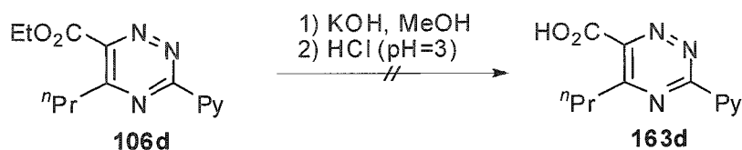
Scheme 48. Attempted FGI of the ester group in triazine 106d .
