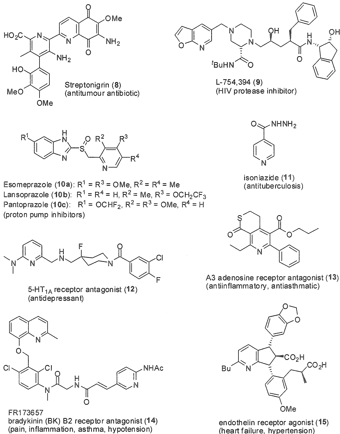
Figure 3. Pyridine-based pharmaceuticals.
