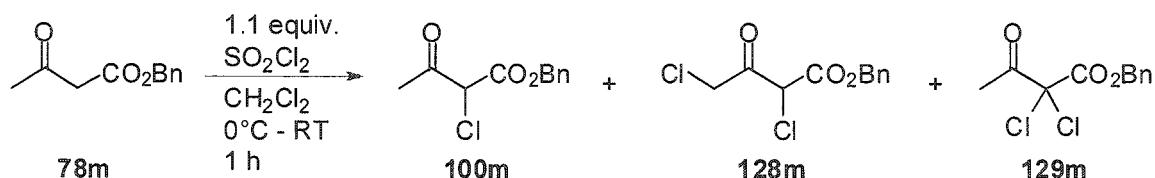
Scheme 29. Product mixture from \alpha -chlorination of 78m .
