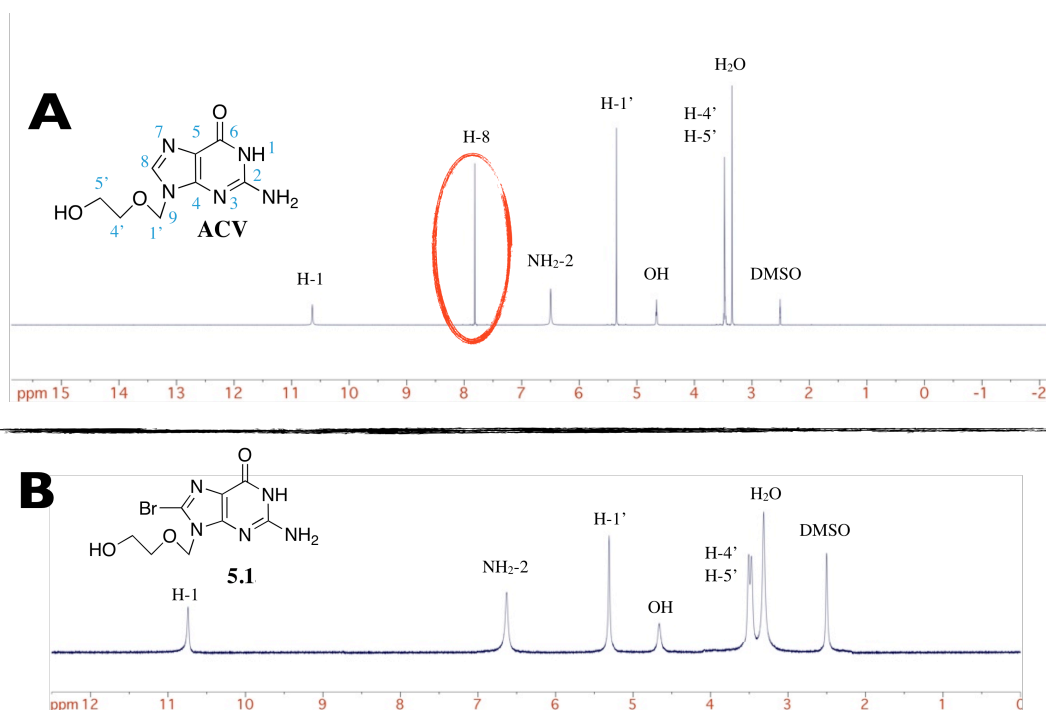
Figure 5.2. H-NMR spectra (DMSO, 500 MHz) of (A) ACV and (B) 8-bromoacyclovir
