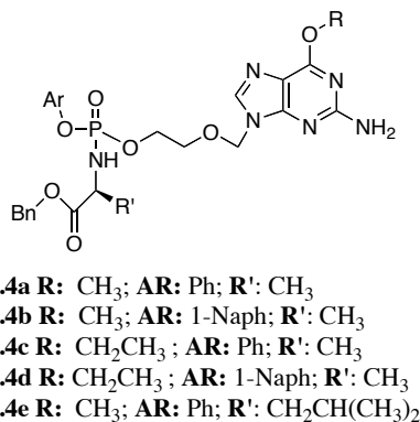
Figure 4.5 Structure of aryl phosphoramidate derivatives 4.4a-e
