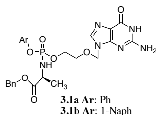
Figure 3.2 L-alanine benzyl ester derivatives 3.1a and 3.1b
