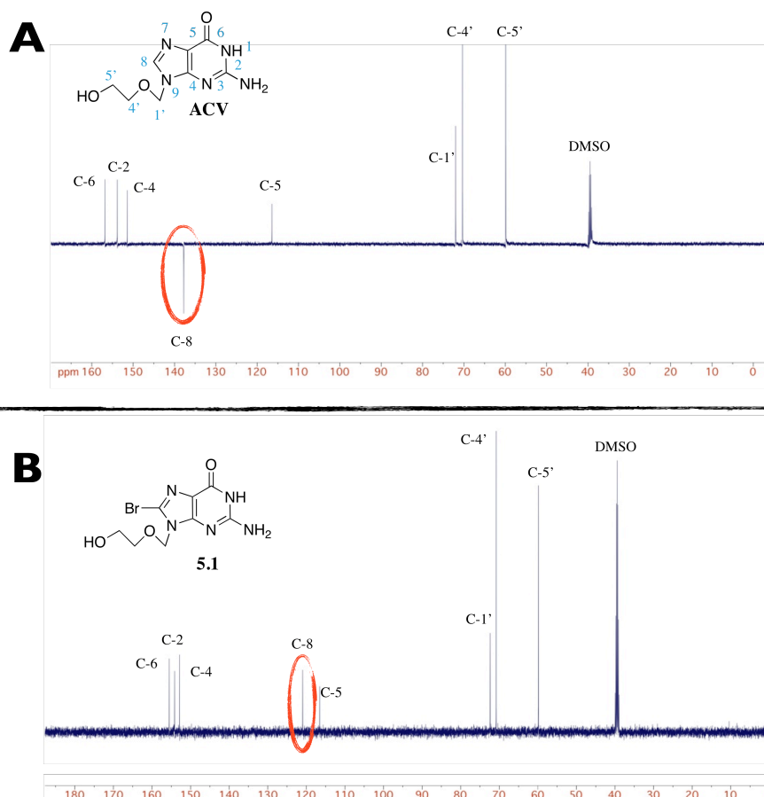
Figure 5.3. ^{13}\text{C} -NMR spectra (DMSO, 125 MHz) of (A) ACV and (B) 8-bromoacyclovir
