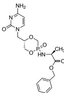
Figure 7.7. Structure of the phosphonoamidate 7.4 .
