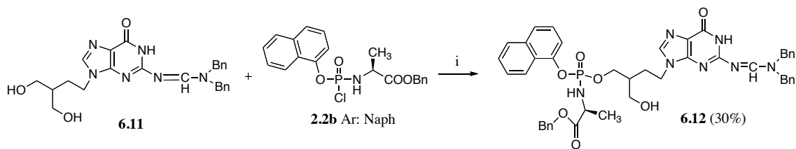
Scheme 6.6. Coupling reaction of N,N -dibenzyl-formamide-protected PCV with the phosphorochloridate 2.2b.
