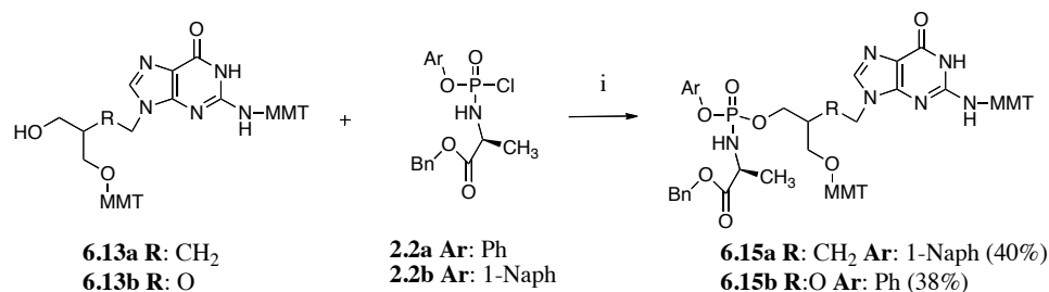
Scheme 6.8. Coupling reaction of 6.13a and 6.13b with the phosphorochloridates 2.2a and 2.2b
