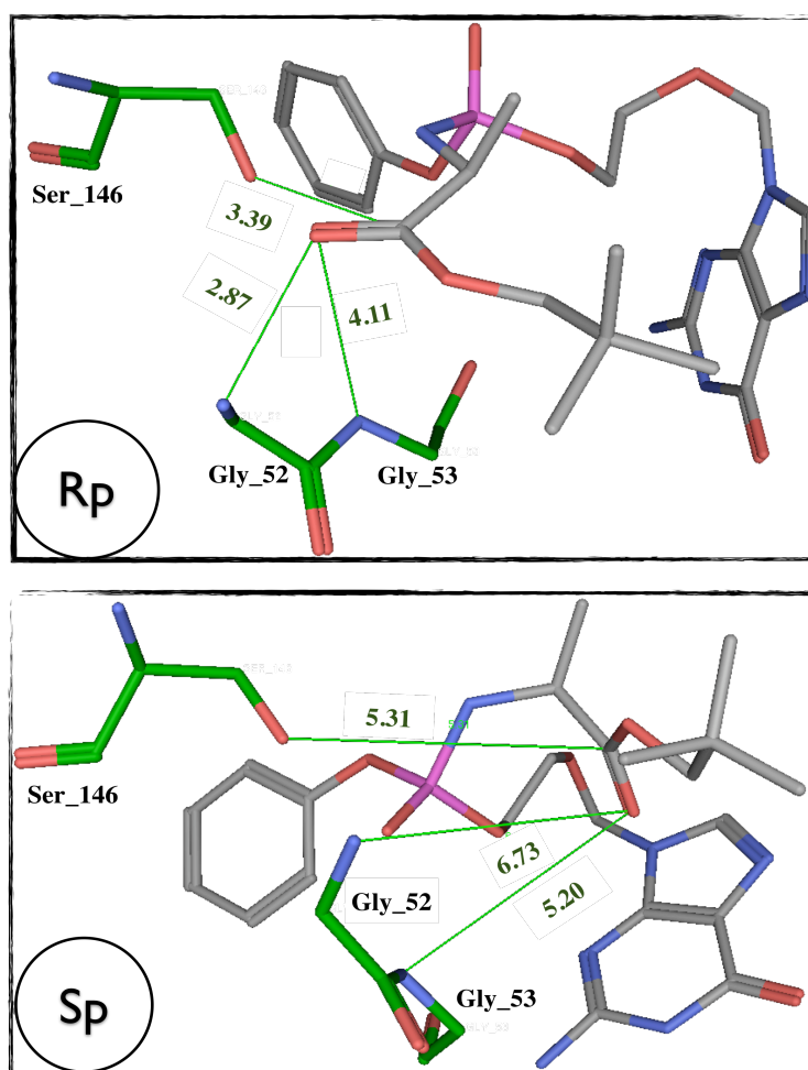
Figure 3.15. Detail of the docking of 3.2I ( Rp and Sp diastereomers) within the active site of CPY showing the orientation and the distance in angstroms of the carboxyl group toward the glycine and serine residues (Gly52, Gly53, and Ser146) responsible for its cleavage.
