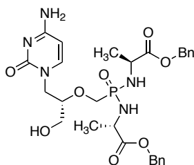
Figure 7.6. Structure of the phosphonodiamidate 7.3
