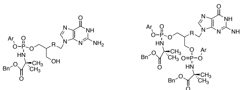
6.6a R: CH 2 Ar: Ph 6.6b R: CH 2 Ar: 1-NaPh 6.6c R: O Ar: Ph 6.6d R: O Ar: 1-Naph
