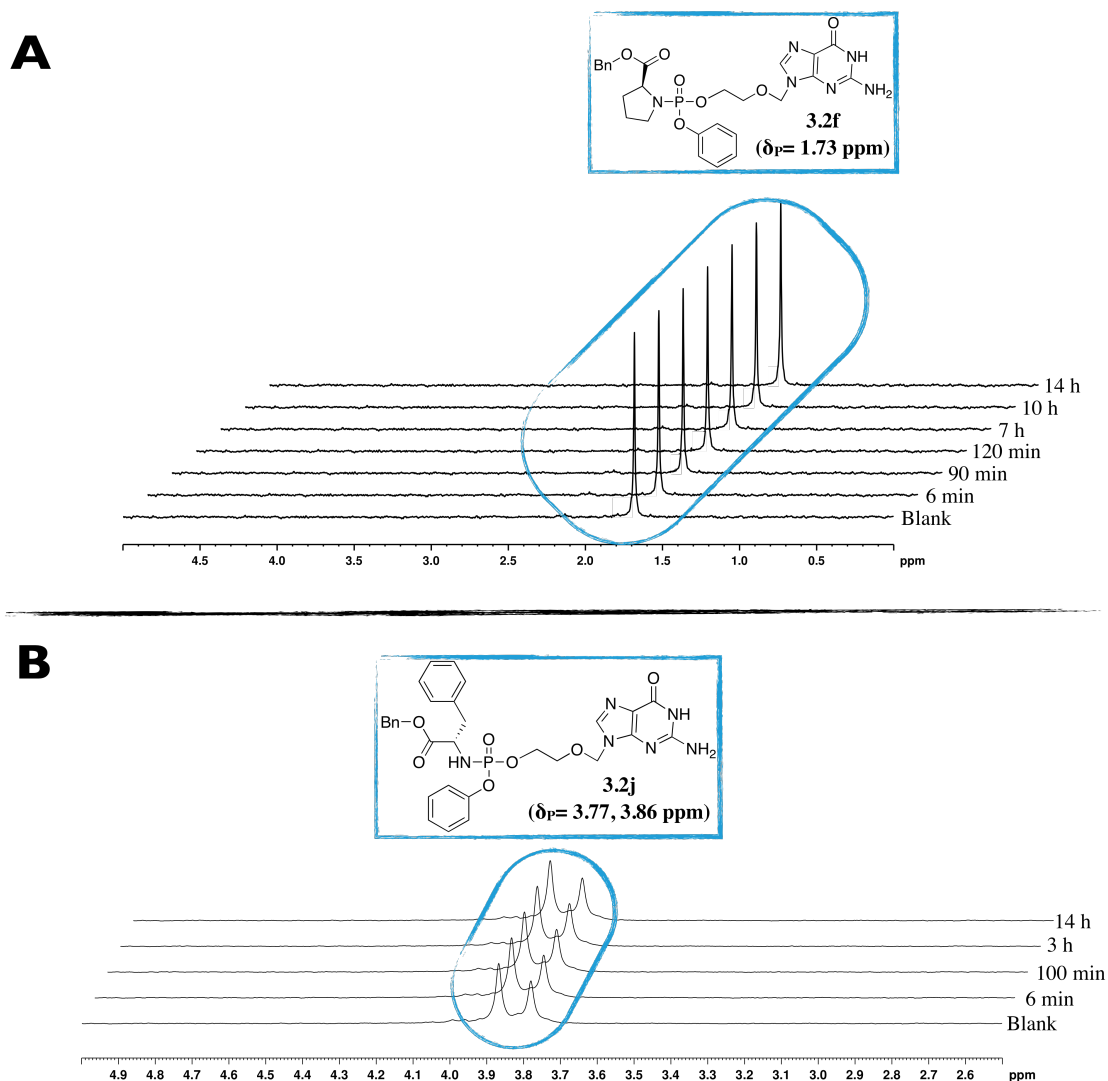
Figure 3.6. ^{31}\text{P} NMR spectra (acetone- \text{D}_6 , 202 MHz) at different time of the enzymatic study performed on compound (A) 3.2f and (B) 3.2j
