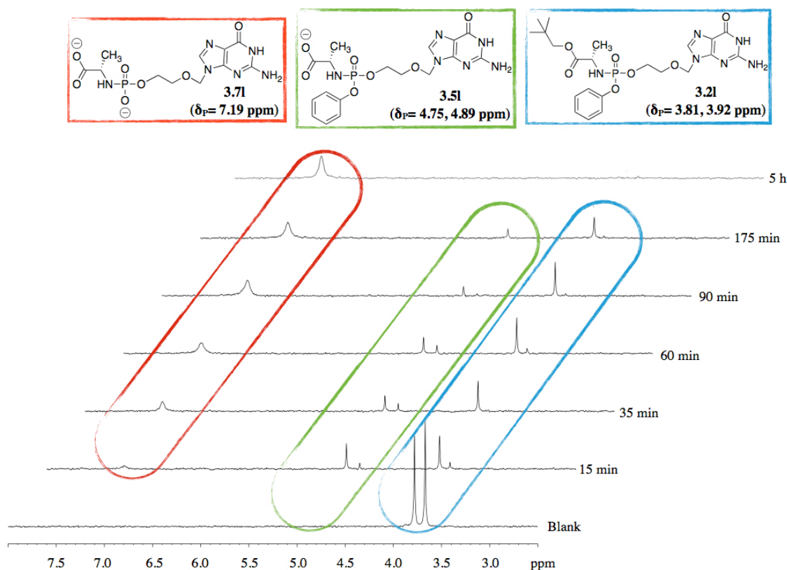
Figure 3.8. ^{31}\text{P} NMR spectra (acetone- \text{D}_6 , 202 MHz) at different time of the enzymatic study performed on compound 3.21
