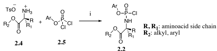
Scheme 2.2 General synthesis of aryl amino acid ester phosphorochloridates
