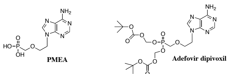
Figure 1.20. Structure of adefovir and its prodrug adefovir dipivoxil
