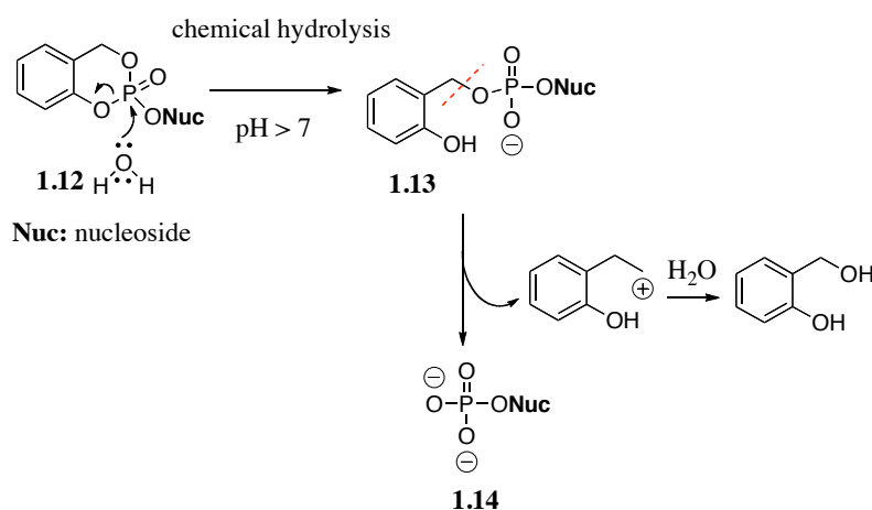
Scheme 1.3. Chemical hydrolysis of a generic Cyclosal pronucleotide
