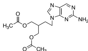
Figure 1.15. Structure of famciclovir
