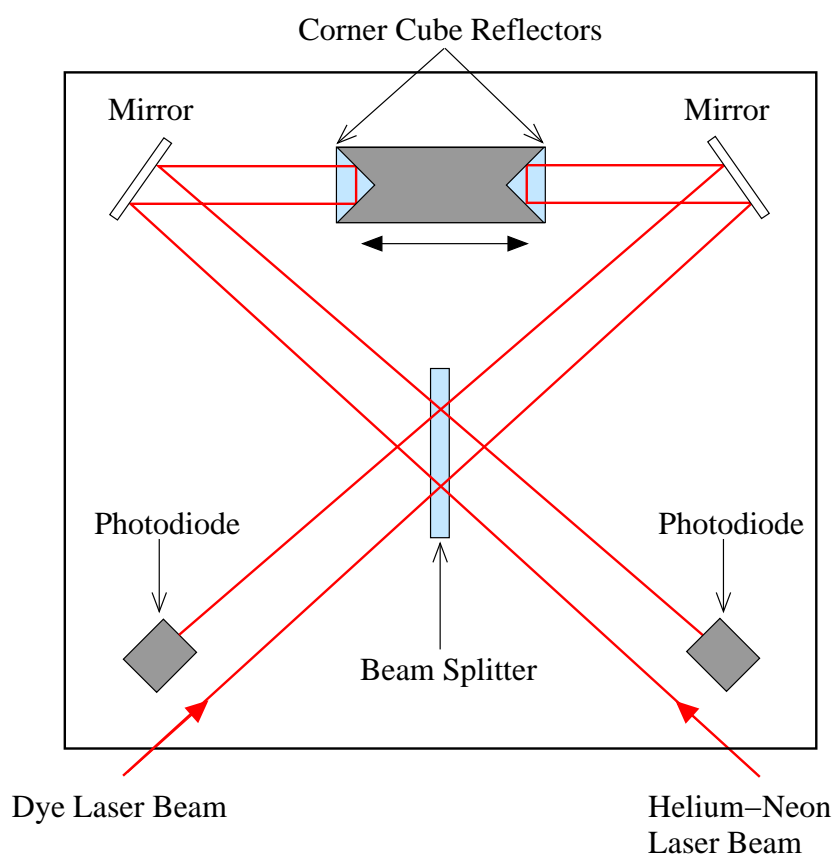
Figure 4.9: Schematic diagram of the wavemeter.
