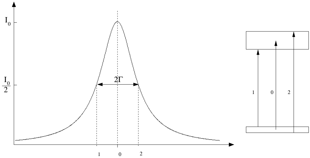
Figure 3.2: Natural Linewidth.
