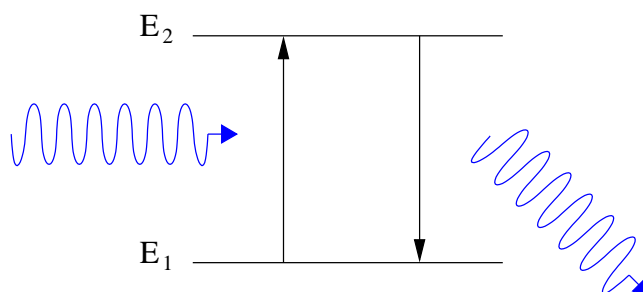
Figure 3.1: Laser Spectroscopy.
