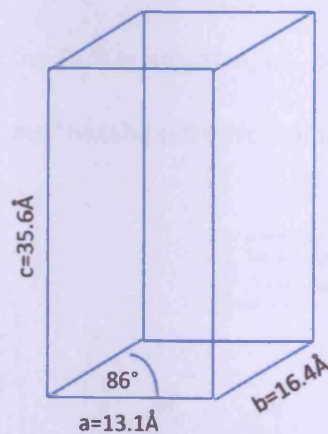
Figure 5.4. The unit dimensions when the inplane peaks at Q_{//}=1.262\text{\AA} and Q_{//}=1.510\text{\AA} are attributed to the (2,2, l ) and (3,1, l ) peaks
