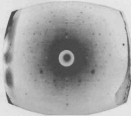
Figure 2.1. Diffraction pattern observed by Laue which resulted in him receiving the Nobel prize for Physics in 1914 taken from [2].
