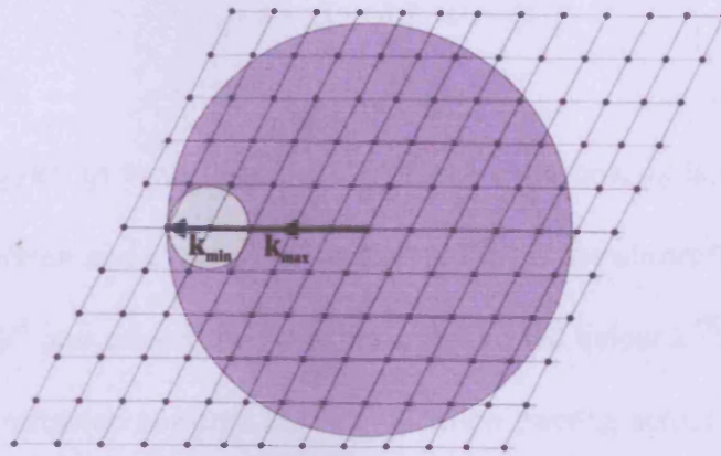
Figure 2.7. Construction of the Ewald Sphere [5]
