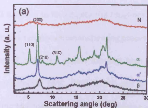
Figure 4.2. X-ray diffraction sections for each of the three distinct sub-phases taken from [15].
