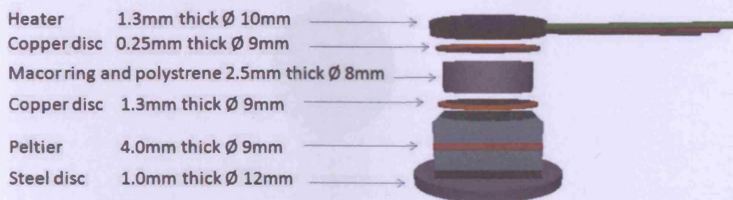
Figure 6.3 – The AFM heater
