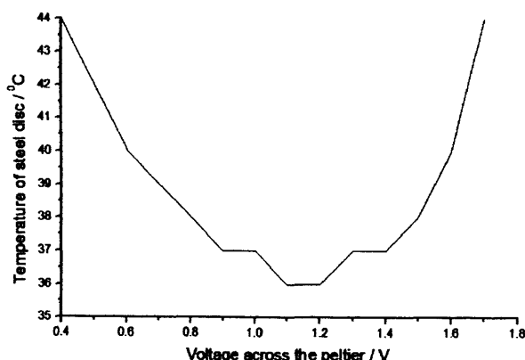
Figure 6.5 – Temperature response of the Peltier for varying voltages
