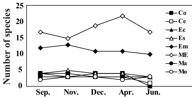
Fig. 4. Time evolution of the number of species per bioecological category for the five campaigns: Co: continental species, occasional in estuaries; Ce: estuarine species from continental origin; Ec: estuarine species from continental origin; Es: strictly estuarine species; Em: estuarine species from marine origin; ME: marine-estuarine species; Ma: marine species accessory in estuaries; Mo: marine species occasional in estuaries.
