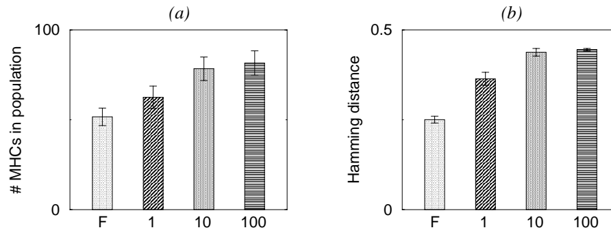
Figure 4. MHC molecules become functionally polymorphic. (a) The average number of different MHC molecules in the host population. (b) The average of the Hamming distances between all possible pairs of different MHC molecules in the host population. For parameters and axis labels see the legends of Figures 1 and 2.
