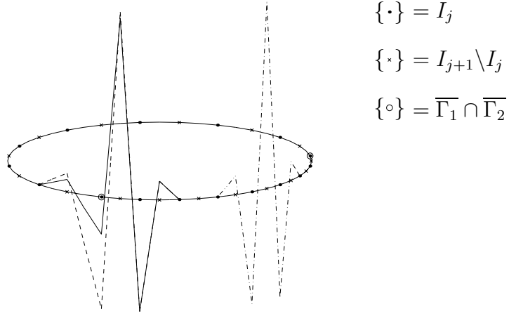
FIGURE 3. Wavelets \psi_{j,y} (‘—’) and \check{\psi}_{j,y} (‘---’) with supports that intersect an interface, and wavelets \psi_{j,y} = \check{\psi}_{j,y} (‘—’) with support inside one patch
