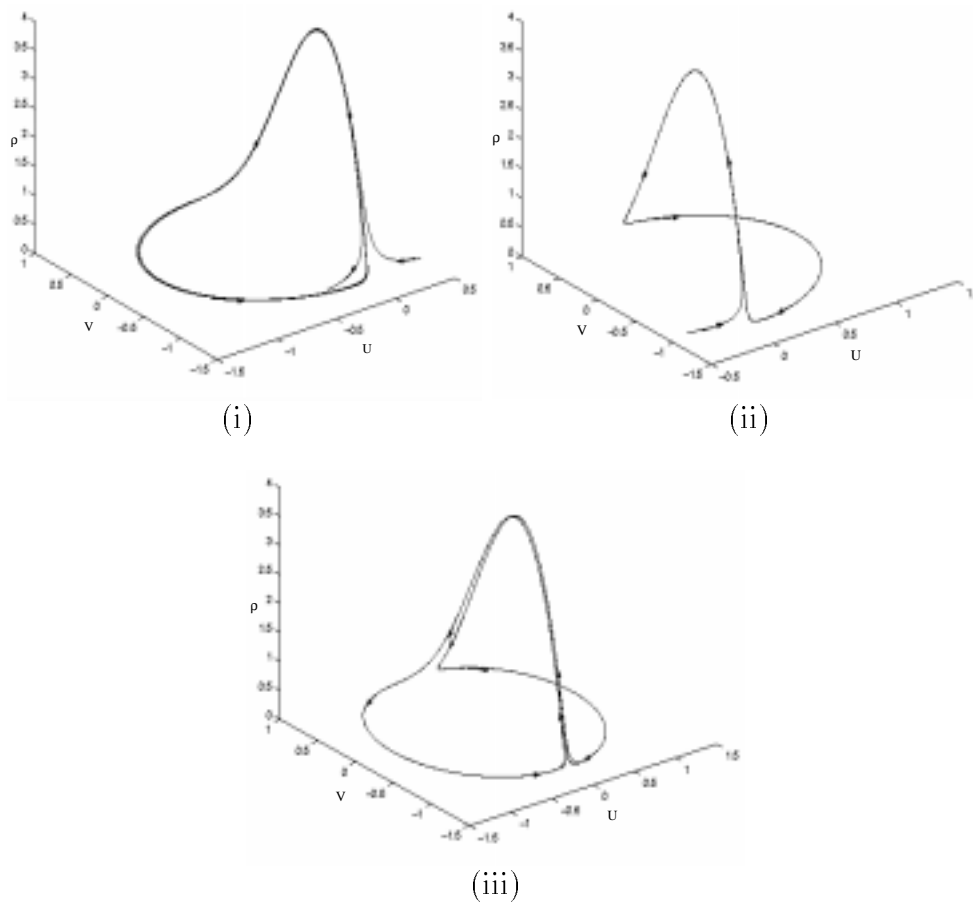
Figure 12: Forced symmetry breaking. (i) a long-periodic orbit for \sigma = 0.01 , (ii) a long-periodic orbit for \sigma = -0.01 , (iii) the combination of (i) and (ii).
