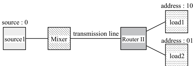
Fig. 10. Schematic diagram of the system to verify the reconstruction of power packets.
