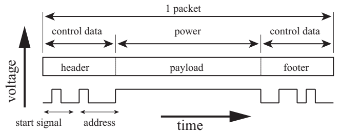
Fig. 1. Structure of power packet.
