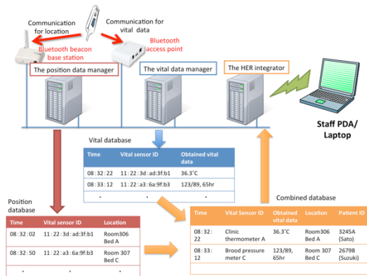
Figure 5. Server configurations
