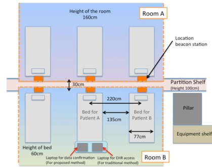
Figure 7. Setup for the evaluation
