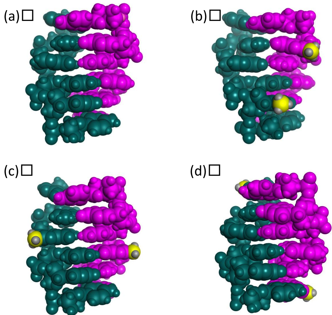
Figure 4. The optimized structures of modified d(CG) 3 strands. (a) d(CGCGCG) 2 ; (b) d(CGcm 8 GCG) 2 ; (c) d(Cm 8 GCGCG) 2 ; (d) d(CGCGcm 8 G) 2 .
