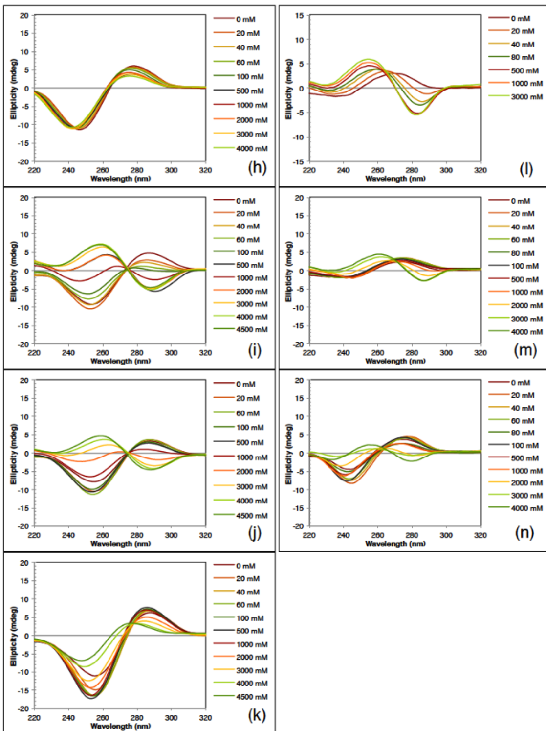
Figure 2. CD spectra of modified d(GC)_3 strands. (H) d(GCGCGC)_2 ; (I) d(GCm^8GCGC)_2 ; (J) d(GCGCm^8GC)_2 ; (K) d(m^8GCGCGC)_2 ; (L) d(GCm^8rGCGC)_2 ; (M) d(GCGCm^8rGC)_2 ; (N) d(m^8rGCGCGC)_2 ; Midpoint NaCl concentration was
