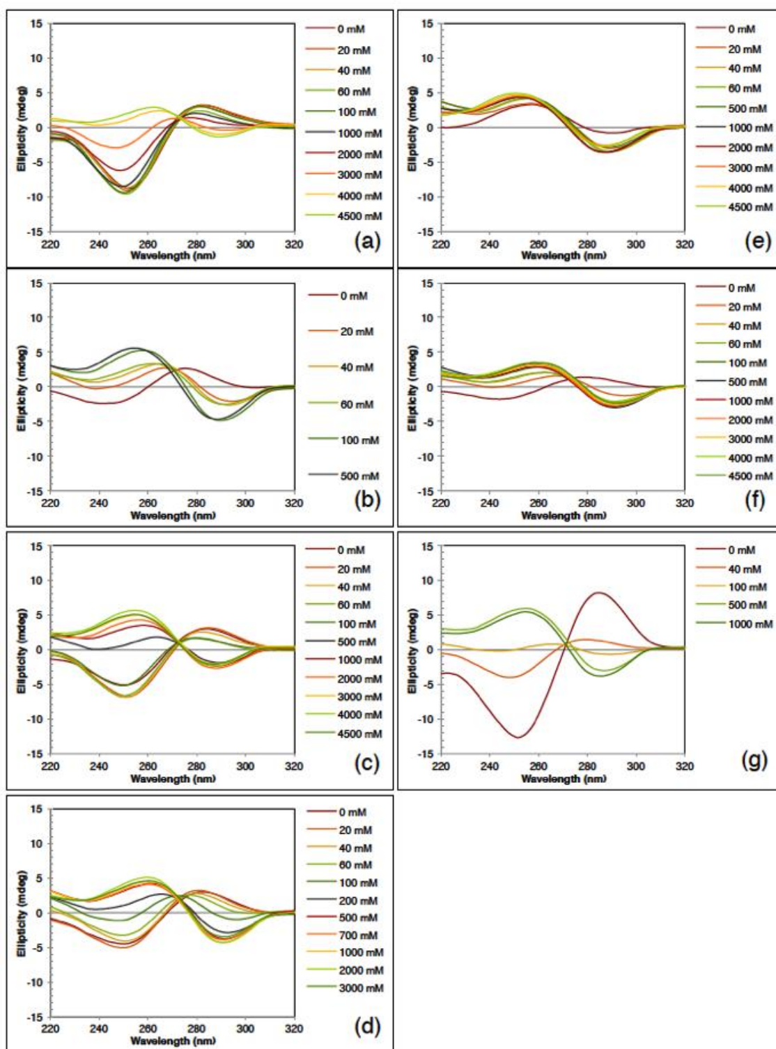
Figure 1. CD spectra of modified d(CG)_3 strands. (A) d(CGCGCG)_2 ; (B) d(CG\text{Cm}^8GCG)_2 ; (C) d(\text{Cm}^8GCGCG)_2 ; (D) d(CGCG\text{Cm}^8G)_2 ; (E) d(CG\text{Cm}^8rGCG)_2 ; (F) d(\text{Cm}^8rGCGCG)_2 ; (G) d(CGCG\text{Cm}^8rG)_2 ; Midpoint NaCl concentration was determined from the 290 nm of CD spectra at 4 °C, under various NaCl
