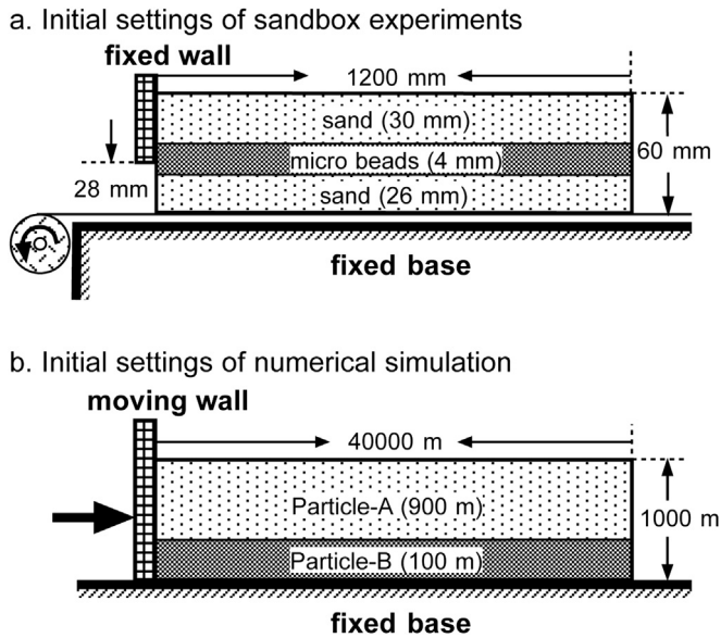
Figure 3. Initial setup of (a) analog experiments and (b) numerical simulation. To produce horizontal shortening, the materials were displaced relative to the fixed wall in the analog models, and a moving wall pushed the particles in the numerical models. The difference in the shortening kinematics has no significant impact on the results, according to Schreurs et al. (2006).
