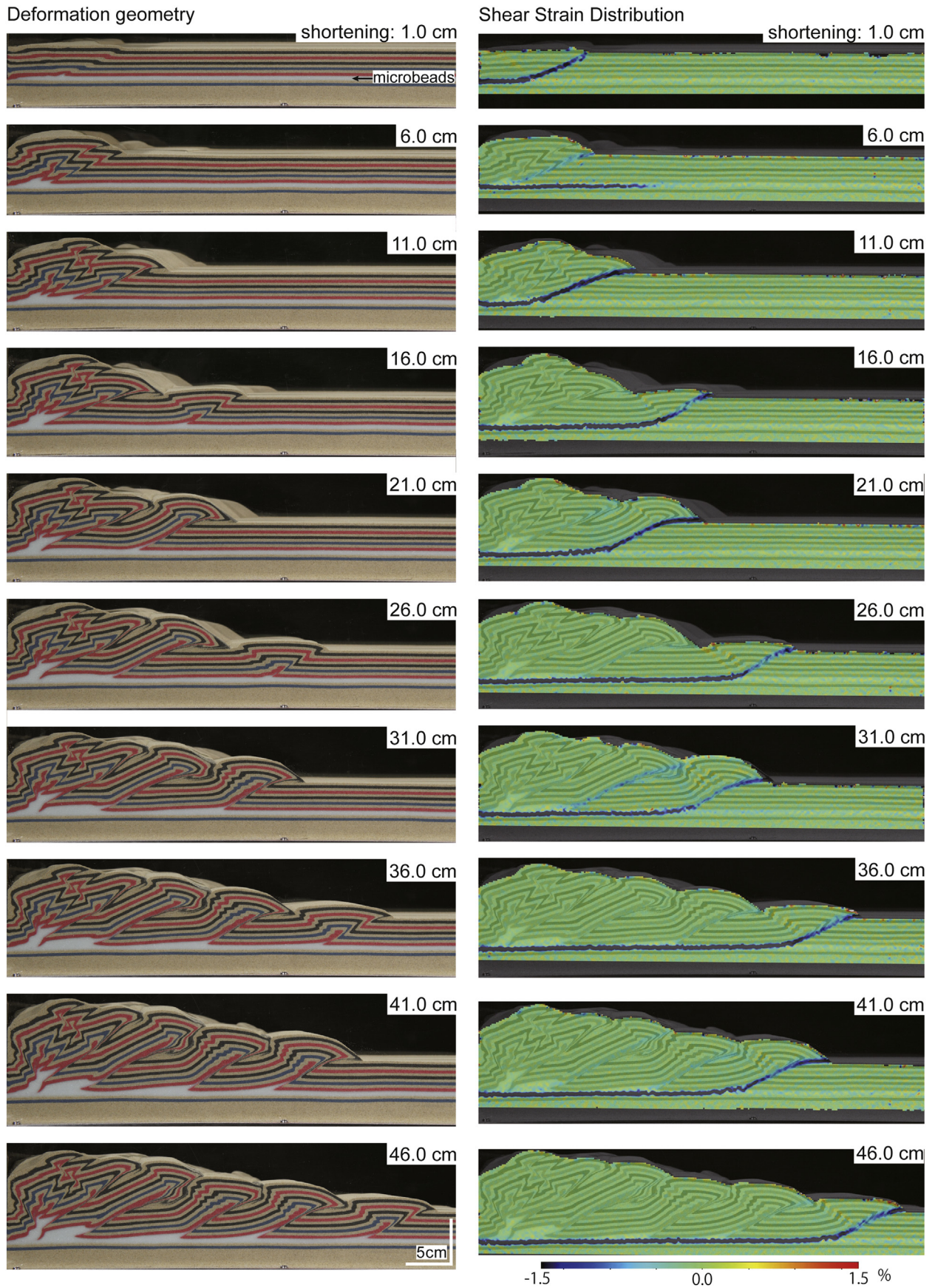
Figure 4. Results of the analog experiment, showing deformation geometry at every 5.0 cm step of horizontal shortening and shear strain distributions calculated with the digital image correlation (DIC) technique. The experiment produced a typical geometry of sequential thrusts accompanied by minor backthrusts, and an accretionary wedge inclined gently toward the deformation front. Reactivation of some older foreland-vergent thrusts can also be identified from the elevated shear strain. Surface gliding can be identified by the thinning of the top sand layers.
