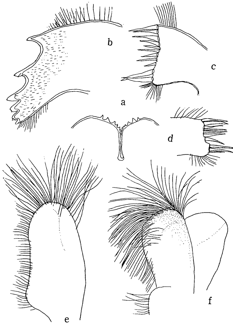
Fig. 7. Balanus improvisus DARWIN from Utiura Cove. a, Labrum; b, mandible; c, d, maxilla I; e, palp; f, maxilla II. (a, e, f \times 43 ; b-d \times 53 )
