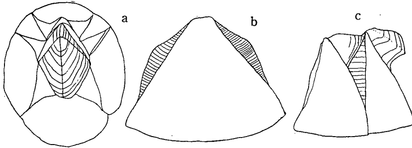
Fig. 8. Balanus eburneus GOULD from Utiura Cove, newly settled young. a, Newly settled young, 3 mm wide, top view; b, rostrum, outer view; c, carino-lateral and lateral compartments connected together. (b-c \times 9 )
