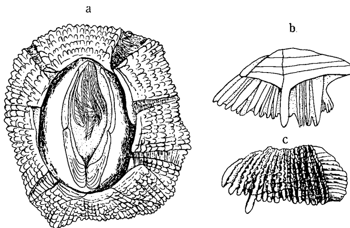
Fig. 10. Platylepas ophiophila LANCHESTER from Mano Bay, Sado Is. a , Animal, top view; b , lateral compartment, inner view; c , lateral compartment, outer view. ( a × 8.5; b , c × 16)
