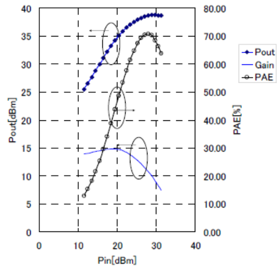
Fig.23 Measured output power, efficiency, and gain of the GaN amplifiers in Kyoto University's phased array
