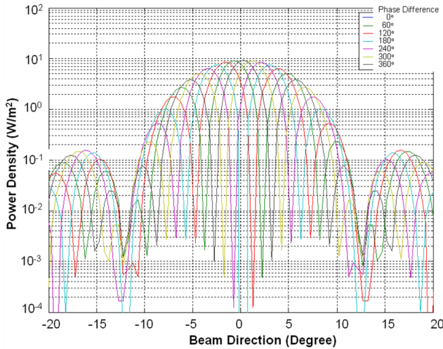
Fig.30 Theoretical beam pattern of the two radial slot antenna array
