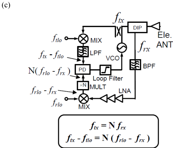
Fig.35 PLL-heterodyne retrodirective system developed by Mitsubishi Electric Corporation and the USEF SPS Study Team in FY2003 [27]. (a) Image of the system, (b) Block diagram of the conventional retrodirective system, and (c) Block diagram of the PLL-heterodyne retrodirective system
