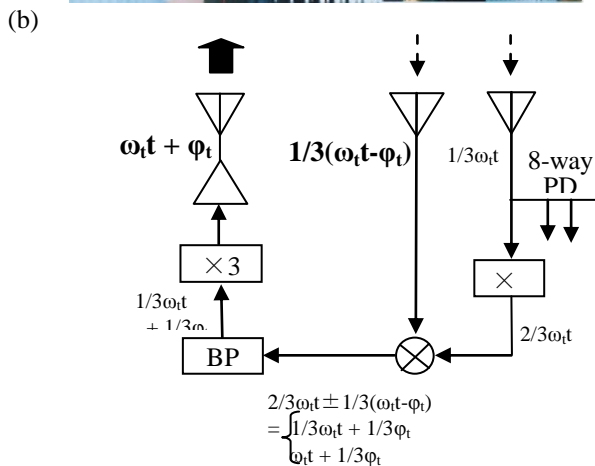
Fig.33 Retrodirective system using the 1/3 frequency pilot signal developed by Kyoto University and Nissan Motor Company.
