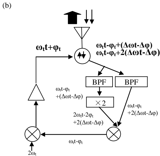
Fig.32 Retrodirective system composed of two asymmetric pilot signals developed by Kyoto University and Mitsubishi Electric Corporation.
