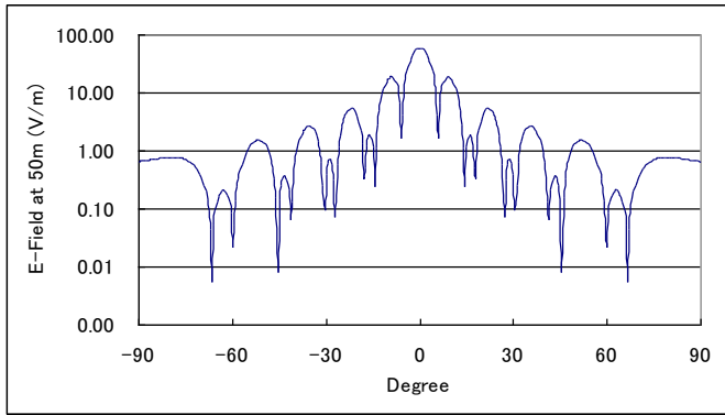
Fig.31 Measured beam pattern (E-field) of the two radial slot antenna array at a distance of 50 m for a radiated microwave power of 600 W
