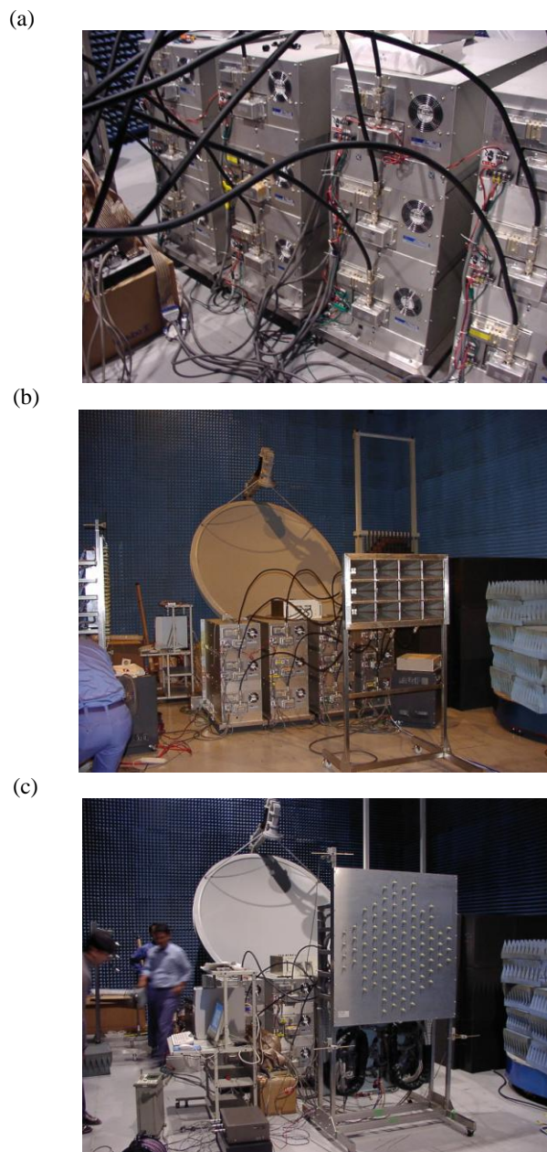
Fig.26 SPORTS-2.45 magnetron phased array.
