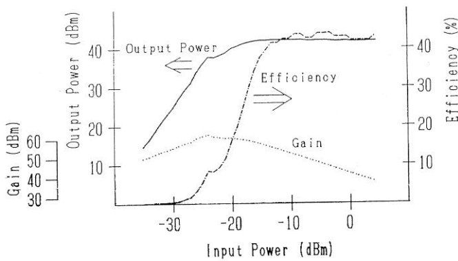
Fig.5 Measured output power, efficiency, and gain of the GaAs amplifiers used for the MILAX and ISY-METS
