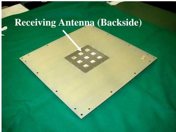
Fig. 17 AIA developed for MPT applications in FY2002
