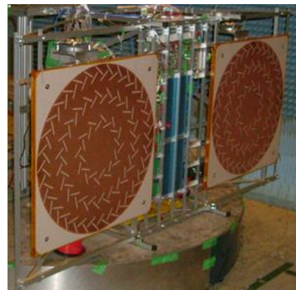
Fig.29 (a) Description of the airship to the ground MPT experiment conducted in 2009, and (b) Radial slot antenna array with two PCMs
