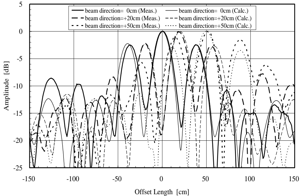
Fig.15 Theoretical and measured beam pattern of the parabolic antenna phased array at the Fresnel region
