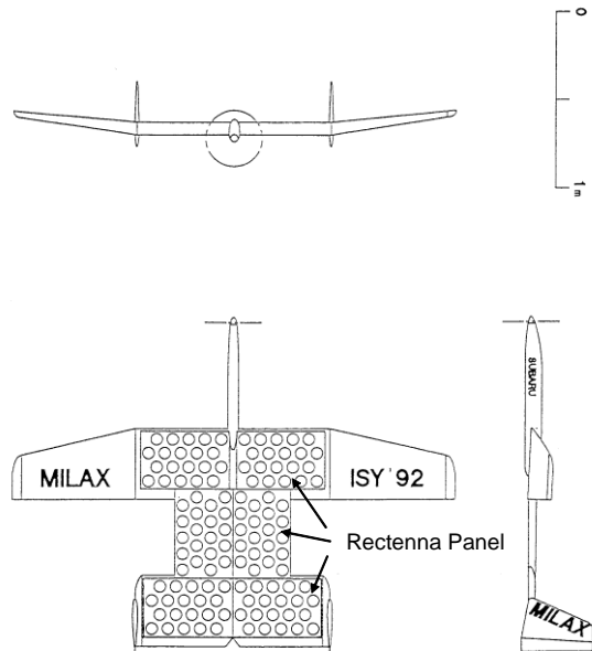
Fig.8 MILAX airplane and rectenna array
