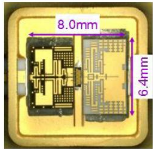
Fig.20 Metal packaged GaN HEMT amplifier [18]
