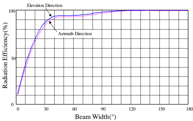
Fig.18 AIA radiation efficiency vs beam width
