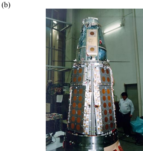
Fig.9 Phased array used in the ISY-METS rocket experiment. (a) Its expanded shape for the experiments, and (b) Its folded shape for launch
