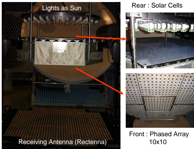
Fig.12 The SPRITZ project conducted in FY2000, demonstrating the phased array developed for the SPS application
