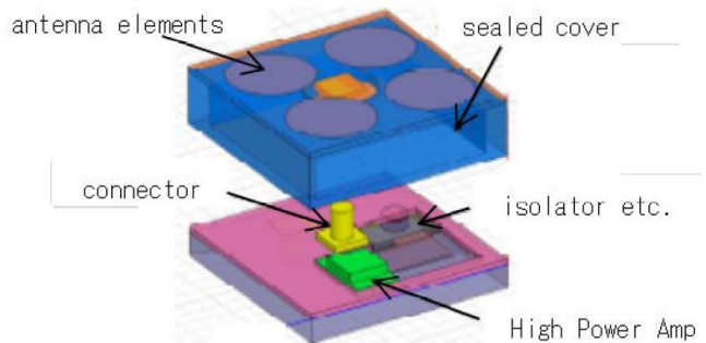
Fig.21 Structure image of the sub-array [18]
