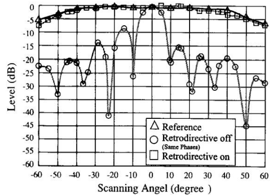
Fig.34 Measured beam pattern owing to retrodirective on and off states
