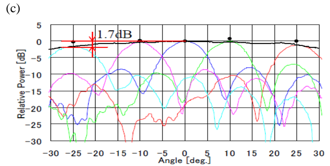
Fig.36 Beam pattern of the PLL-heterodyne retrodirective system [27]. (a) Beam target of 0 degree, (b) Beam target of 25 degrees, and (c) Beam pattern with and without the retrodirective system engaged
