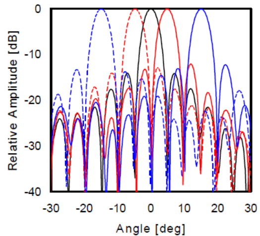
Fig.25 Measured elevation beam pattern of the phased array (beam steering angle: EL = -15, -5, 0, 5, and 15 degrees (AZ = 0 degree))
