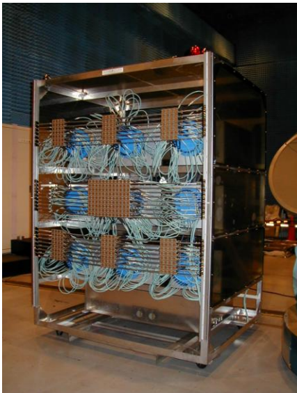
Fig. 28 SPORTS-5.8 magnetron phased array
