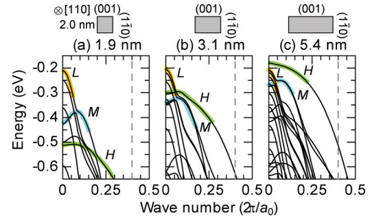
FIG. 7. (Color online) Valence band structure of 2.0-nm-height rectangular cross-sectional [110]/(001) nanowires with widths of (a) 1.9 nm (square case), (b) 3.1 nm, and (c) 5.4 nm. The energy is referenced from the band edge of bulk. Rectangles above each plot indicate the cross-sectional shape of calculated nanowires. Band structure contains three different types of subbands: small effective mass subband ( L band), half-M-shaped subband ( M band), and large effective mass subband ( H band). The dash line indicates the position of k = 0.4 \times 2\pi/a_0 .
