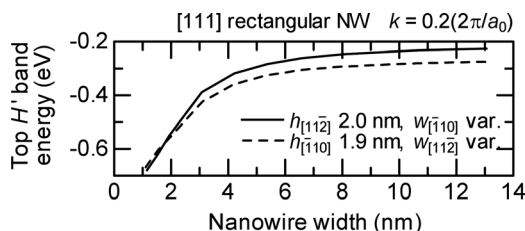
FIG. 12. The energy level of the highest heavy ( H' ) band in [111] rectangular cross-sectional silicon nanowires at k = 0.2 \times 2\pi/a_0 . The energy is referenced from the band edge of bulk. Solid: [111]/(112) wires with constant |\bar{1}12\rangle height ( h_{|\bar{1}12\rangle} = 2.0 nm) and varying |\bar{1}10\rangle widths ( w_{|\bar{1}10\rangle} ); dashed: [111]/(110) wires with constant |\bar{1}10\rangle height ( h_{|\bar{1}10\rangle} = 1.9 nm) and varying |\bar{1}12\rangle widths ( w_{|\bar{1}12\rangle} ).
