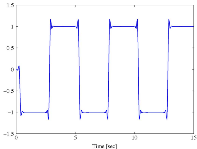
Fig. 8. Response of a sampled-data design filter against a rectangular wave.
