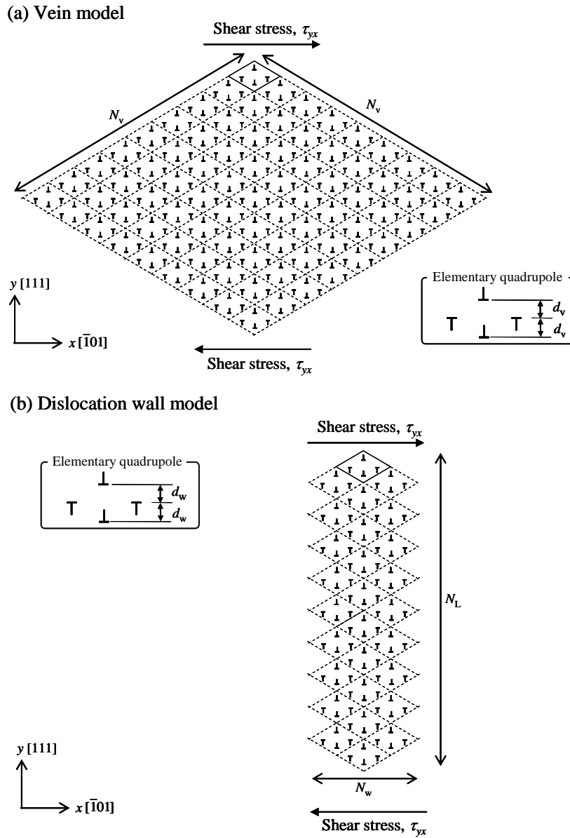
Fig. 2 Simulation models of (a) veins and (b) dislocation walls. \perp and \text{T} denote positive and negative edge dislocations, respectively.
