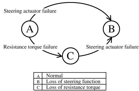
Figure 3: State transition of baseline SBW
