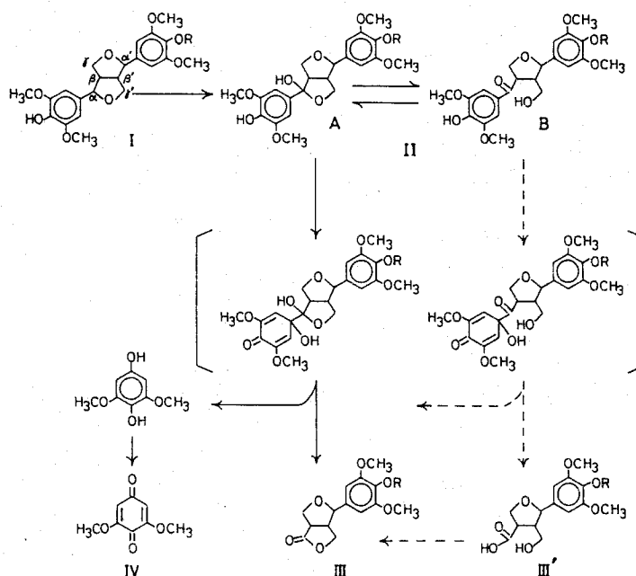
Fig. 5. Proposed degradation pathway for d,l -syringaresinol (I, R=H) and its monobenzyl ether (Ib, R=Bzl) by Fusarium solani M-13-1
