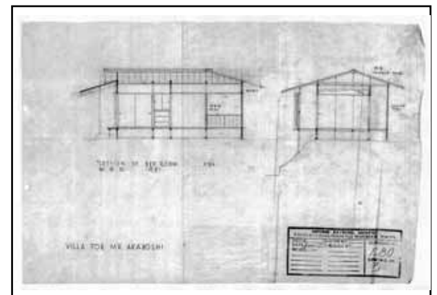
Section: bedroom
