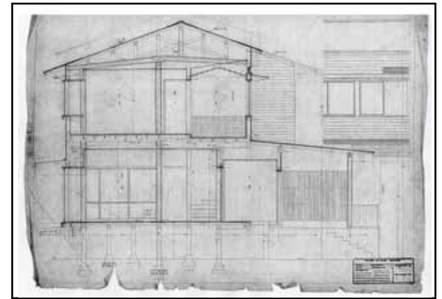
Cross section (1:20)
