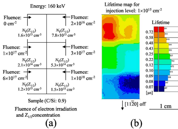
FIG. 3. (Color online) (a) Fluence of electron irradiation and distribution of Z_{1/2} concentration in a 50- \mu\text{m} -thick 4H-SiC epilayer selectively irradiated with a Cu mask. Electron irradiation was performed onto the sample grown at a C/Si ratio of 0.9 (donor concentration: 1.5 \times 10^{15} \text{ cm}^{-3} ). (b) Maps of carrier lifetimes in the electron-irradiated sample annealed at 950 °C for an illumination intensity of N_0 = 1 \times 10^{15} \text{ cm}^{-2} .
