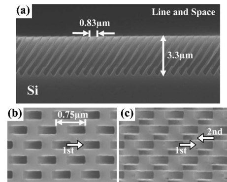
FIG. 4. Scanning electron microscope images of Si wafers with angled etching. A SF_6/O_2 ICP etching process at cryogenic temperatures is applied. (a) Cross sectional view of an angled-etched line-and-space pattern. A vertical depth of 3.3 \mu\text{m} is achieved. (b) Top view after first angled etching process for fabrication of a 3D PC. (c) Top view of a 3D PC after first and second angled etching processes. The thickness of the 3D PC is \sim 1 period.
