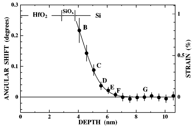
FIG. 4. Angular shift of the channeling dip as a function of depth from the surface. The axis on the right shows the local compressive strain estimated from the observed angular shift with Eq. (1).
