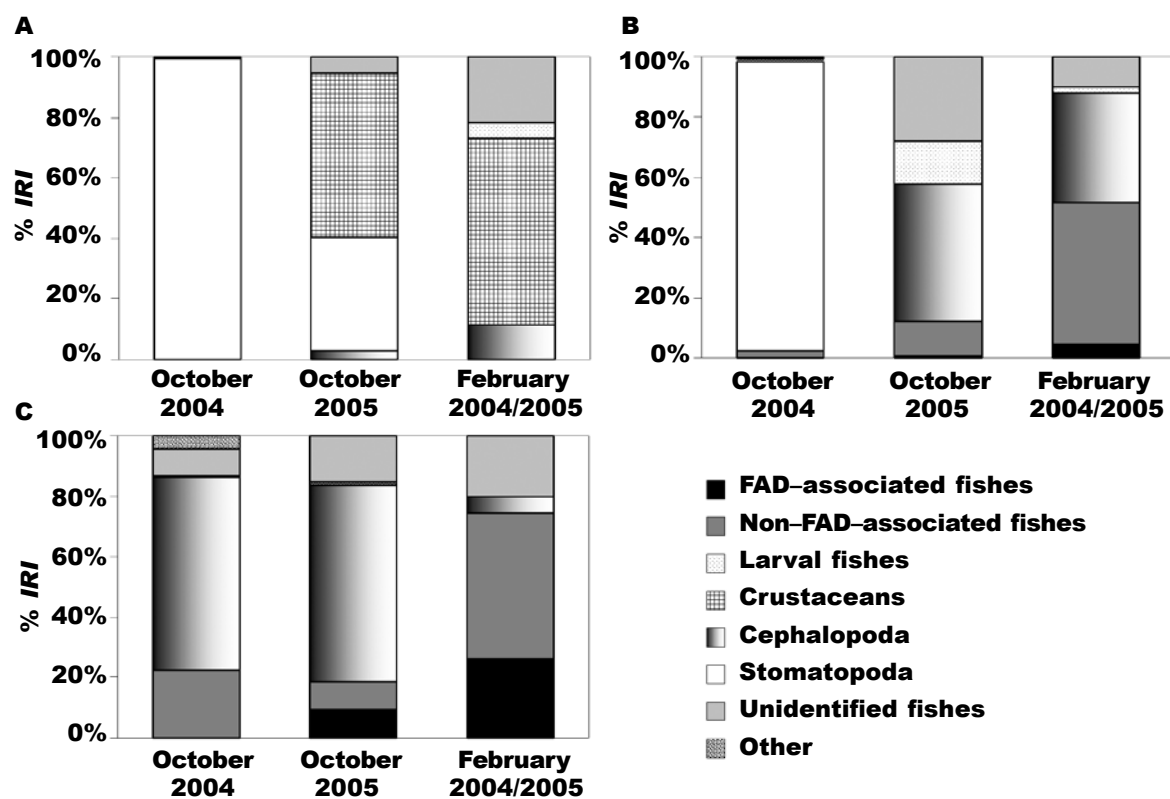
Fig. 2 Index of relative importance (% IRI) for the diets of: A. Yellowfin tuna ( Thunnus albacores ); B. Dolphinfish ( Coryphaena hippurus ); and C. Wahoo ( Acanthocybium solandri ) in October 2004, October 2005, and combined February 2004/2005.
