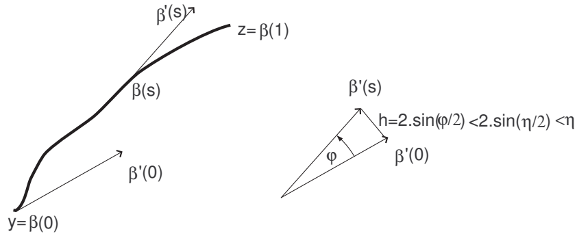
Figure 3 – Bounds for small angles
