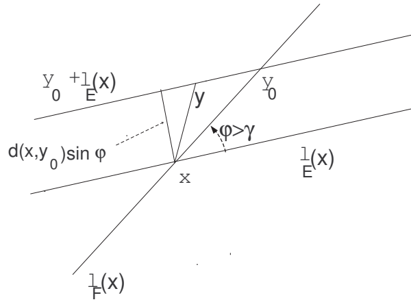
Figure 4 – Bounds for the distance between x and y \in y_0 + l_E(x)
