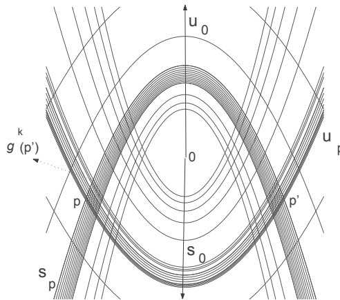
Figure 2 – Singularity of a generalized pseudo-Anosov
