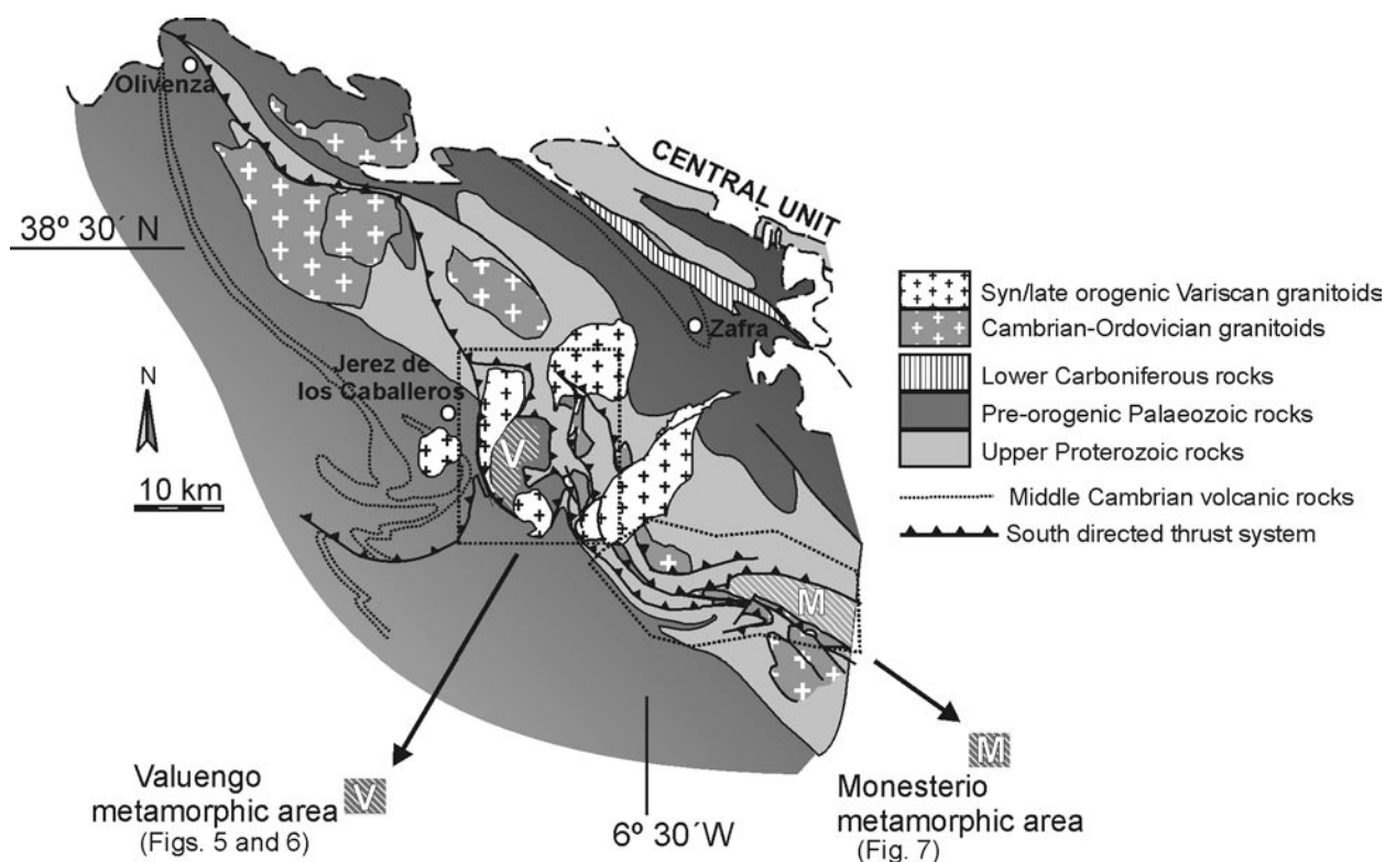
Fig. 4.- Geological and geographical location of the Valuengo and Monesterio metamorphic areas.
