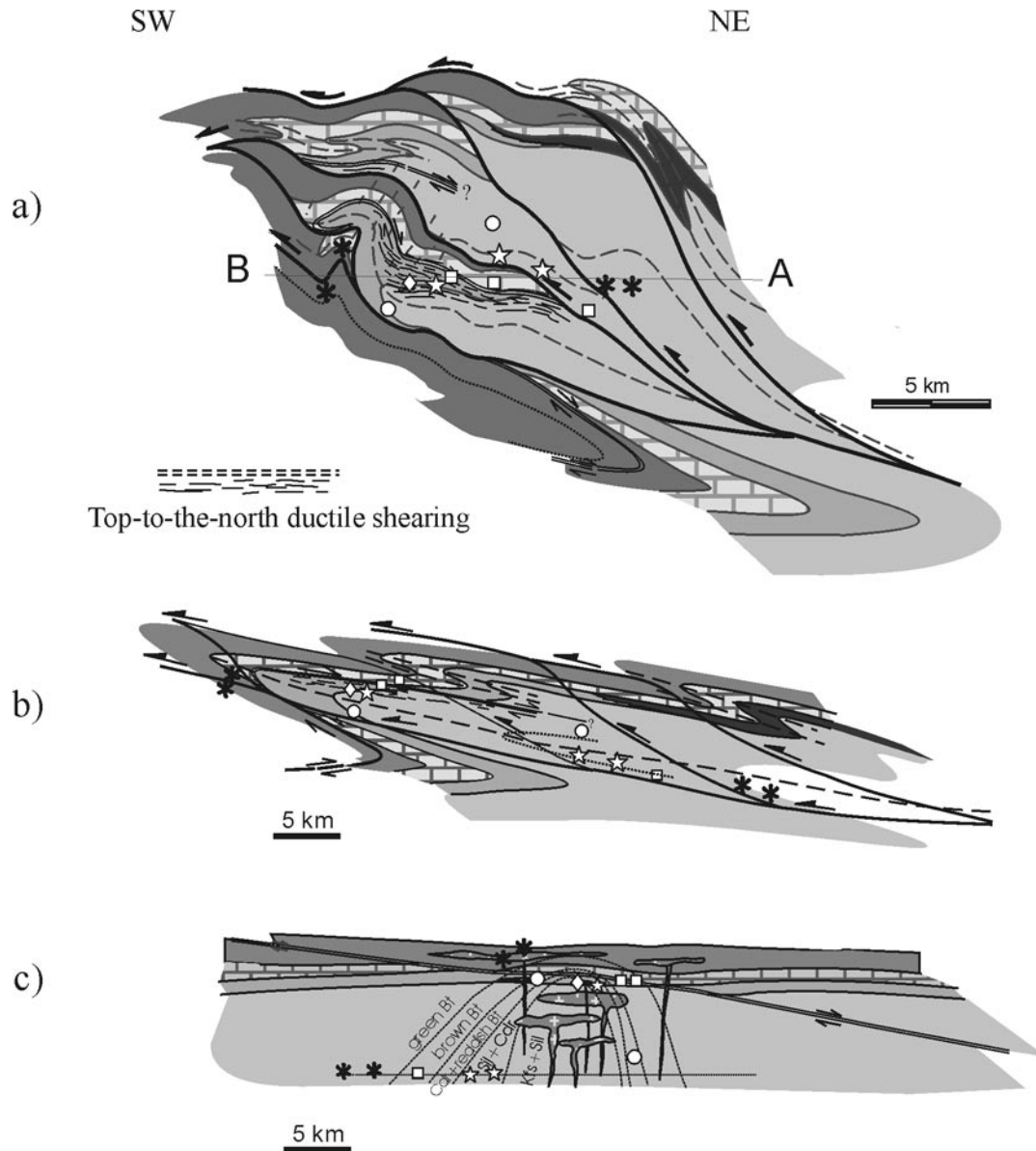
Fig. 6.- a) Geological cross-section of the Valuengo area. b) Partially restored cross-section, after removal of late folds and thrust displacements. c) Approximate complete restoration, showing the shape and distribution of metamorphic zoning. Subsurface plutons drawn in the metamorphic core are inferred to exist, but there is no direct evidence of them.
