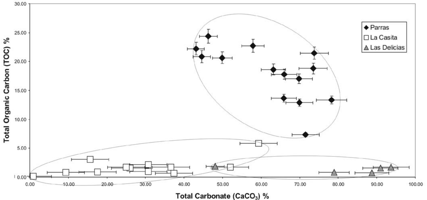
Fig. 9.- Total Organic Carbon (TOC) and Total Carbonate ( \text{CaCO}_3 ) contents. Samples from the three sections show distinct proportions indicating that environmental conditions greatly differed over the accumulation area. High TOC values correlate with low bioturbation as seen in Figure 5, while lower values are associated with distorted primary sedimentary structures and burrowing (Figs. 3 and 4).
