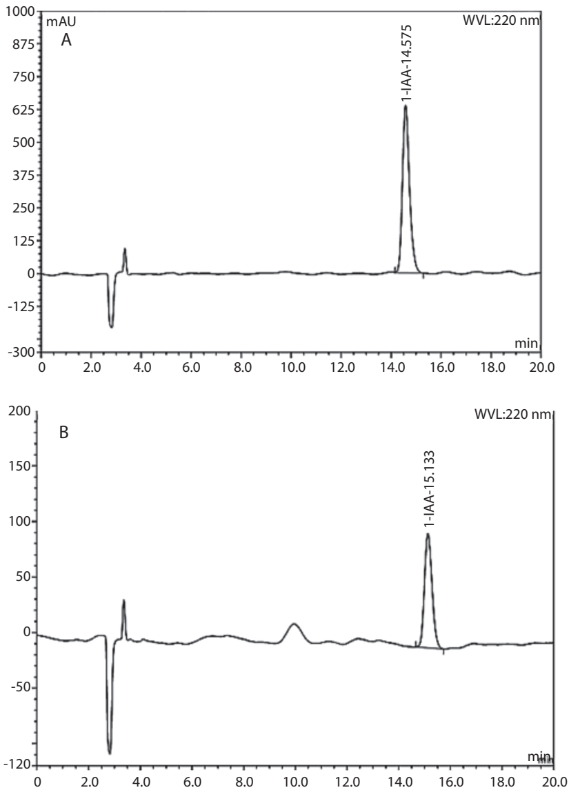
Fig. 4. HPLC analysis of (A) standard IAA; (B) extracted IAA from Leptolyngbya strain MMG-1.
