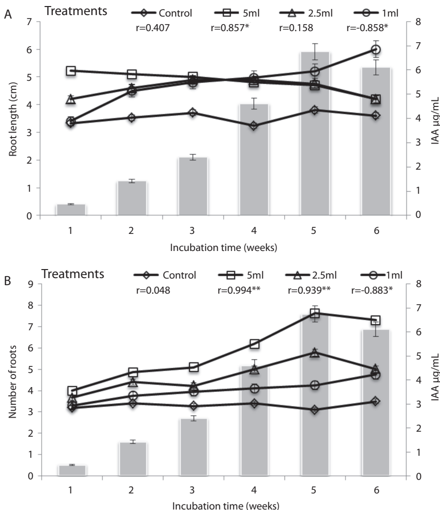
Fig. 5. Effect of supernatant (5, 2.5 and 1mL treatments) of Leptolyngbya strain MMG-1 on P. sativum seedling: (A) root length (B) number of lateral roots. Histogram represents IAA content of strains after a specific period of growth. Mean of three replicates, Correlation coefficient (r) between IAA and root length/number of lateral roots in different treatments (values beneath the legends). (.,=control treatment; o=5mL, r=2.5mL, i=1mL supernatant supplementations) (**. Correlation is significant at the 0.01 level, *. Correlation is significant at the 0.05 level).
