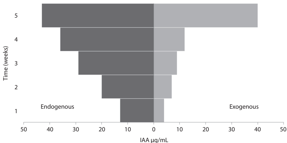
Fig. 3. IAA produced in media supplemented with varying amounts of the precursor L-tryptophan and after different time intervals. Mean of three independent experiments.
