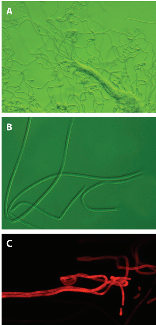
Fig. 1. Micrographs of Leptolyngbya strain MMG-1. (A) Trichomes growing on agar (Scale bar 50 \mu m) (B) Trichomes observed using differential interference contrast microscopy (Scale bar 10 \mu m) (C) Trichomes observed using confocal laser scanning microscopy (Scale bar 5 \mu m).
