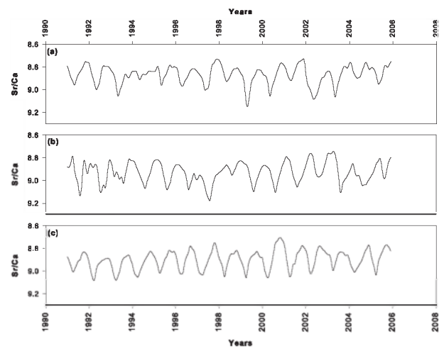
Fig. A1. The Sr/Ca time-series of coral cores MAS1 (a), ANDRA (b) and IFAHO (c) for the common period 1991–2005.
