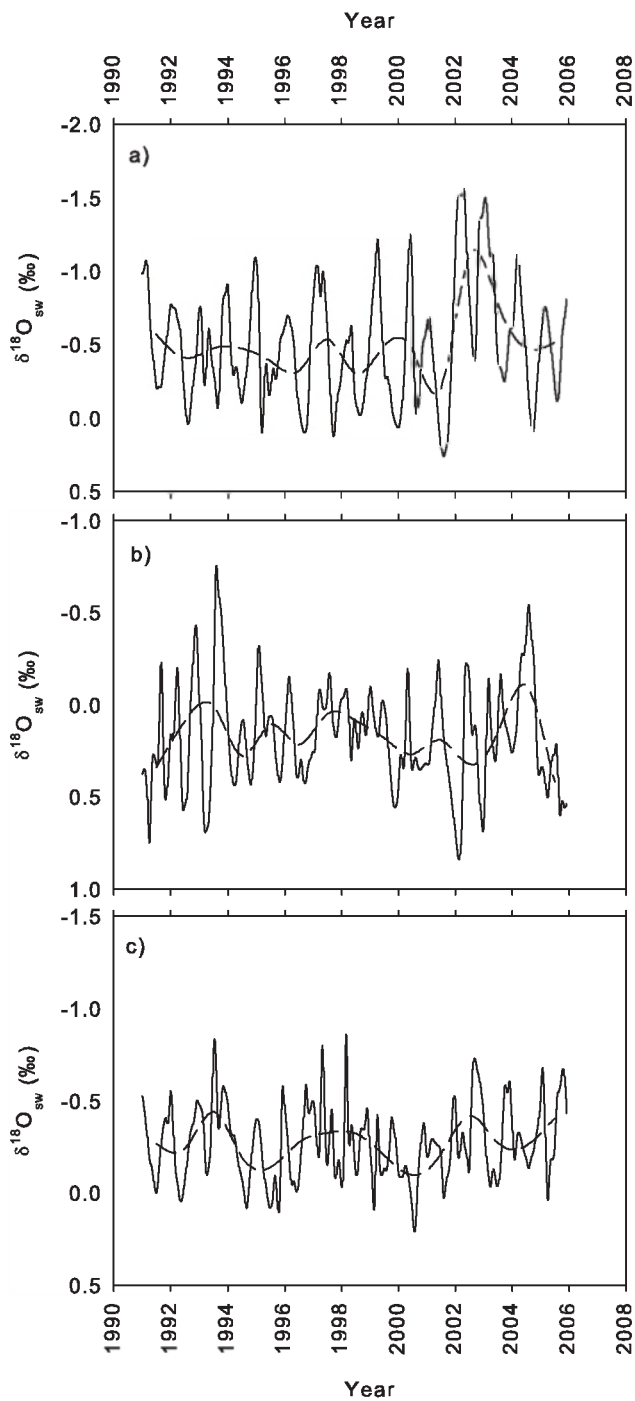
Fig. A3. The \delta^{18}\text{O}_{\text{seawater}} ( \delta^{18}\text{O}_{\text{sw}} ) of coral cores MAS1 (a), ANDRA (b) and IFAHO (c) calculated by subtracting the thermal component from coral skeletal \delta^{18}\text{O} based on the relative changes in Sr/Ca-SST following Ren et al. (2002). The annual average (dashed line) values were calculated by averaging the months January to December for each of the 15 yr.
