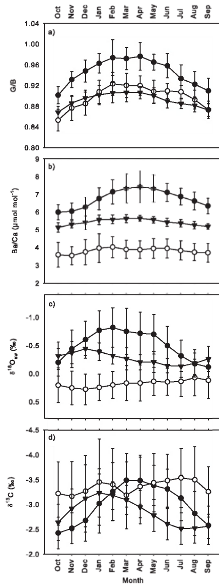
Fig. 6. Monthly averaged G/B (a), Ba/Ca (b), \delta^{18}\text{O}_{\text{sw}} (c) and \delta^{13}\text{C} (d) for MAS1 (solid circles), ANDRA (open circles) and IFAHO (triangles), indicating the average seasonal cycles. Monthly averages were calculated for the 15 yr period spanning January 1991 till December 2005. The standard deviations for individual months are given as error bars. The \delta^{18}\text{O}_{\text{sw}} and \delta^{13}\text{C} is given relative to V-PDB.
