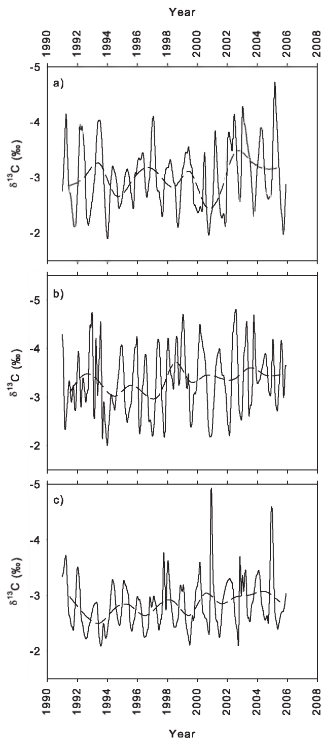
Fig. A4. The \delta^{13}\text{C} of coral cores MAS1 (a), ANDRA (b) and IFAHO (c) relative to V-PDB. The annual average (dashed line) values were calculated by averaging the months January to December for each of the 15 yr.
