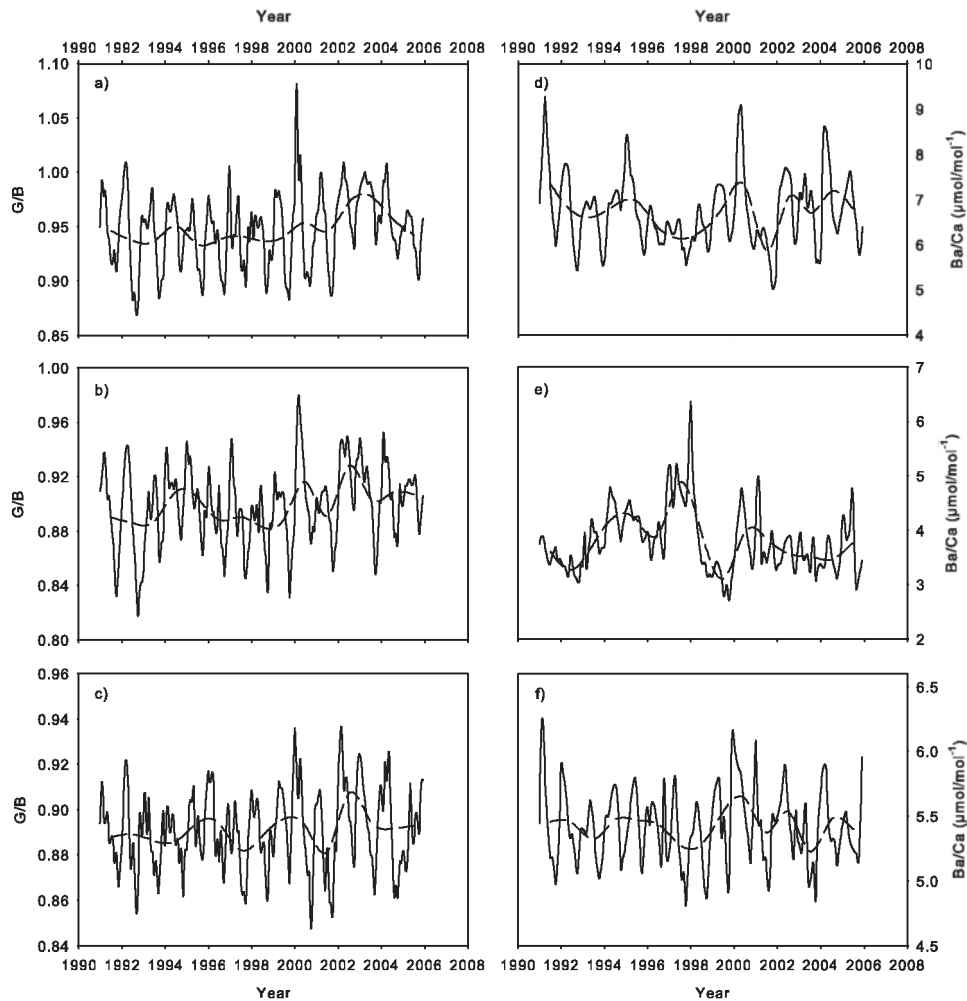
Fig. 4. Monthly G/B (a, b and c) and Ba/Ca (d, e and f) time-series over the 15 yr period between 1991 and 2005 for the three corals MAS1 (a and d), ANDRA (b and e) and IFAHO (c and f). The annual average (dashed line) G/B (a, b and c) and Ba/Ca (d, e and f) values were calculated by averaging the months January to December for each of the 15 yr.
