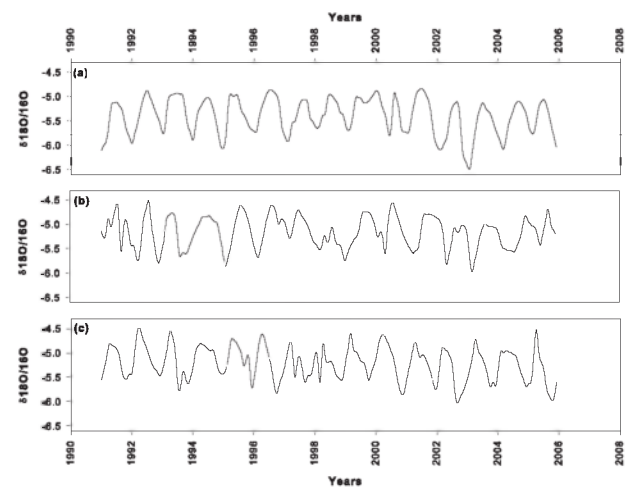
Fig. A2. The skeletal \delta^{18}\text{O} time-series of coral cores MAS1 (a), ANDRA (b) and IFAHO (c) for the common period 1991–2005.
