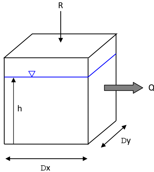
Figure 3 Basic structure of lumped catchment groundwater model
