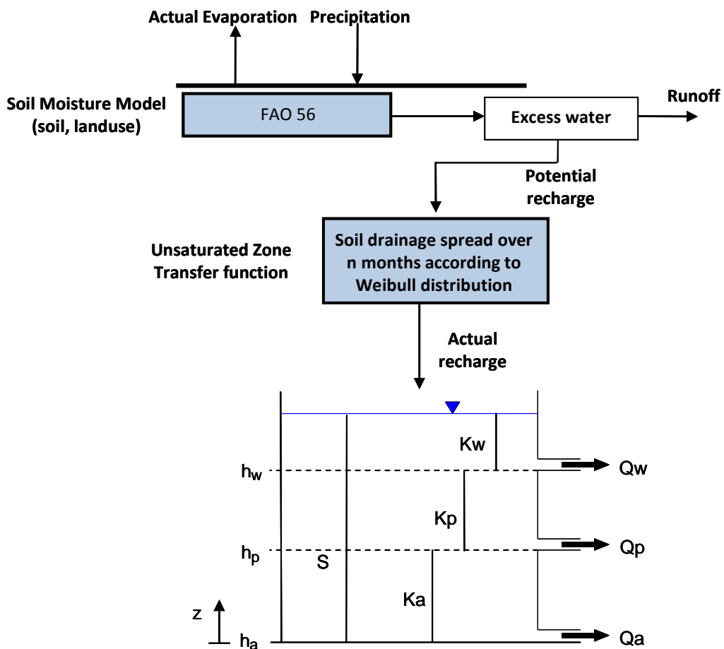
Figure 1 Structure of R-Groundwater
