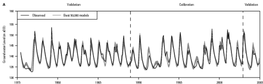
Figure 5 Observed and simulated hydrograph for the Baydon Hole borehole, Berkshire Downs.
