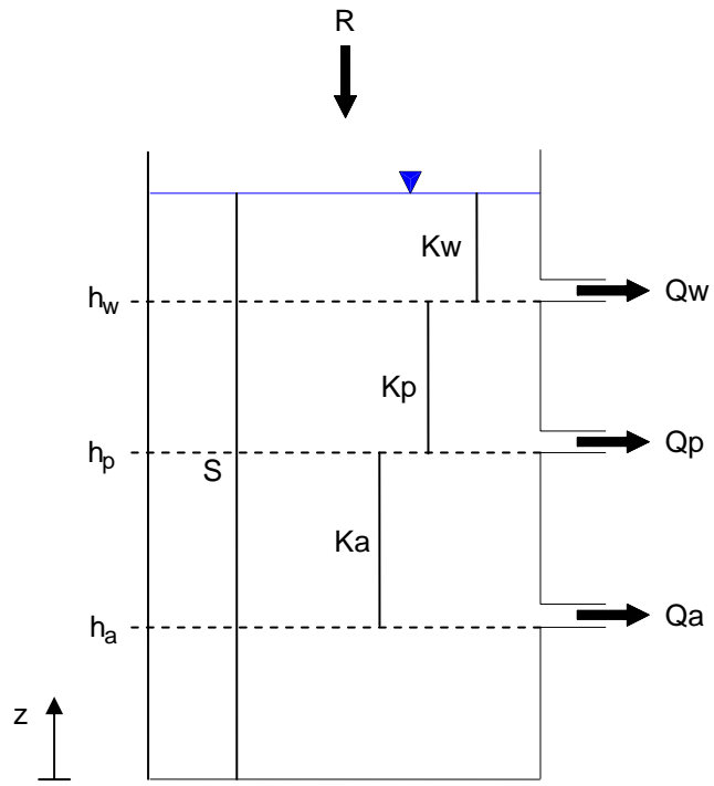
Figure 4 Example lumped groundwater model structure for application to a Chalk aquifer
