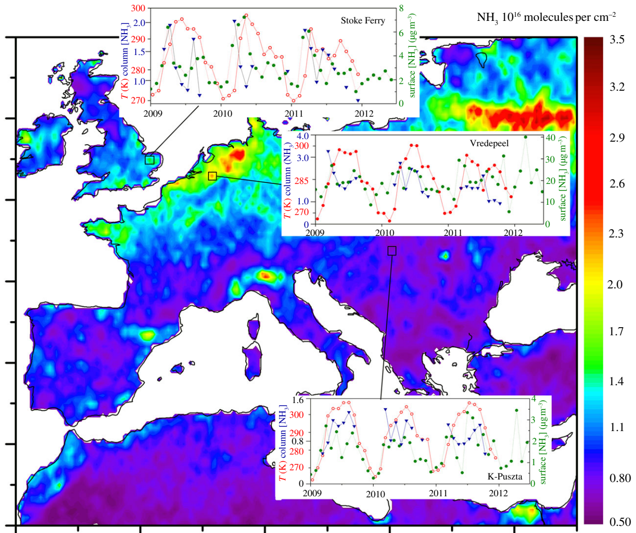
Figure 5. Satellite estimates of the \text{NH}_3 column ( 10^{16} molecules \text{cm}^{-2} ) and ground temperature, showing the mean for 2009, 2010 and 2011 (from the infrared atmospheric sounding interferometer on the MetOp platform), as compared with ground-based measurements of atmospheric \text{NH}_3 concentrations at three selected sites.
