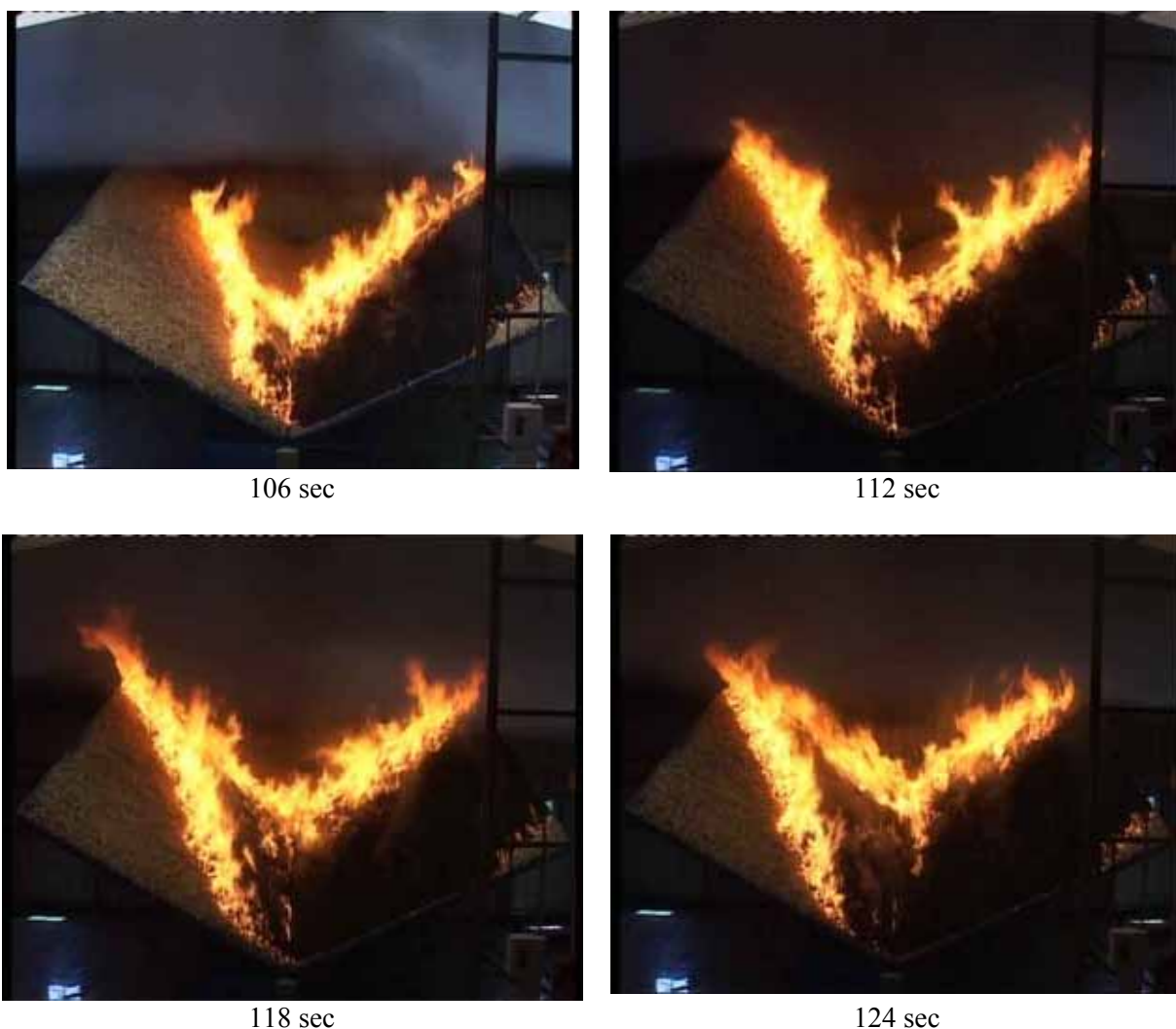
Figure 3.5. Sequence of images of fire spread during the following 24 seconds of the test performed at the DE4 of LEIF. The time step between frames is now 6 seconds.
