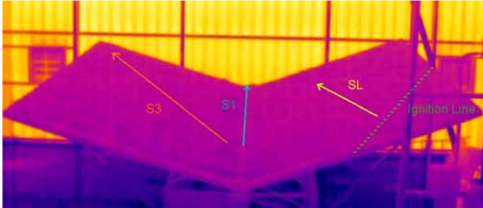
Figure 4.9. Schematic view of the Canyon Table of the Forest Fire Laboratory of the University of Coimbra indicating the position of the ignition line and the three directions S1, SL, and S3 along which the fire spread was analyzed.
