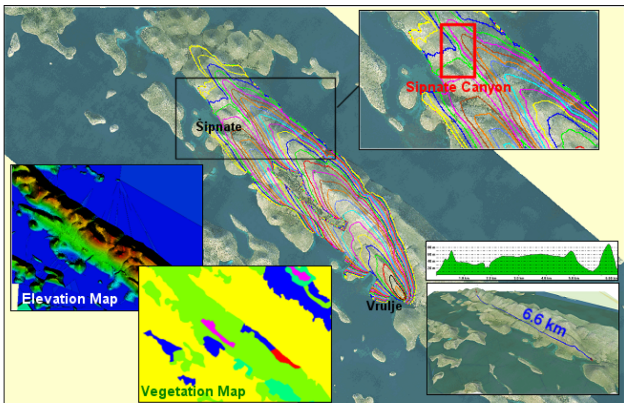
Figure 4.8. Fire spread simulation from the ignition point at Vrulje bay to the location of accident at Sipnate canyon based on Rothermel equations and adapted for Croatia at the University of Split. The dominant vegetation (light green) was modeled by Albini-Anderson category 1 (short grass), dead fuel humidity was 12\% and average mid-flame wind speed 2.29 \text{ m/s} .
