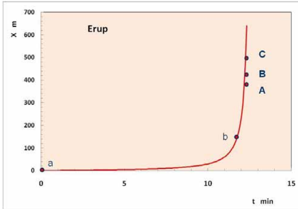
Figure 4.11. Predicted distance of advance of the fire along the water line of Sipnate canyon with time since its entrance at the base of the canyon at point a .
