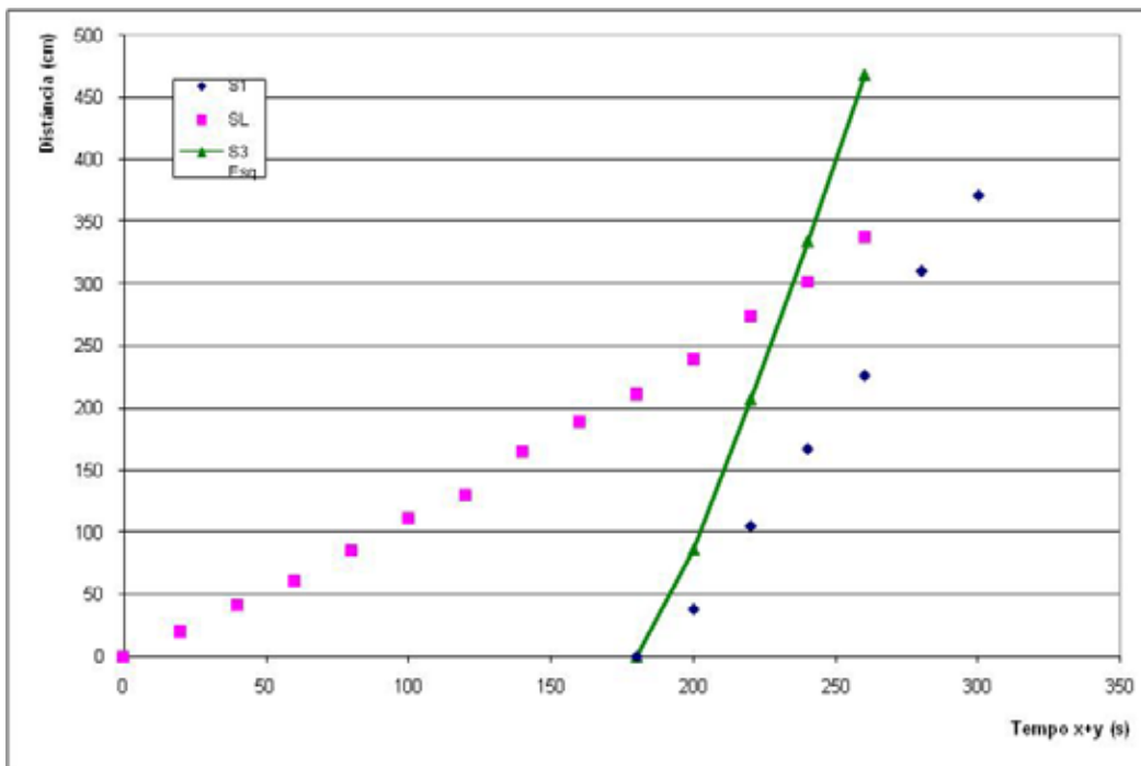
Figure 4.10. Distance traveled by the fire along the three main directions indicated in Figure 4.9.
