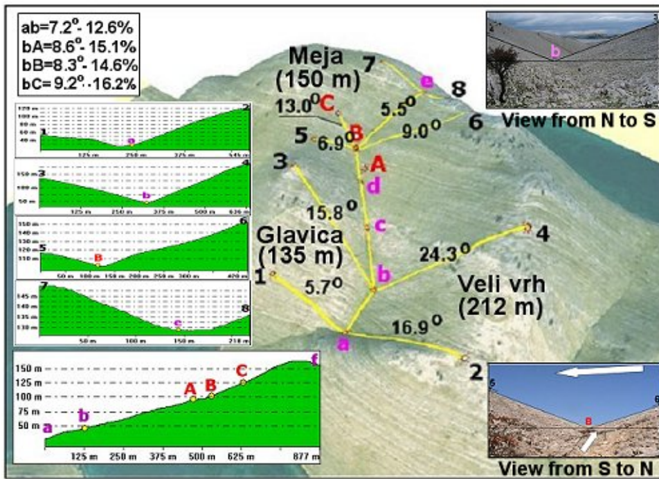
Figure 4.3. Sipnate canyon configuration with slope angles and canyon photos from north to south and vice versa
