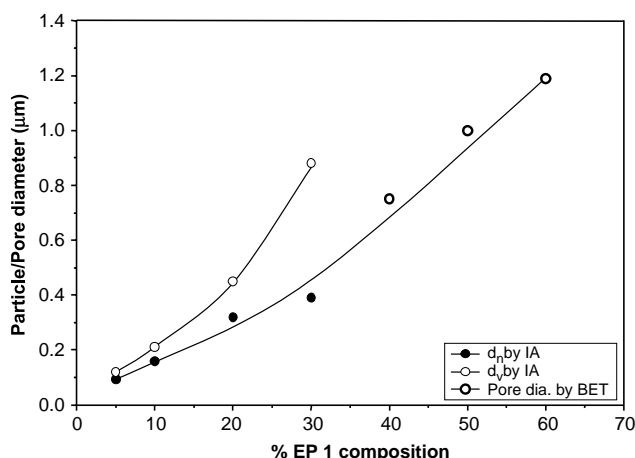
Fig. 7. Average particle/pore diameters as a function of composition for EP 1/PP 2 blends (IA stands for image analysis).
