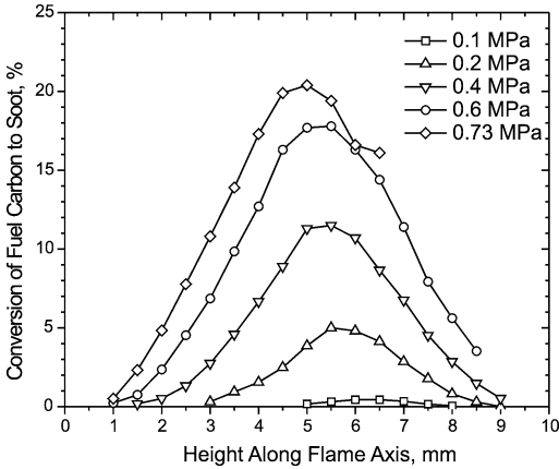
Fig. 13. Percentage conversion of carbon from fuel to soot as a function of axial location along the flame axis.
