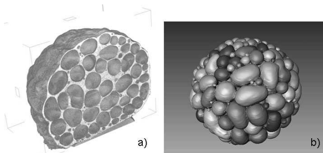
Fig. 2. Al-Cu-Mg alloy foamed without blowing agent by pressure manipulation, i.e. melting a powder compact under 6 bar pressure (Argon) and releasing pressure to 1 bar; a) visualisation of foam by X-ray tomography, b) computer-assisted segmentation of individual pores in the sample (Courtesy of F. García-Moreno, HMI Berlin).
