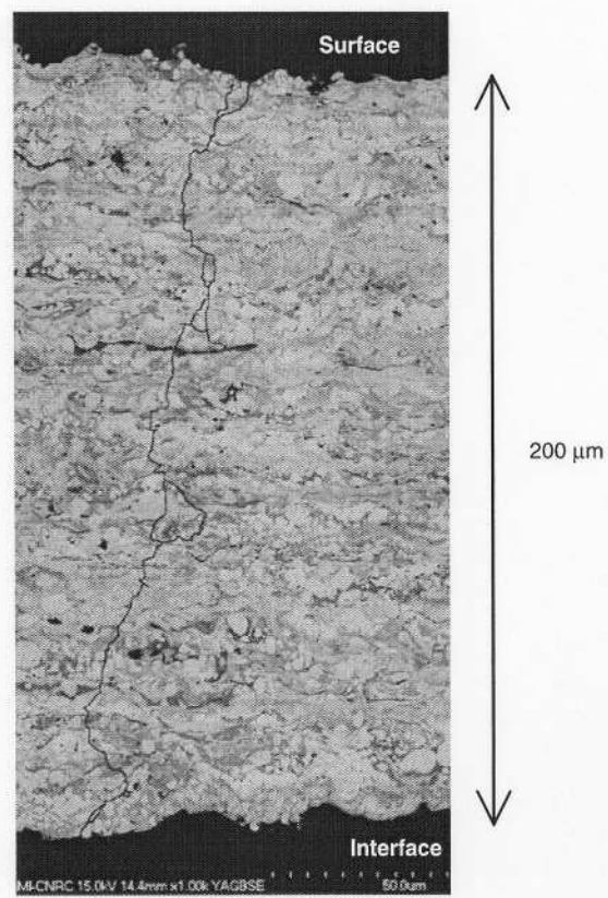
Figure 15. Microscopic image of a crack.
