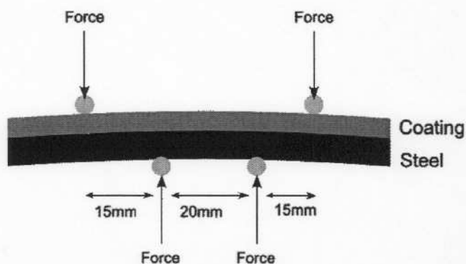
Figure 5. Four-point-bending specification.
