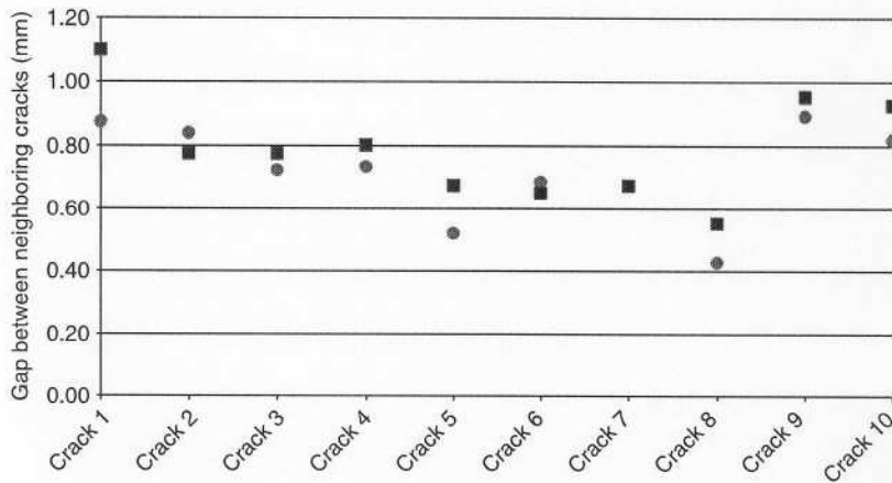
Figure 13. Crack spacing comparison of column A. ● Thermography ■ Microscope.
