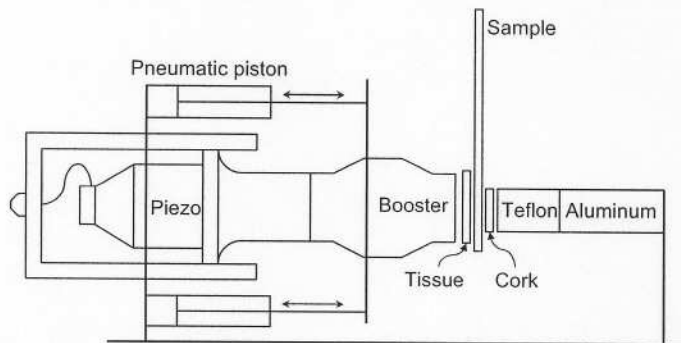
Figure 3. Experimentation approach.
