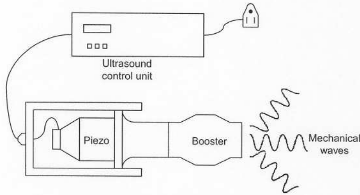
Figure 2. Ultrasound source.
