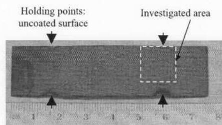
Figure 4. Tungsten carbide Almen strip.
