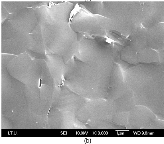
Fig. 1. SEM images of initial (a) and irradiated by 1.37 \times 10^{21} \text{ n.m}^{-2} neutron fluence (b) of \text{B}_4\text{C} .
