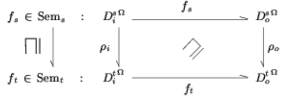
Fig 4: Commutative diagram expressing correct implementation
