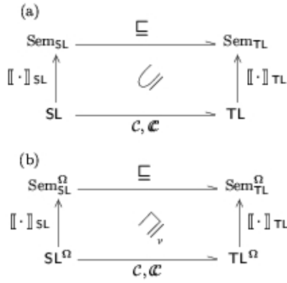
Fig 12. Correctness of extended compiling specifications. The original diagrams (a) (for \mathcal{C} and \mathcal{C} ) are commutative if and only if the corresponding extended diagrams (b) are.
