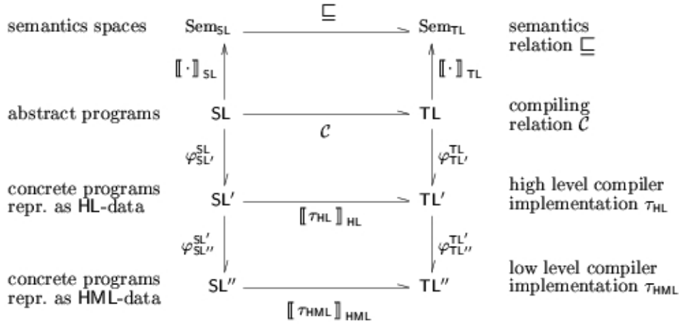
Fig 2. Three steps for correct compiler implementation \tau_{HML}
