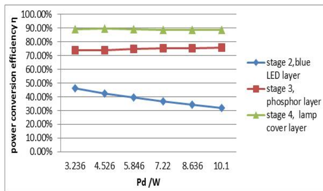
Figure 6. Conversion efficiency of the LED bulb for Stage 2 to Stage 4 at 3 W to 10 W.
